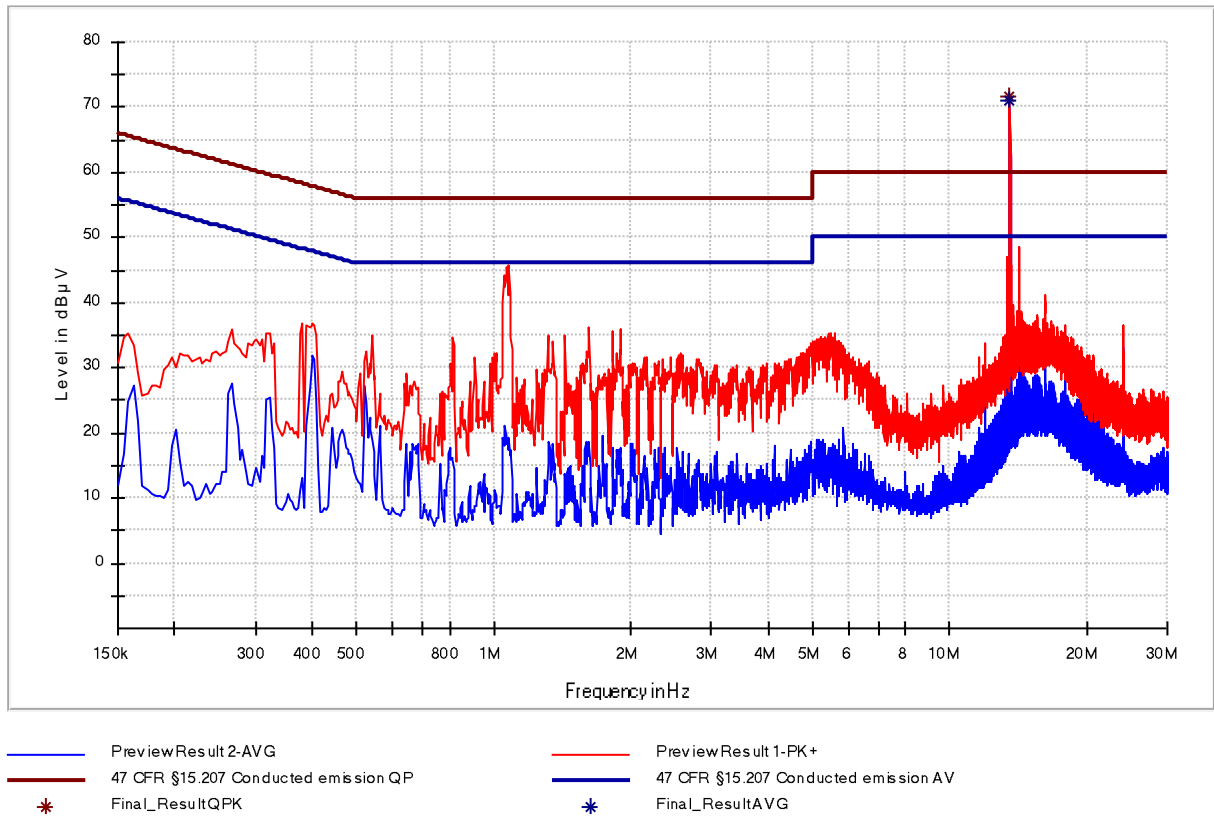
Figure 5: Chart of AC power-line conducted emissions test – phase L1, without termination
