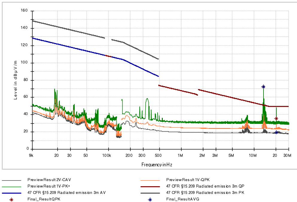
Figure 12: Chart of emissions test below 30 MHz without tag in position 1, antenna in line @ 3 m
