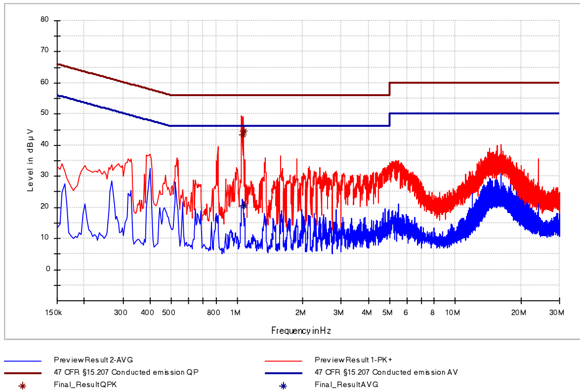
Figure 7: Chart of AC power-line conducted emissions test – phase L1, with termination
