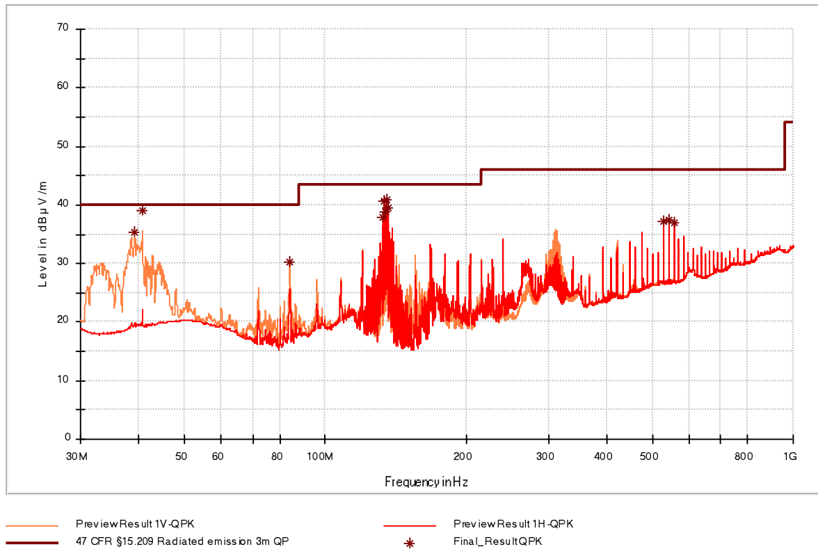
Figure 13: Chart of emissions test from 30 MHz to 1 GHz with tag in position 2 with tag @ 3 m
