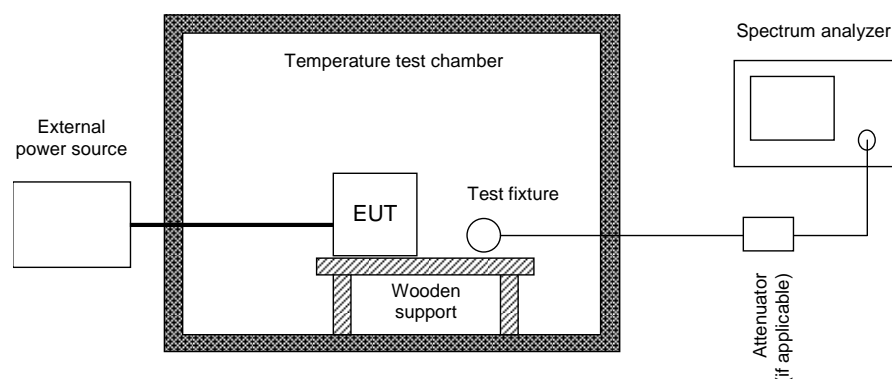
Figure 4: Test setup for carrier frequency stability measurement
