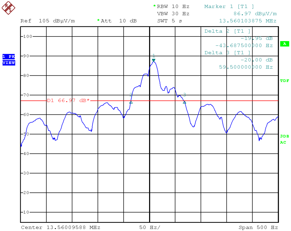
Figure 9: Chart of 20 dB bandwidth
