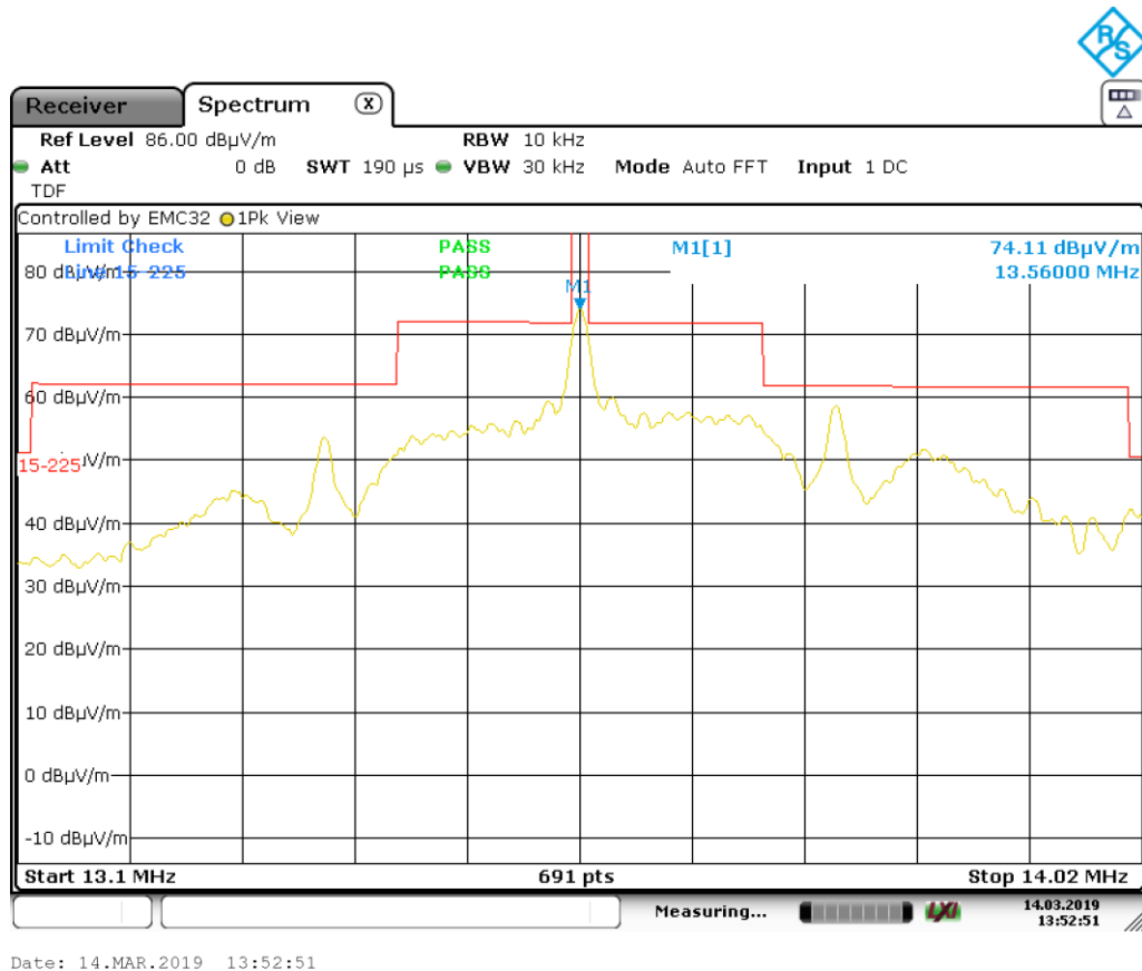
Figure 11: Spektrum mask of 13.56 MHz @ 3m distance
