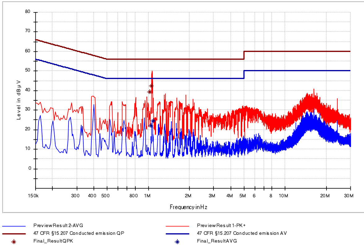
Figure 8: Chart of AC power-line conducted emissions test – phase N, with termination
