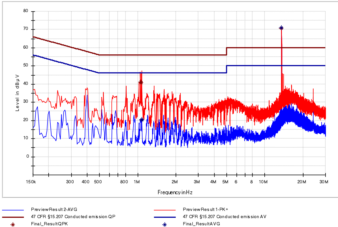
Figure 6: Chart of AC power-line conducted emissions test – phase N, without termination
