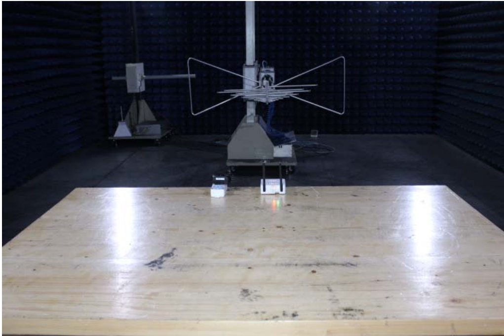
Photograph of set-up for Radiated Emission
