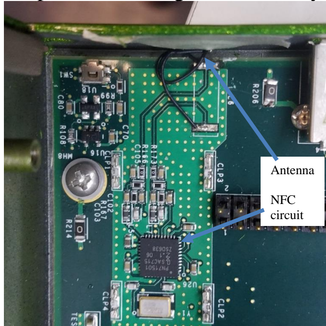
Top view showing NFC circuitry
