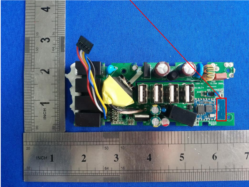
WIFI PCB antenna
