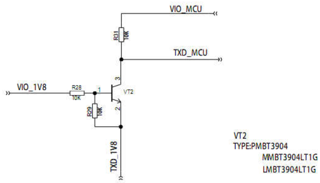
Figure 2-20 Recommended TXD circuit
