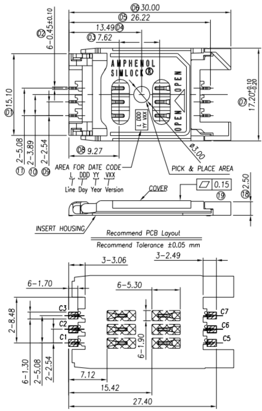
Figure 2-13 Amphenol C707 10M006 512 2 USIM Card Holder
