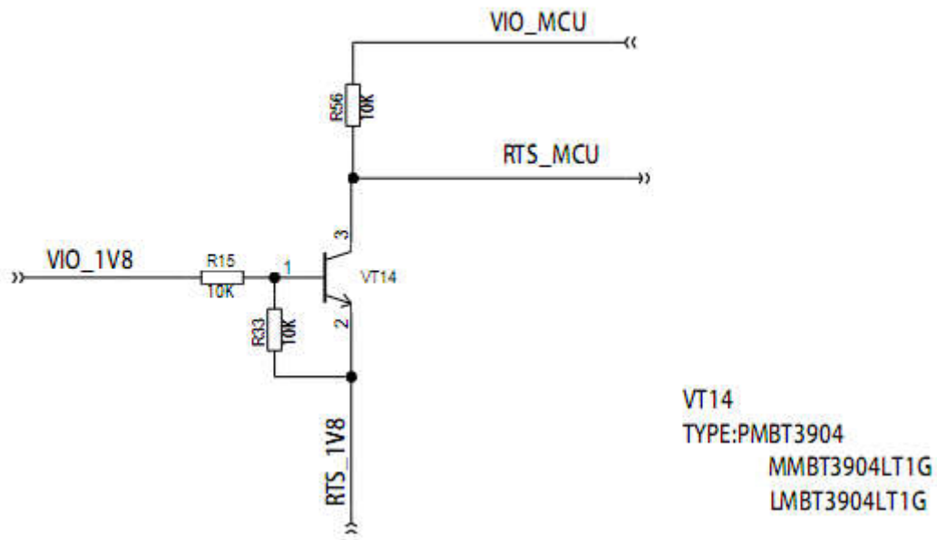
Figure 2-22 Recommended RTS circuit
