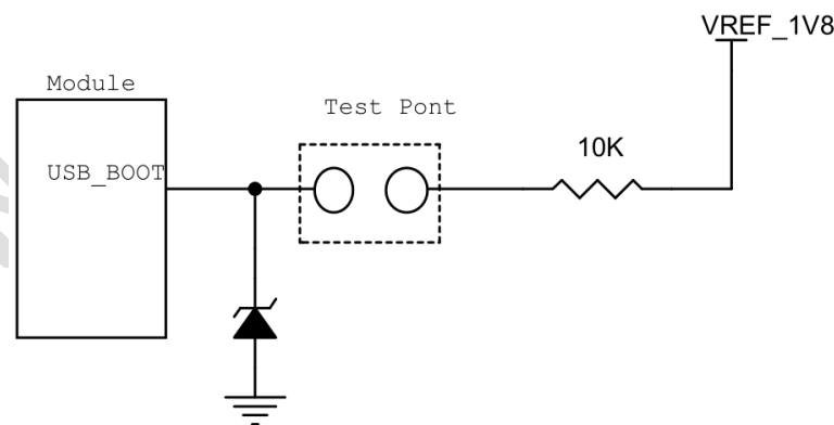
Figure 2-34 USB_BOOTreference design
