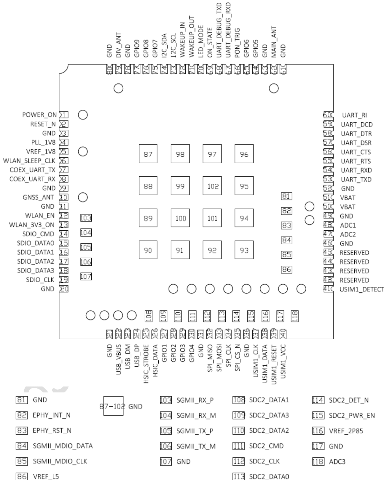
Figure 2-1 Pin Assignment
