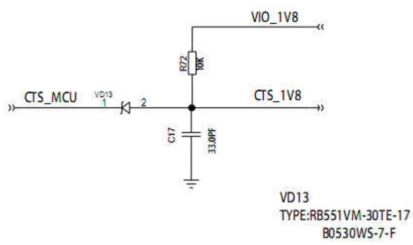
Figure 2-23 Recommended CTS circuit
