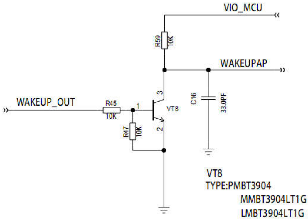
Figure 2-33 WAKEUP_OUTreference design
