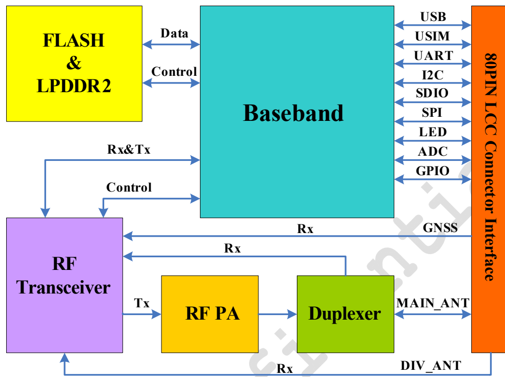
Figure 1–1System Connection Structure
