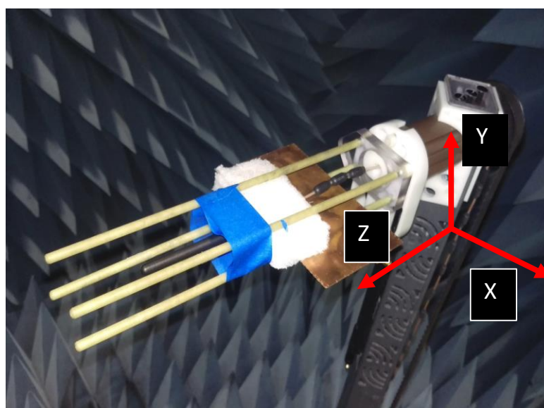
Chamber Setup
