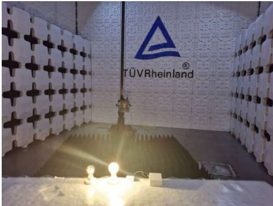
Photograph 5: Set-up photo for Radiated Emissions Above 1GHz
