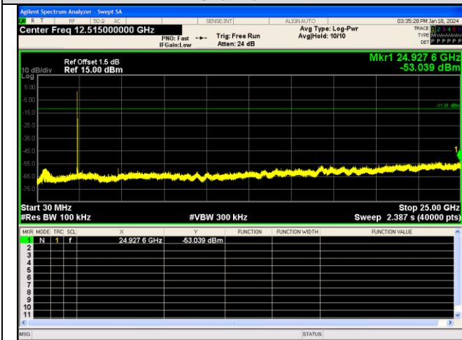
Spurious Emission Channel 11
