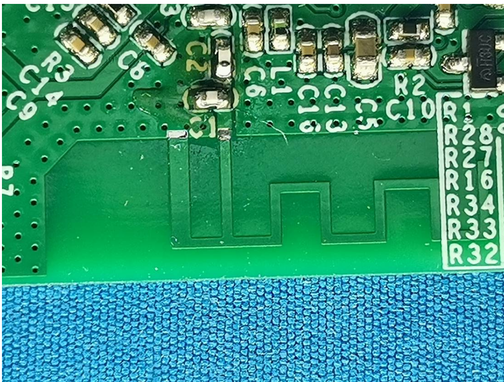
WiFi/BLE Antenna
