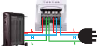
4.2 One wire output instruction (Eg: light).
