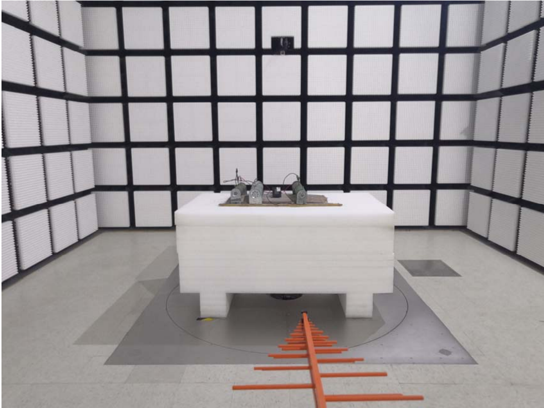
Radiated Emission Below 1GHz View- Model: M5-2C-120
