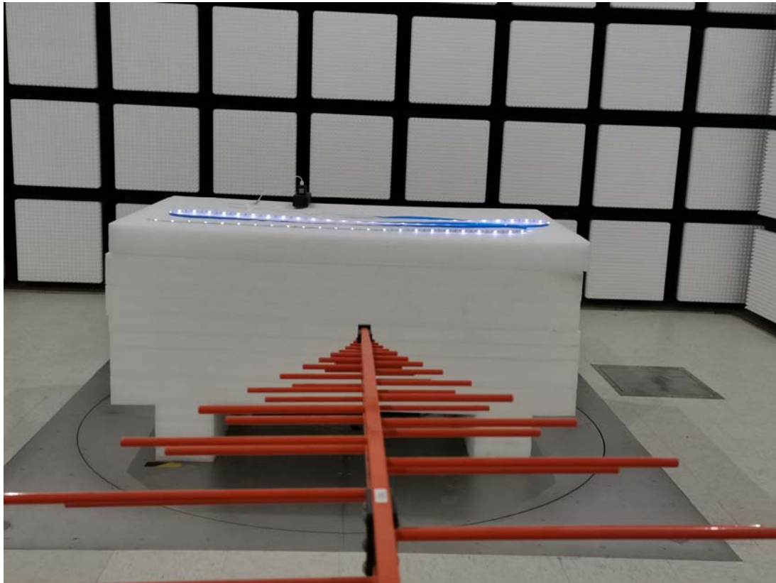
Radiated Emission Below 1GHz View-Model: L3-5M
