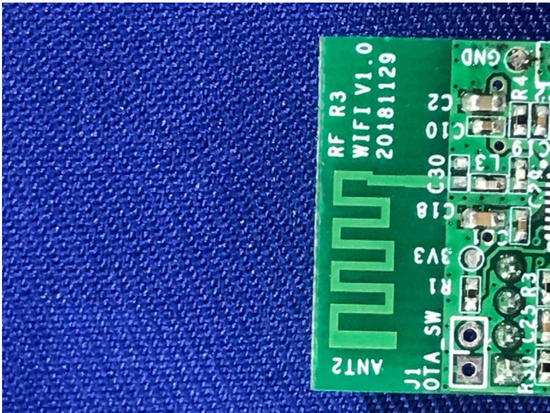
Wi-Fi Antenna
