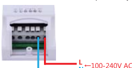
4.1 2 appliances Wiring Instruction.
