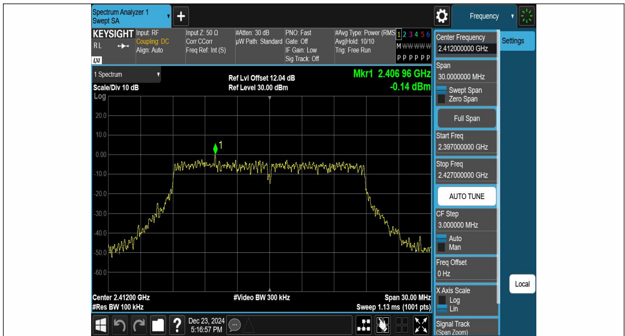
11N20SISO-Ant1-2412-0~Reference-PASS
