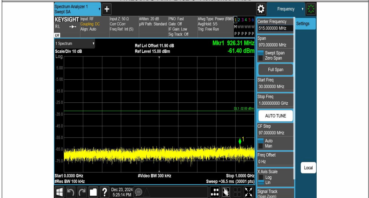
11N20SISO-Ant1-2462-30~1000-PASS
