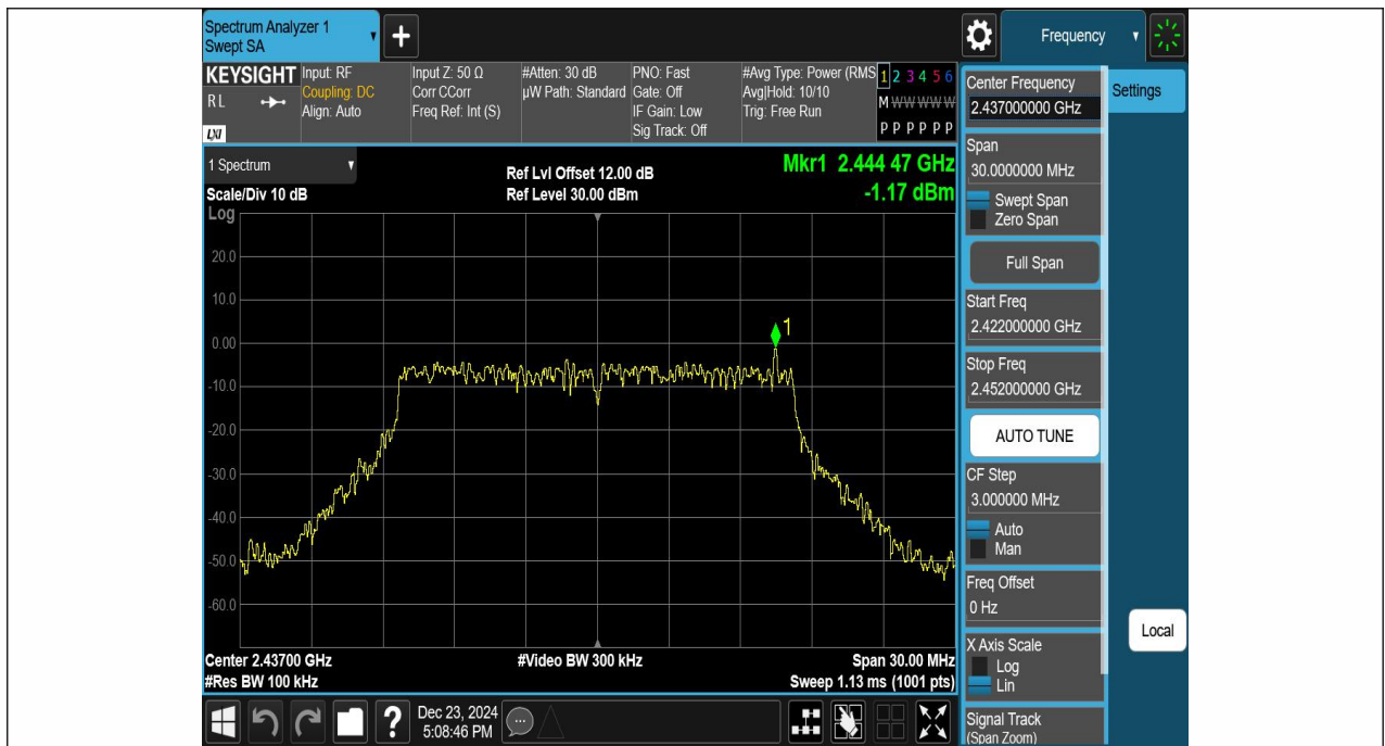
11G-Ant1-2437-0~Reference-PASS
