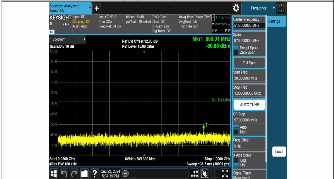
11N40SISO-Ant1-2437-30~1000-PASS
