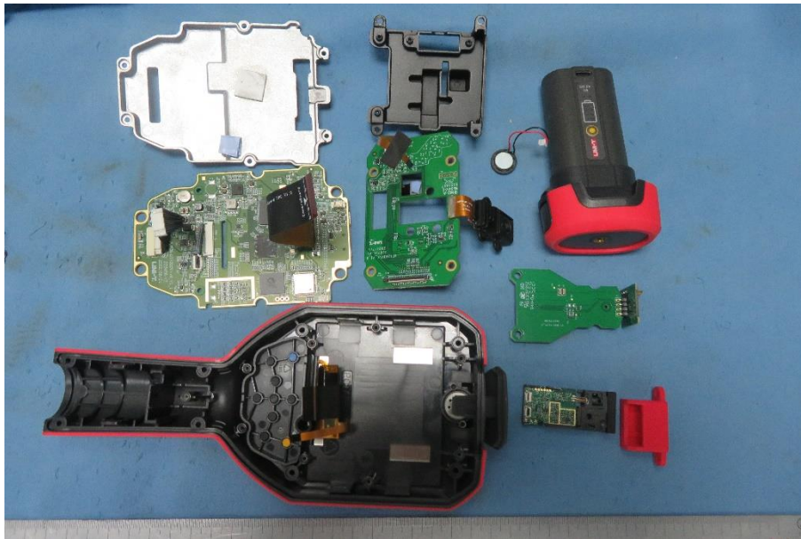
Internal view of model UTi260V, UTi260E
