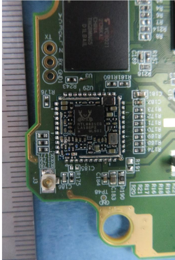
Model UTi320E has not M1 laser ranging module
