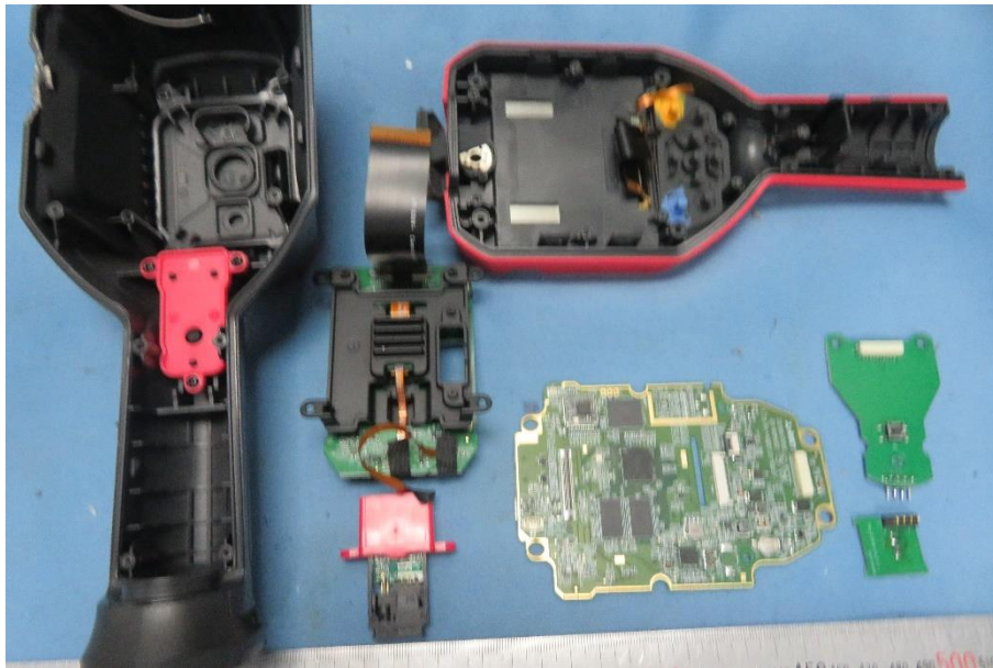
Internal view of model UTi320V+, UTi320E
