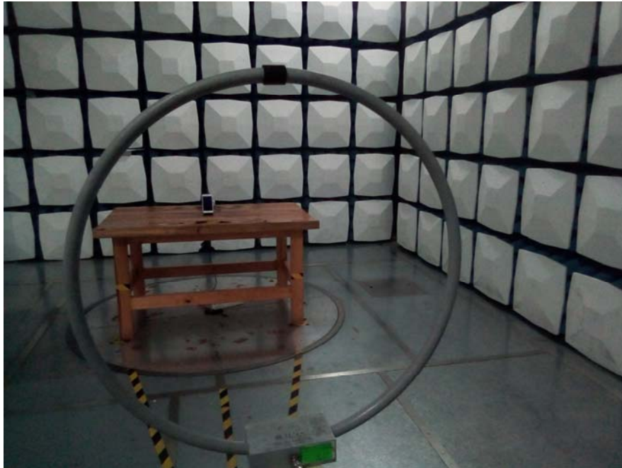
Radiated Emission View (9 kHz~30 MHz) for Power Transmission
