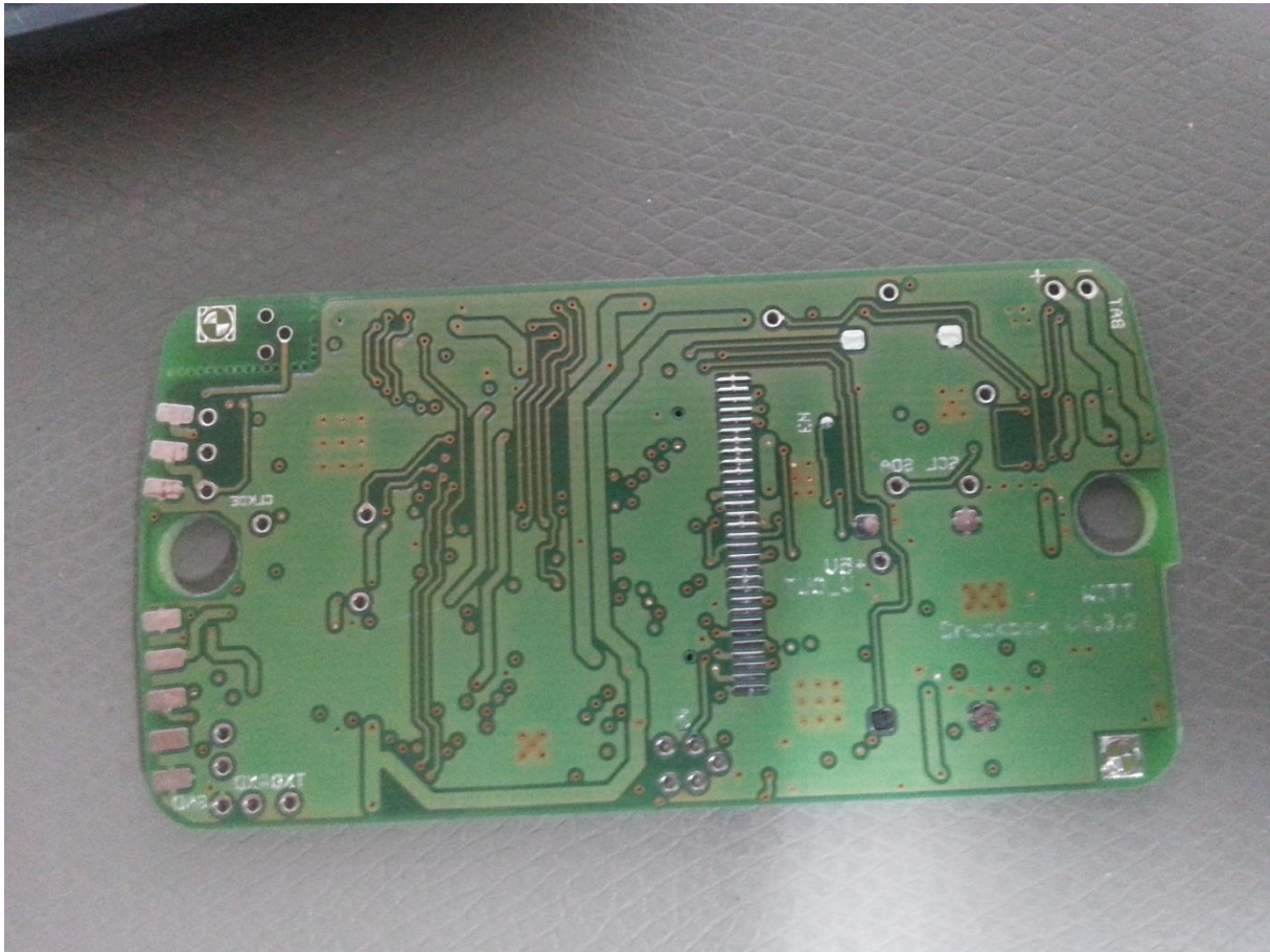
Figure 8: PCB Baseboard (bottom side)
