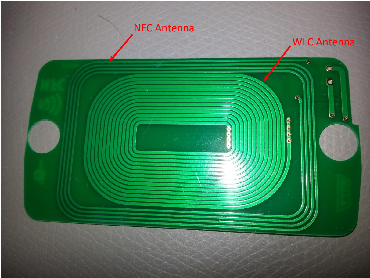
Figure 2: Antenna Board (bottom side)
