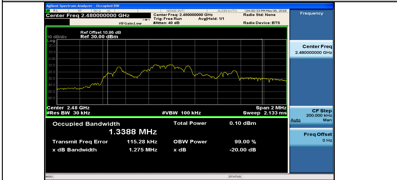
Occupied Bandwidth_3DH5_2480
