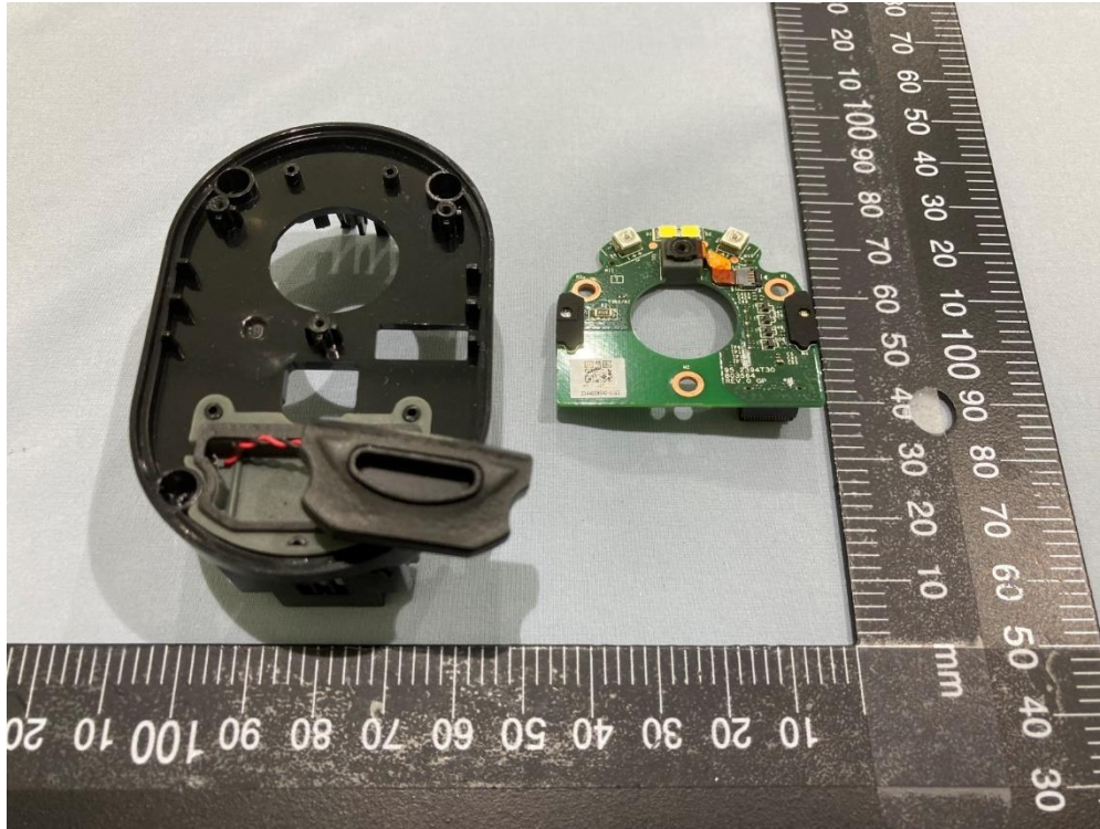
VMC4060P Pic 31
