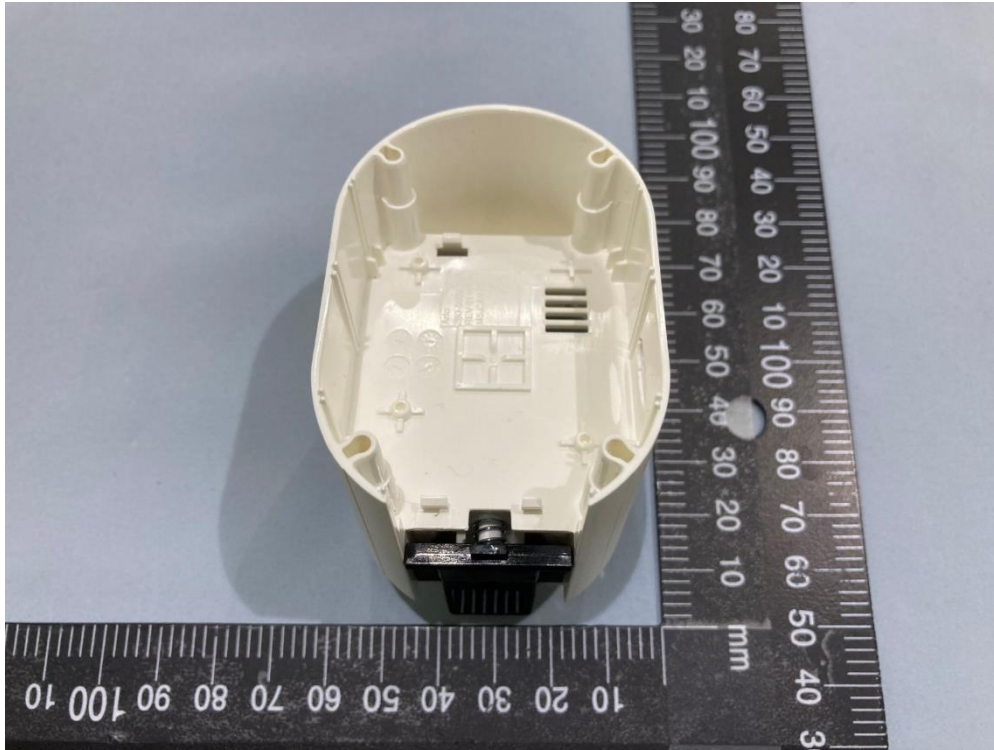
VMC4060P Pic 7
