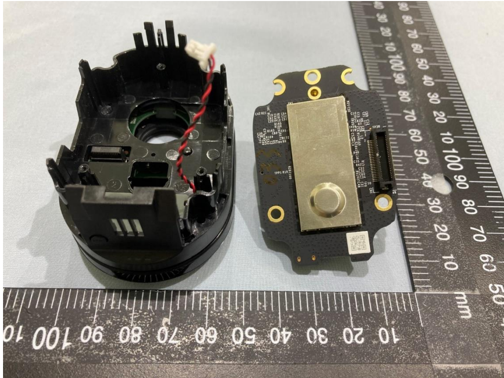
VMC4060P Pic 22
