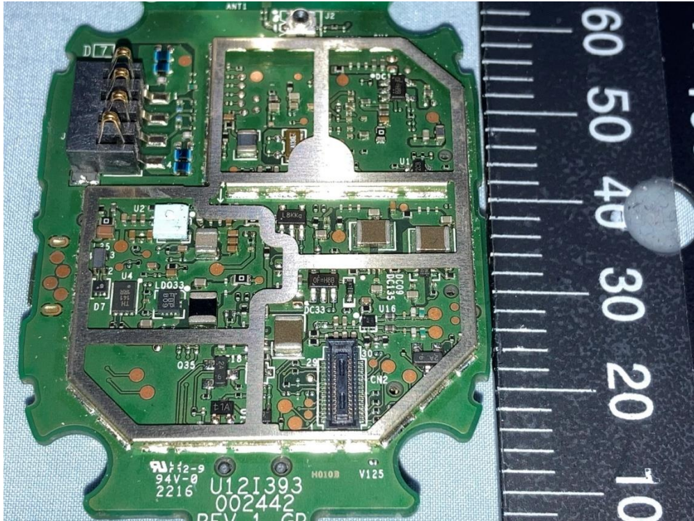
VMC4060P Pic 14
