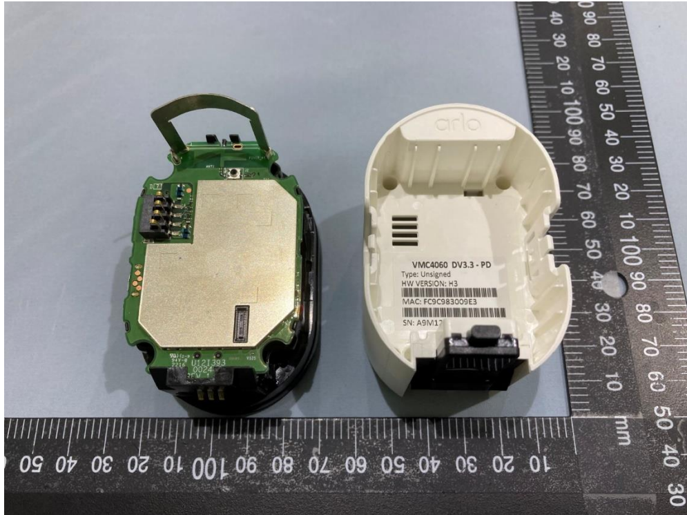
VMC4060P Pic 6
