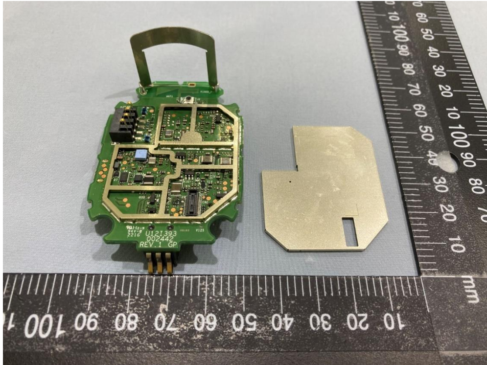
VMC4060P Pic 12
