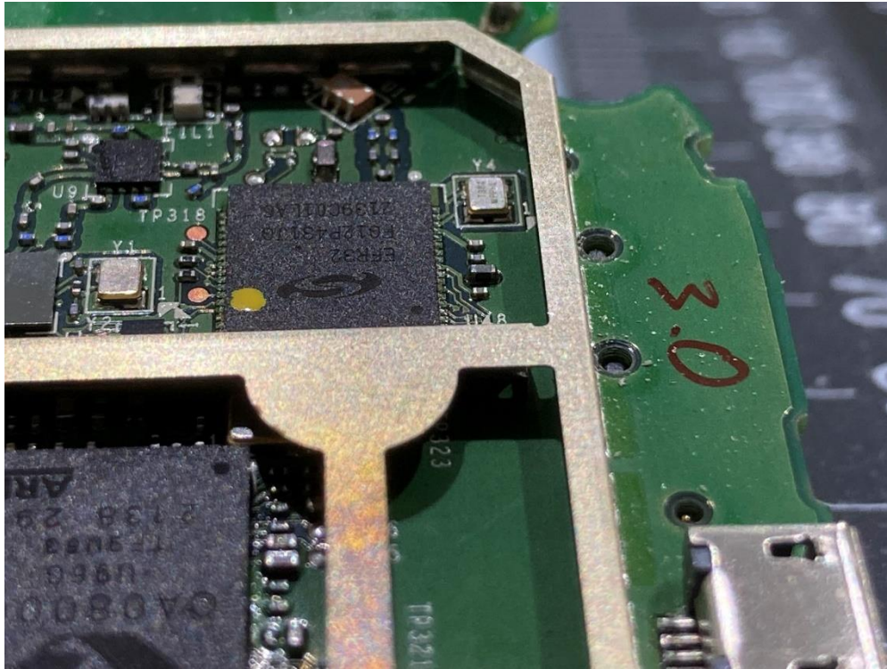
VMC4060P Pic 19
