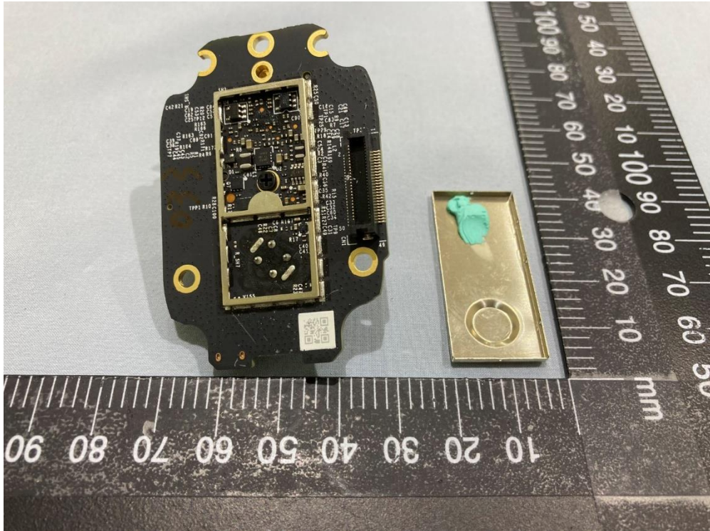
VMC4060P Pic 26
