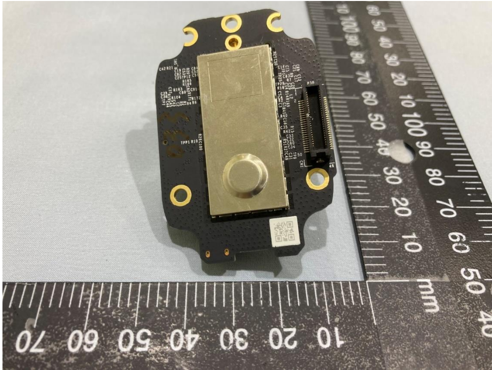
VMC4060P Pic 23
