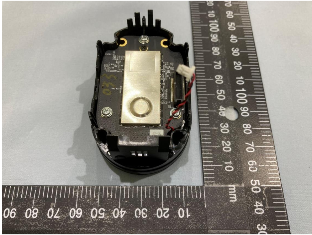
VMC4060P Pic 21
