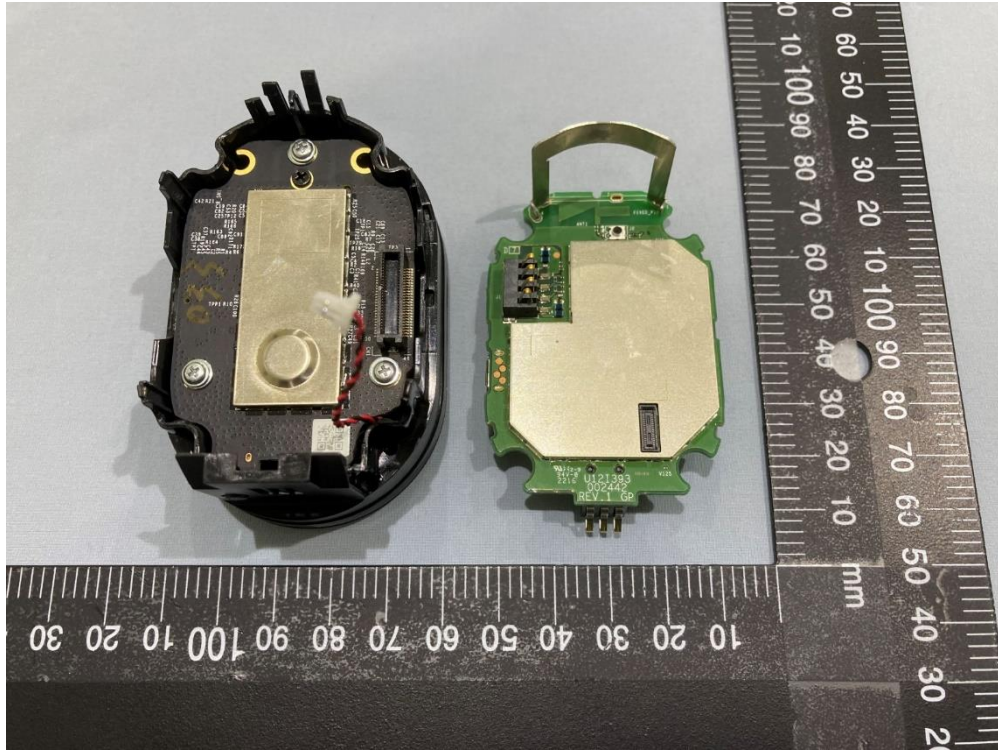
VMC4060P Pic 9
