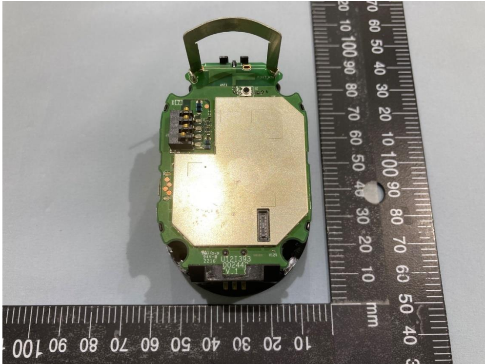
VMC4060P Pic 8
