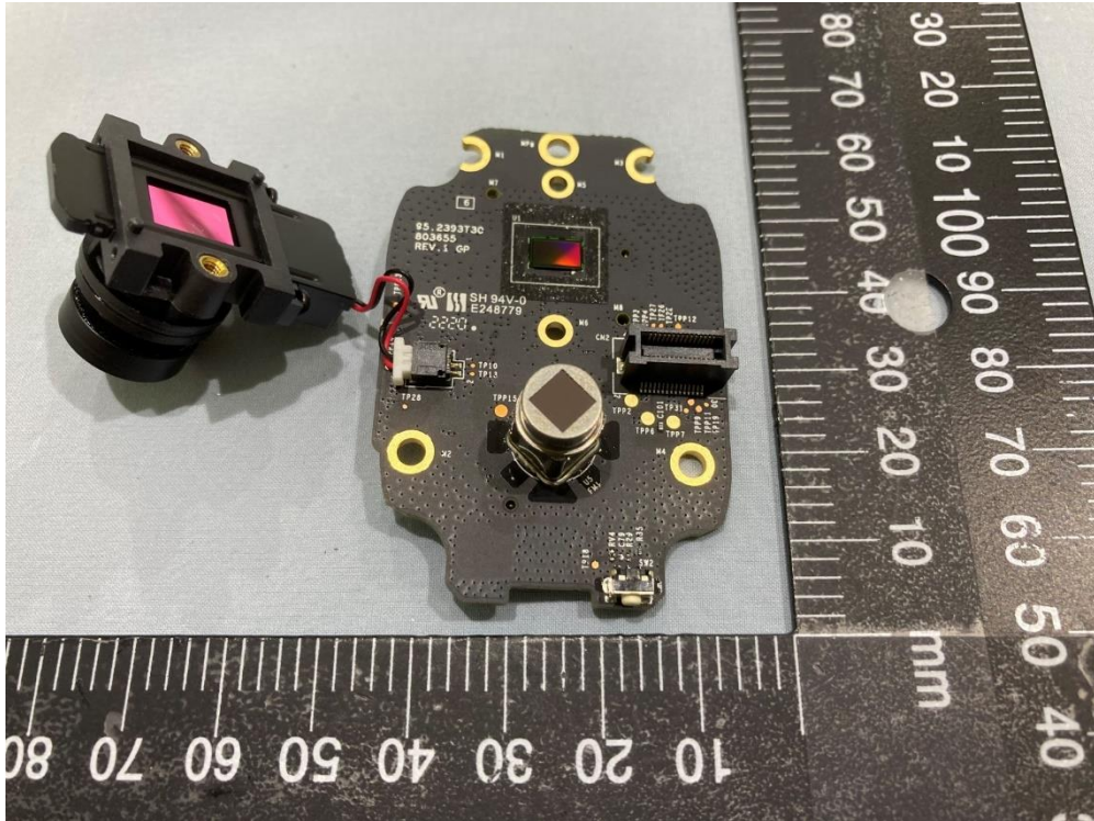
VMC4060P Pic 28
