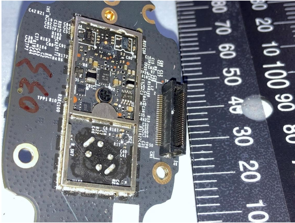
VMC4060P Pic 27
