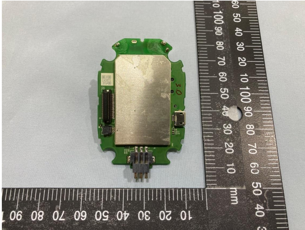
VMC4060P Pic 11
