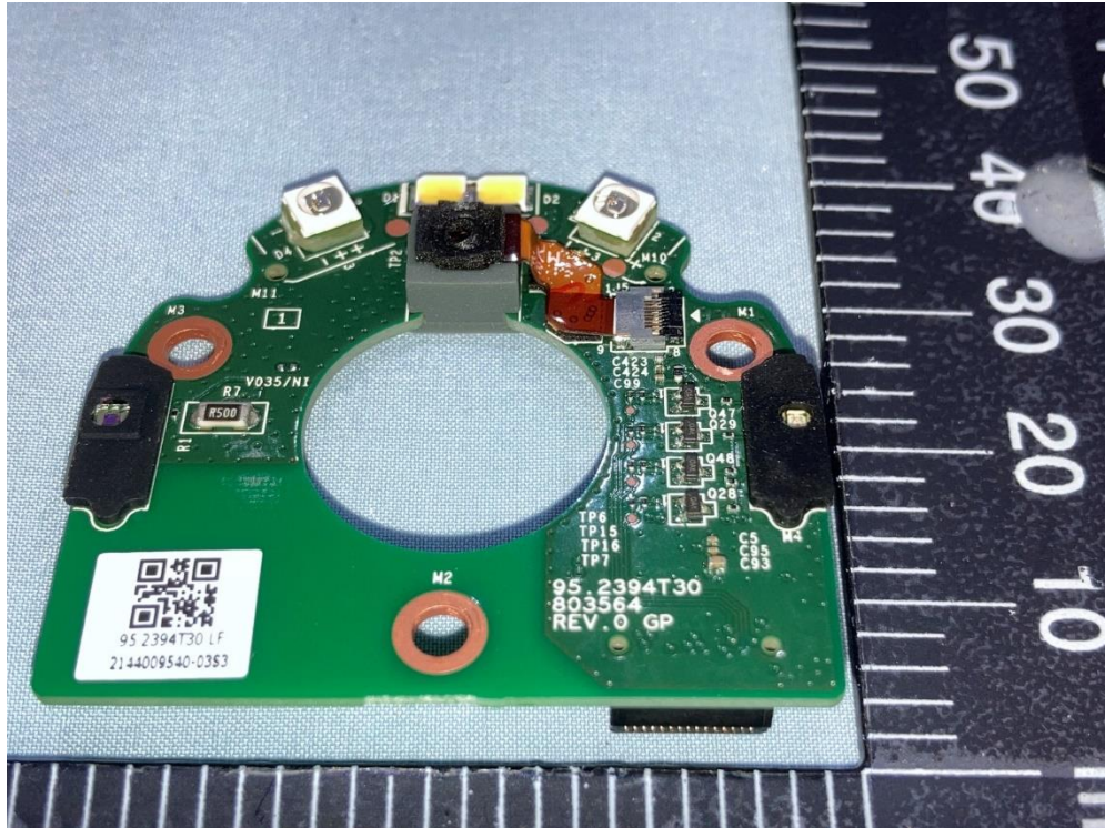
VMC4060P Pic 32
