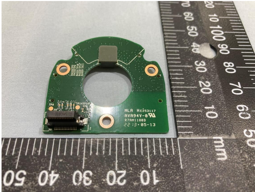
VMC4060P Pic 33
