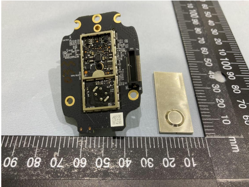
VMC4060P Pic 25
