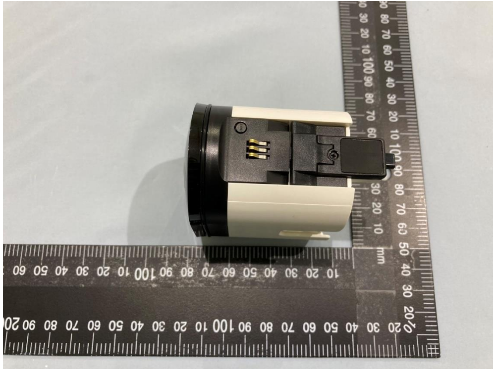
VMC4060P Pic 4
