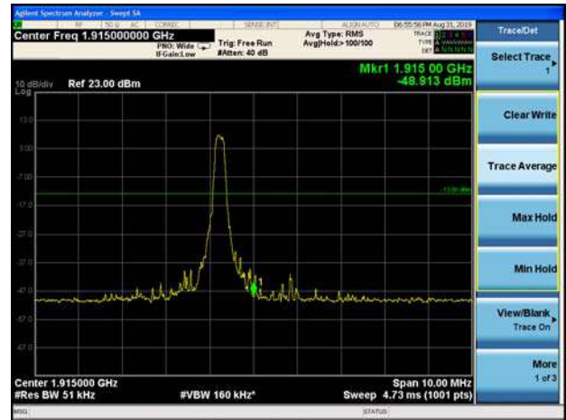
LTE Band 25 10MHz QPSK 100%RB CH-High
