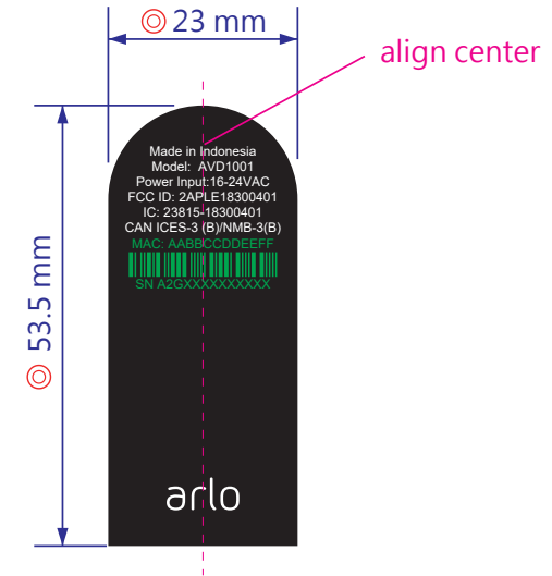
Printing Content for factory 工廠端印刷內容 Printing color: White
