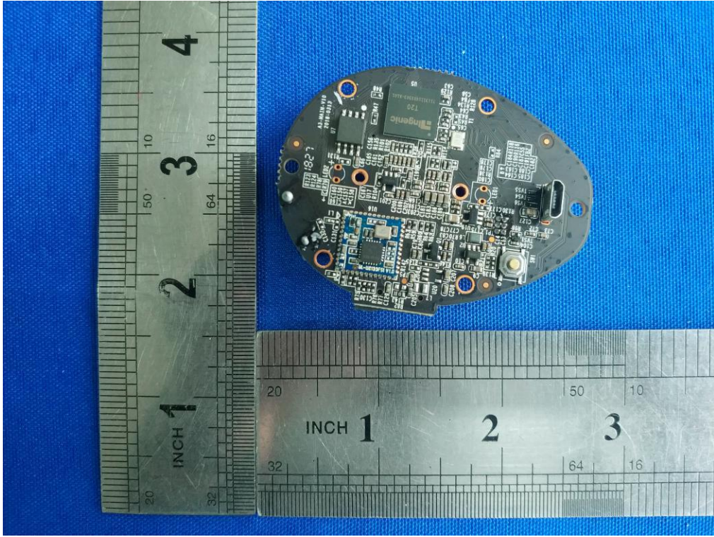
Internal Antenna
