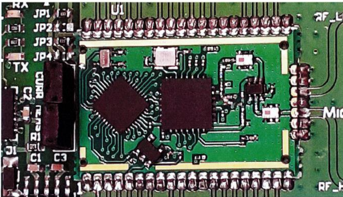
Components of Microchip RN2903A with shield opened top side
