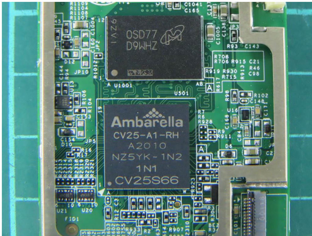
(43) EUT Photo
