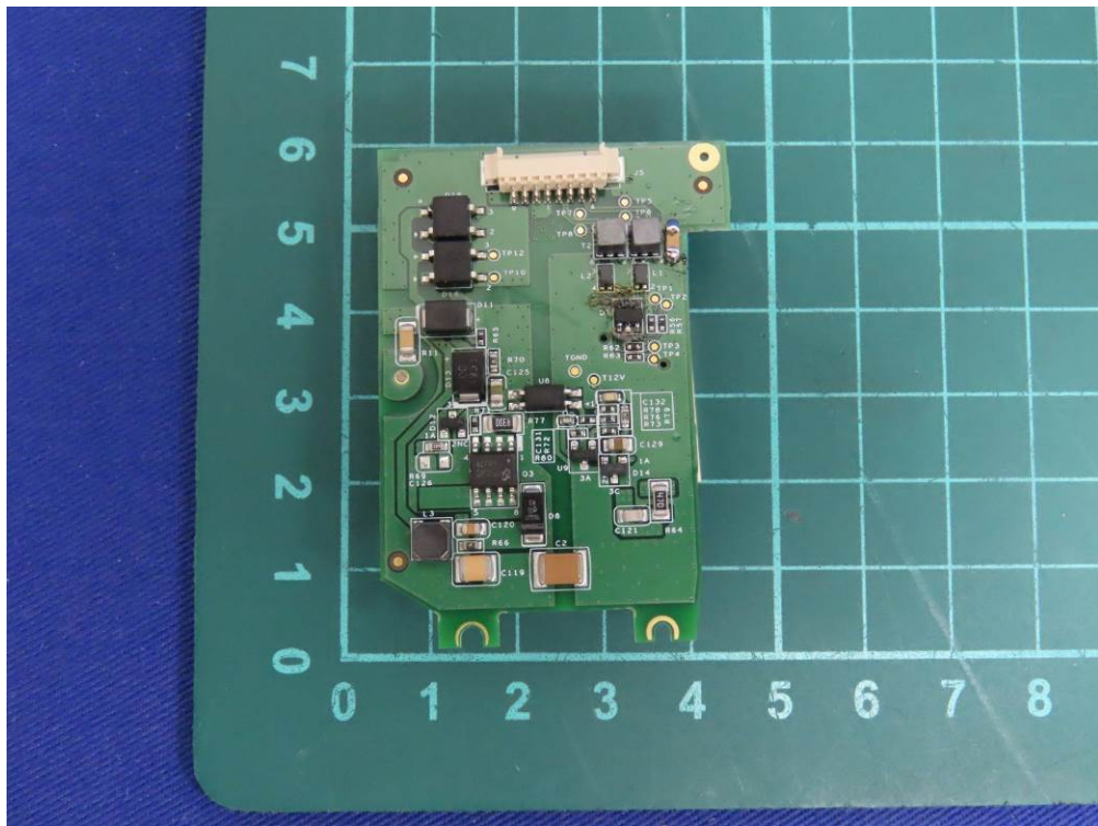
(51) EUT Photo
