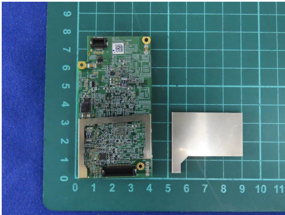
(45) EUT Photo
