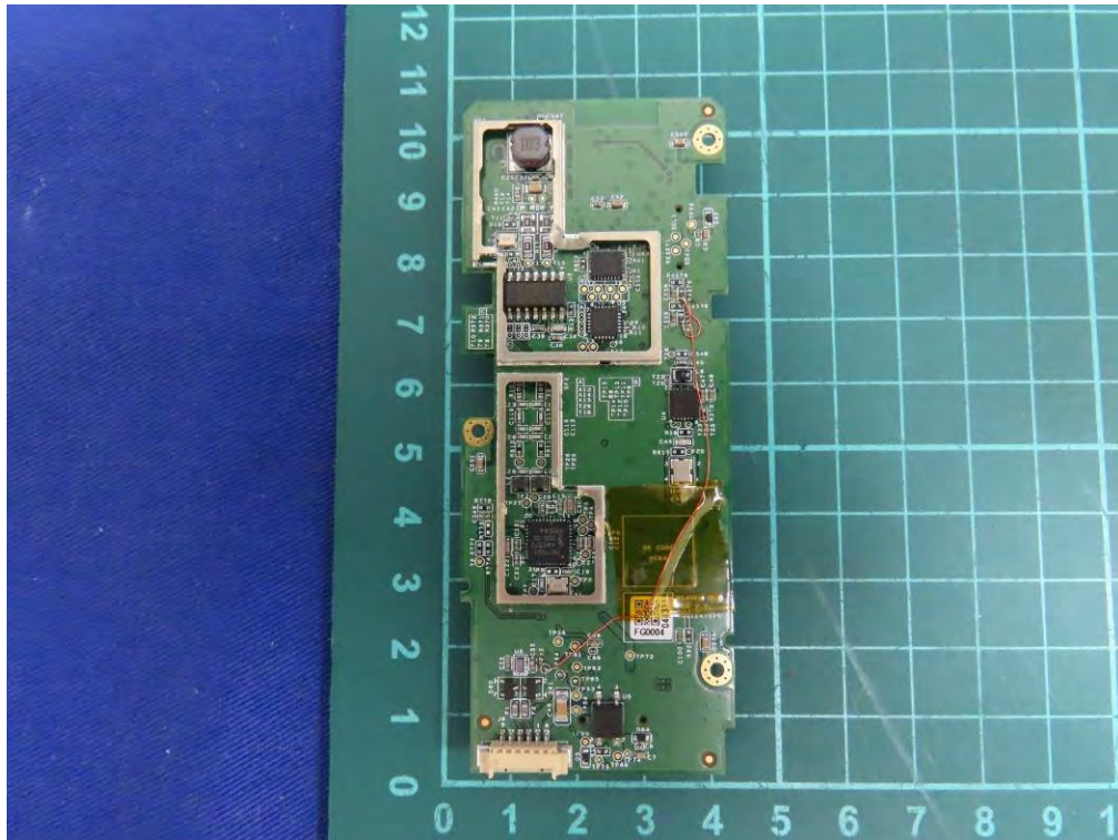
(27) EUT Photo
