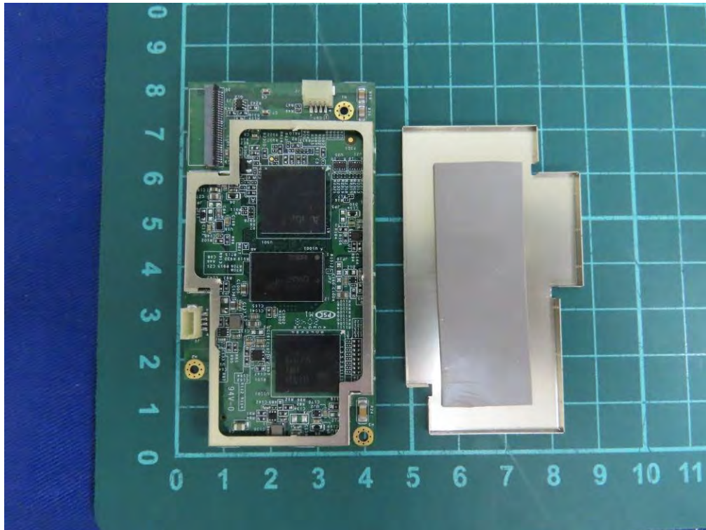
(55) EUT Photo
