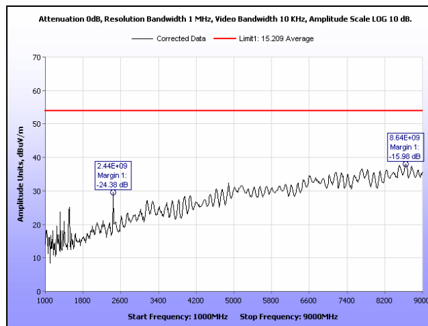
Plot 8. Radiated Spurious Emissions, Mid Channel, 1 GHz – 9 GHz, Average
