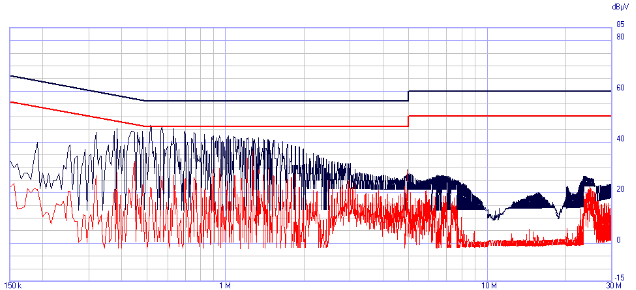
Plot 1. Conducted Emissions, Line
