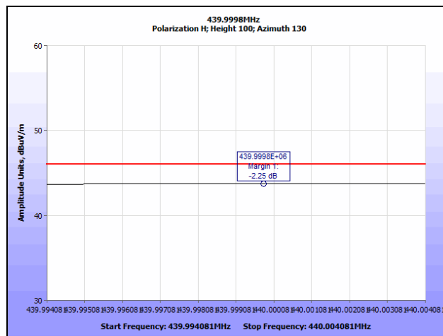
Plot 23. Radiated Spurious Emissions, High Channel, 439.9998 MHz QP
