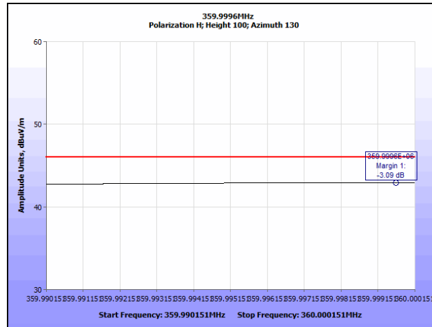
Plot 18. Radiated Spurious Emissions, Low Channel, 359.996 MHz QP
