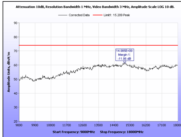
Plot 15. Radiated Spurious Emissions, Mid Channel, 9 GHz – 18 GHz, Peak
