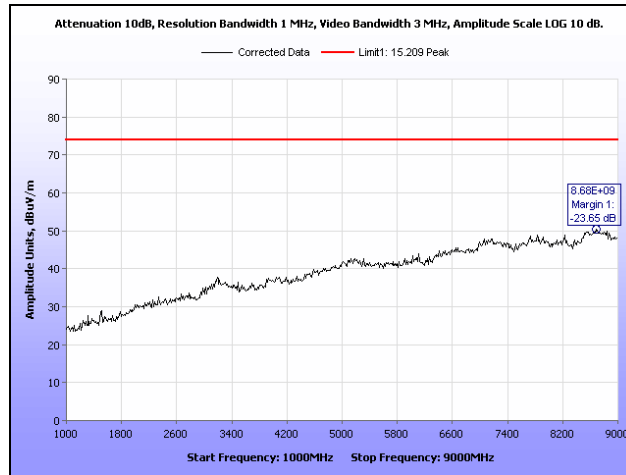
Plot 9. Radiated Spurious Emissions, Mid Channel, 1 GHz – 9 GHz, Peak
