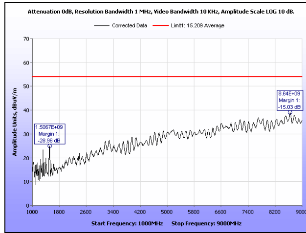
Plot 6. Radiated Spurious Emissions, Low Channel, 1 GHz – 9 GHz, Average
