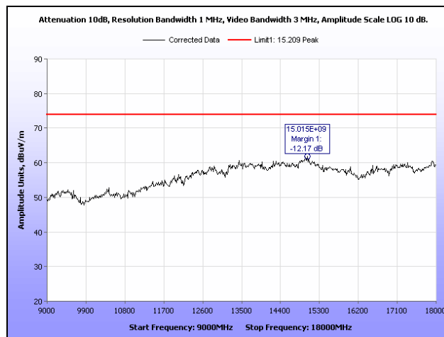
Plot 17. Radiated Spurious Emissions, High Channel, 9 GHz – 18 GHz, Peak
