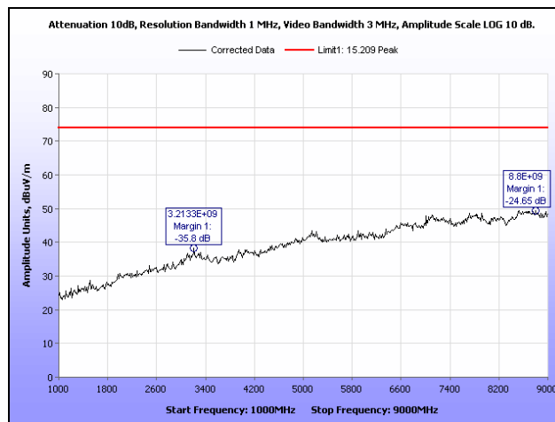
Plot 11. Radiated Spurious Emissions, High Channel, 1 GHz – 9 GHz, Peak
