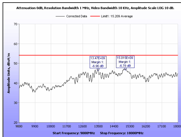
Plot 14. Radiated Spurious Emissions, Mid Channel, 9 GHz – 18 GHz, Average
