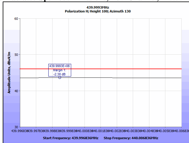
Plot 20. Radiated Spurious Emissions, Mid Channel, 439.9993 MHz QP
