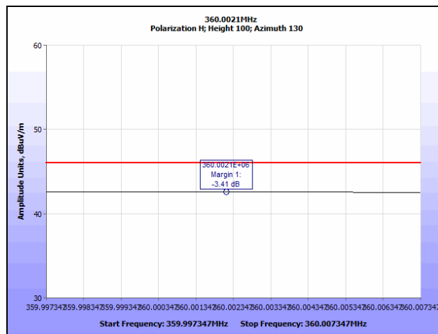
Plot 18. Radiated Spurious Emissions, High Channel, 360.0021 MHz QP
