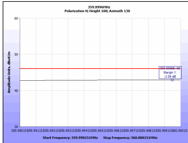
Plot 16. Radiated Spurious Emissions, Low Channel, 359.996 MHz QP
