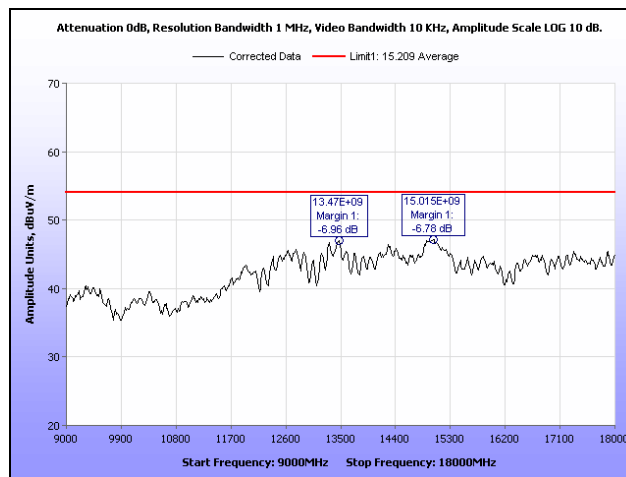
Plot 12. Radiated Spurious Emissions, Mid Channel, 9 GHz – 18 GHz, Average
