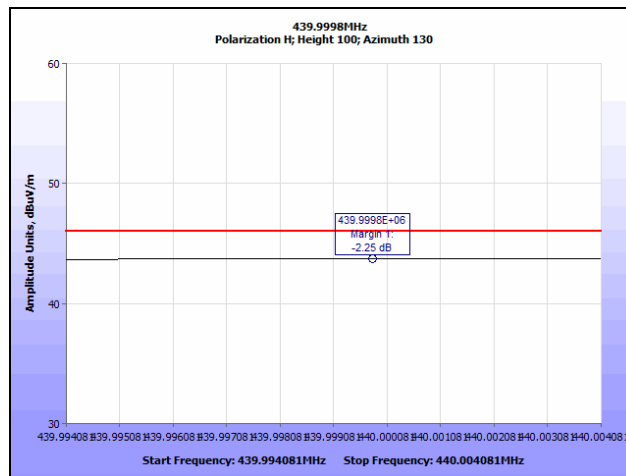
Plot 21. Radiated Spurious Emissions, High Channel, 439.9998 MHz QP
