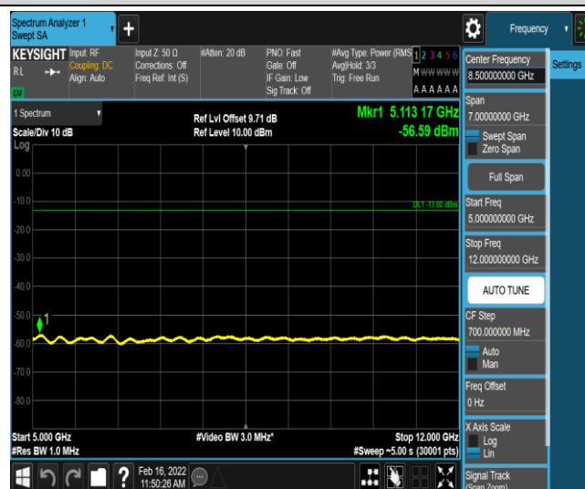
Band66-20MHz-QPSK-132572-1-0-High-5000-12000--56.59-PASS
