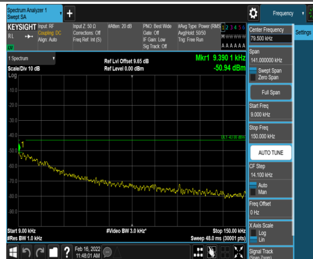
Band66-20MHz-16QAM-132322-1-0-Low-0.009-0.15--50.94-PASS
