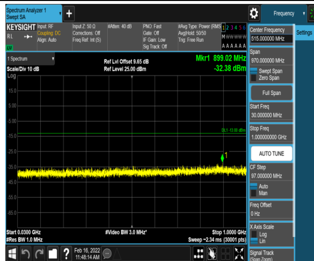
Band66-20MHz-16QAM-132322-1-0-Low-30-1000--32.38-PASS
