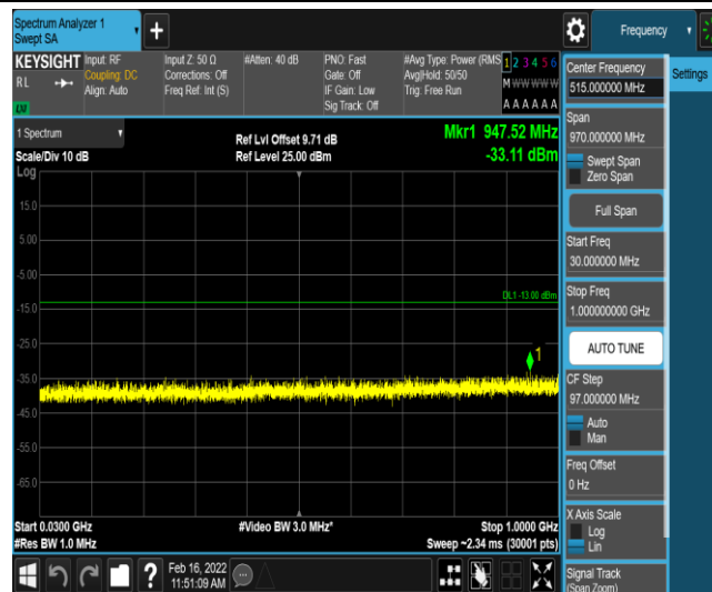
Band66-20MHz-16QAM-132572-1-0-High-30-1000--33.11-PASS
