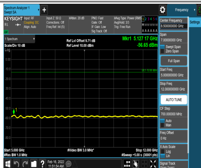
Band66-20MHz-16QAM-132572-1-0-High-5000-12000--56.65-PASS
