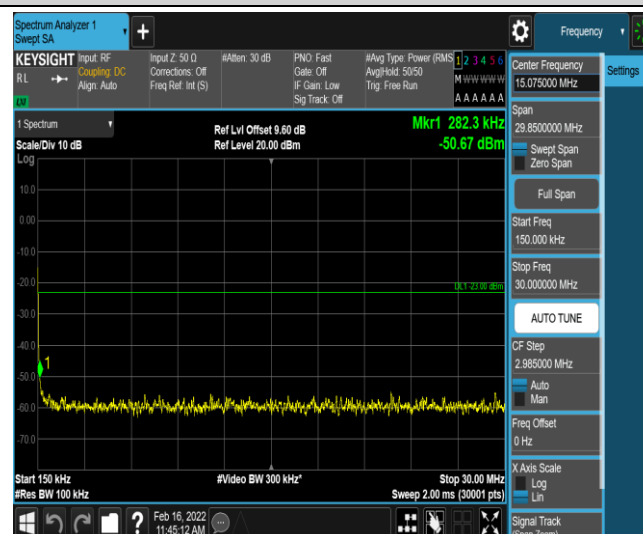
Band66-20MHz-16QAM-132072-1-0-Low-0.15-30--50.67-PASS
