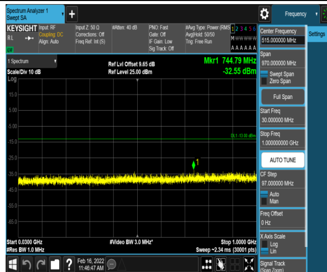
Band66-20MHz-QPSK-132322-1-0-Low-30-1000--32.55-PASS
