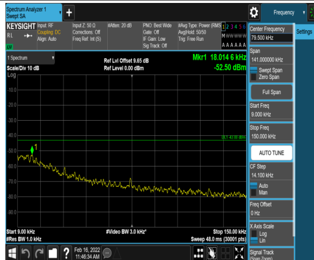
Band66-20MHz-QPSK-132322-1-0-Low-0.009-0.15--52.5-PASS
