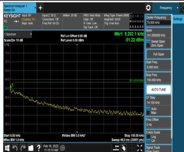
Band66-15MHz-16QAM-132047-1-0-Low-0.009-0.15--51.22-PASS
