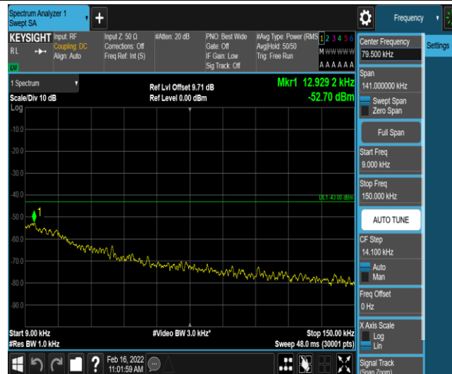
Band66-10MHz-QPSK-132622-1-0-High-0.009-0.15--52.7-PASS
