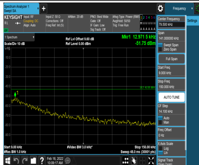
Band66-10MHz-QPSK-132022-1-0-Low-0.009-0.15--51.75-PASS
