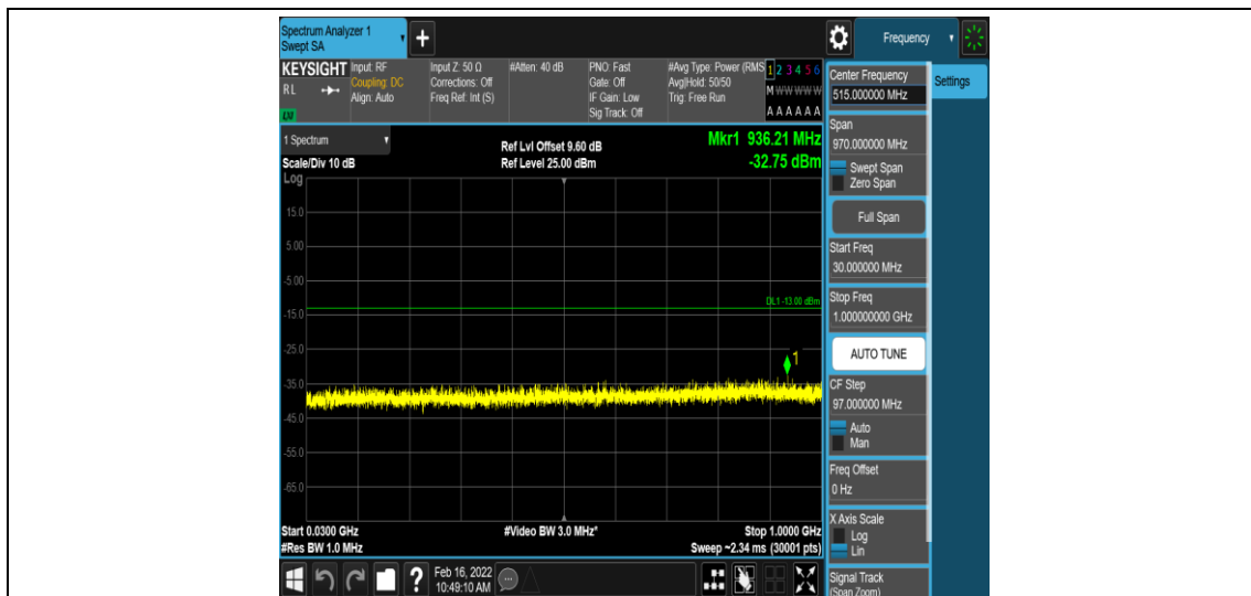
Band66-10MHz-16QAM-132022-1-0-Low-30-1000--32.75-PASS
