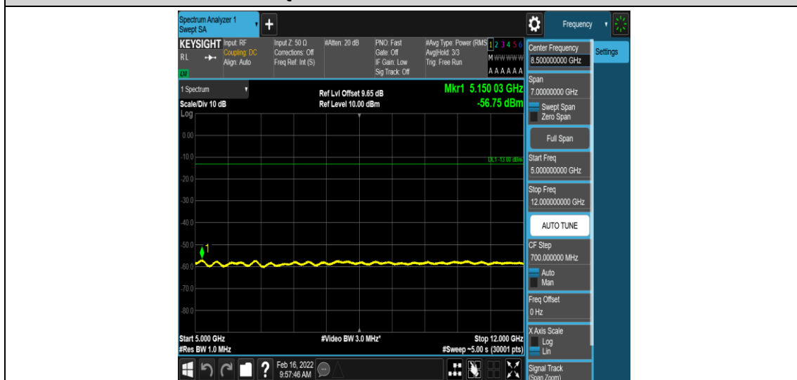
Band66-5MHz-16QAM-132322-1-0-Low-5000-12000--56.75-PASS
