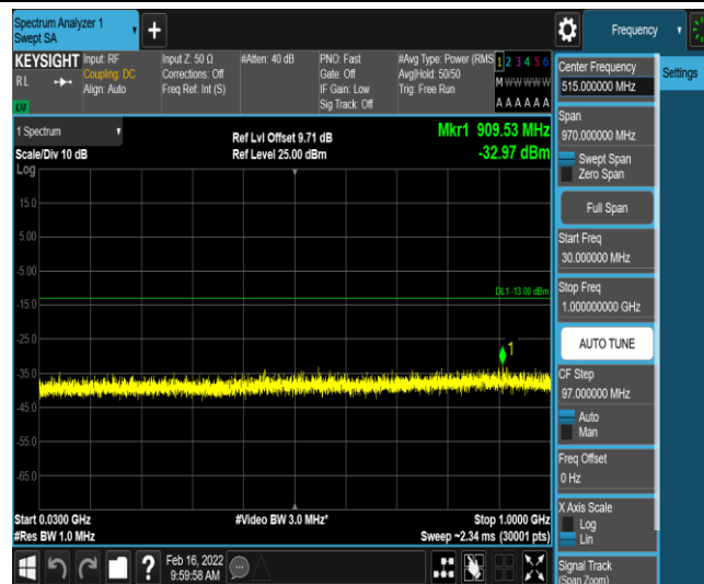
Band66-5MHz-16QAM-132647-1-0-High-30-1000--32.97-PASS
