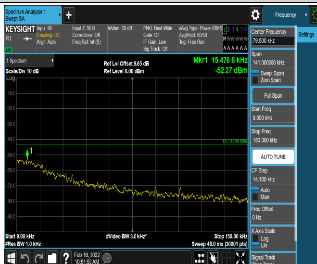
Band66-10MHz-16QAM-132322-1-0-Low-0.009-0.15--52.27-PASS
