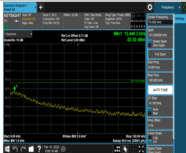
Band66-5MHz-QPSK-132647-1-0-High-0.009-0.15--52.52-PASS
