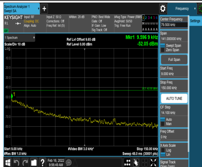
Band66-5MHz-16QAM-132322-1-0-Low-0.009-0.15--52.05-PASS
