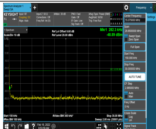
Band66-5MHz-16QAM-131997-1-0-Low-0.15-30--48.89-PASS
