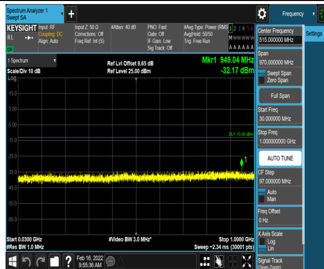
Band66-5MHz-QPSK-132322-1-0-Low-30-1000--32.17-PASS
