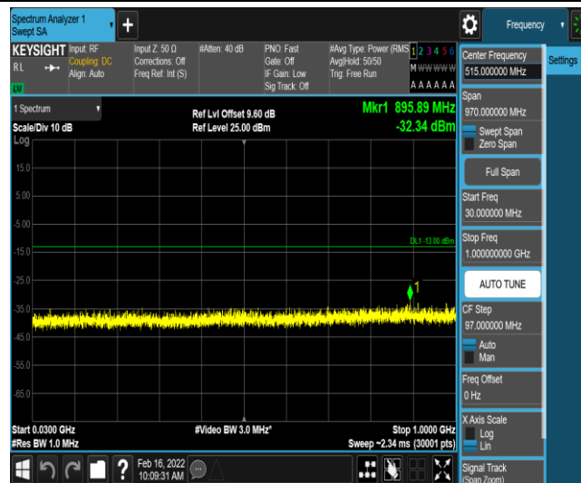
Band66-10MHz-QPSK-132022-1-0-Low-30-1000--32.34-PASS
