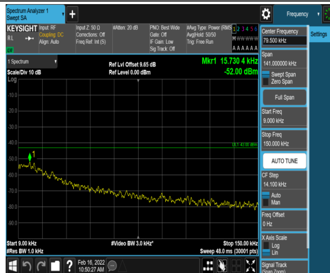
Band66-10MHz-QPSK-132322-1-0-Low-0.009-0.15--52-PASS
