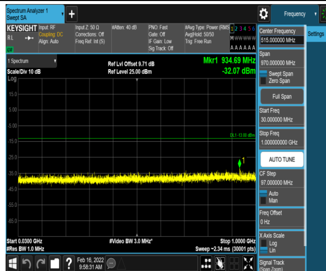
Band66-5MHz-QPSK-132647-1-0-High-30-1000--32.07-PASS
