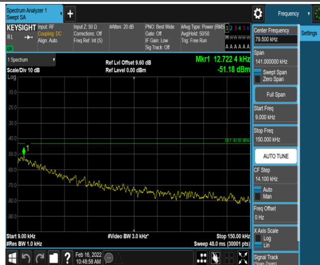
Band66-10MHz-16QAM-132022-1-0-Low-0.009-0.15--51.19-PASS
