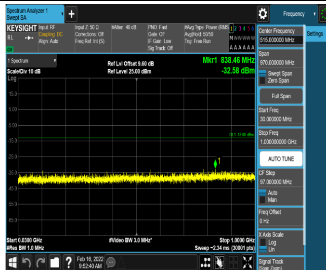
Band66-5MHz-QPSK-131997-1-0-Low-30-1000--32.58-PASS
