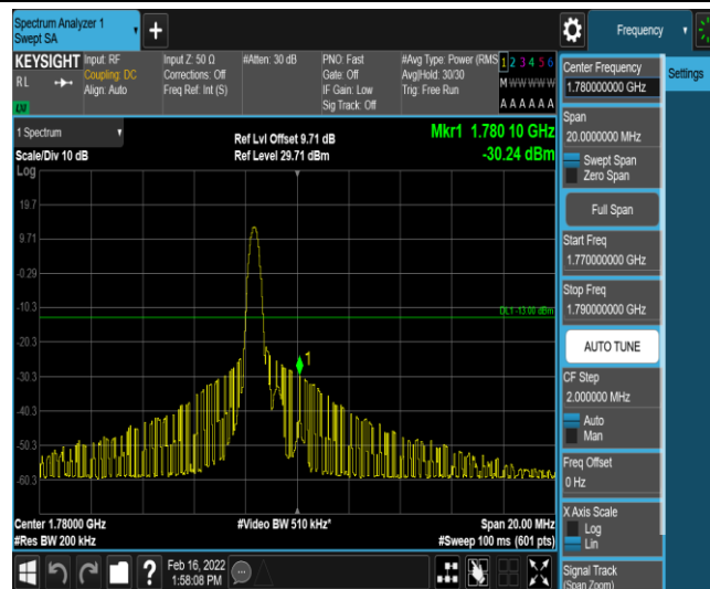
Band66-10MHz-QPSK-132622-1-0-High--30.24-PASS
