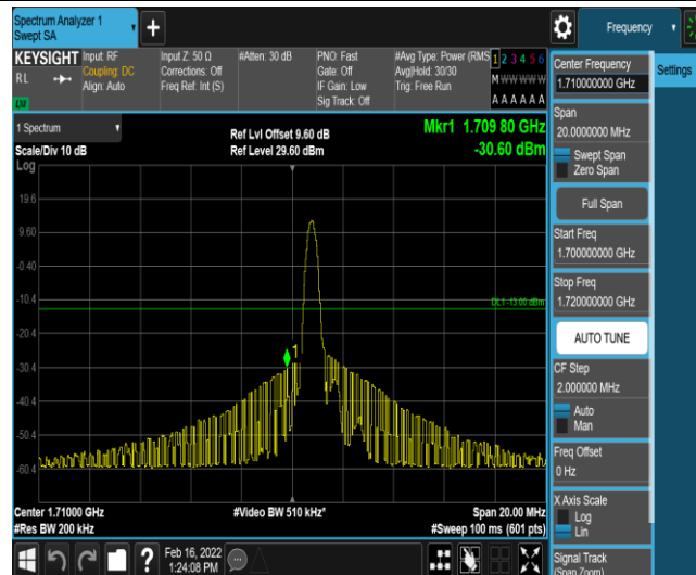
Band66-10MHz-QPSK-132022-1-0-Low--30.60-PASS
