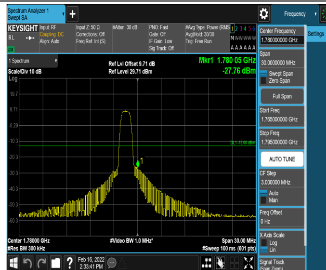
Band66-15MHz-16QAM-132597-6-0-High--27.76-PASS
