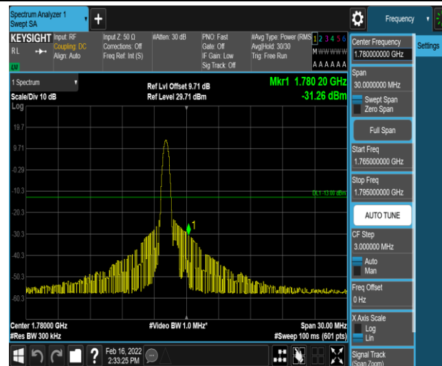
Band66-15MHz-16QAM-132597-1-0-High--31.26-PASS
