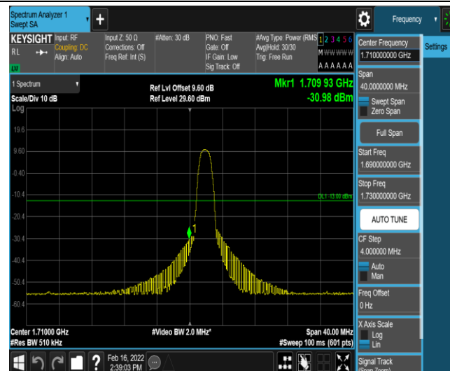
Band66-20MHz-16QAM-132072-6-0-Low--30.98-PASS
