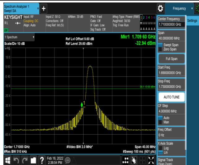
Band66-20MHz-QPSK-132072-6-0-Low--32.94-PASS
