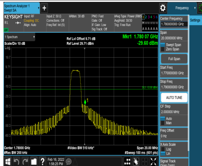
Band66-10MHz-QPSK-132622-6-0-High--29.60-PASS
