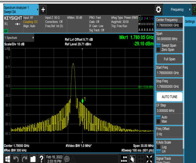
Band66-15MHz-QPSK-132597-1-0-High--29.10-PASS
