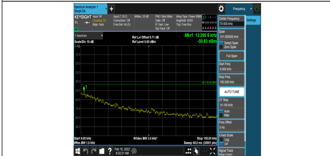
Band66-1.4MHz-QPSK-132665-1-0-High-0.009-0.15--50.84-PASS
