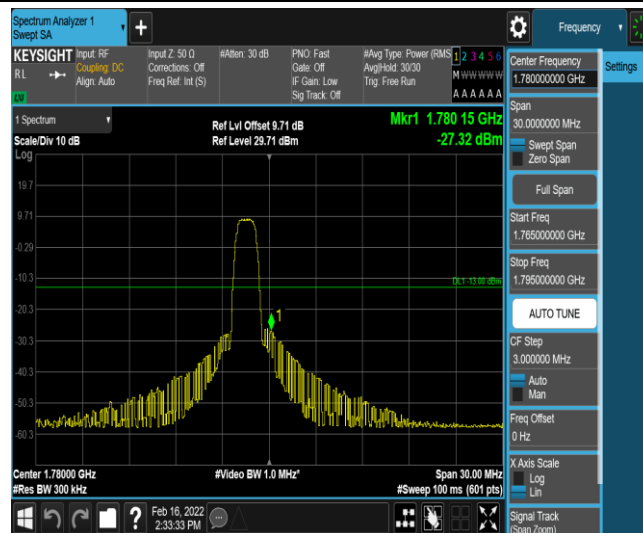
Band66-15MHz-QPSK-132597-6-0-High--27.32-PASS
