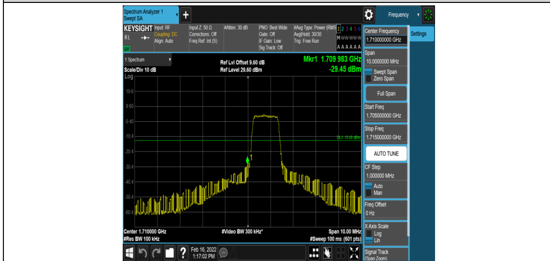
Band66-5MHz-16QAM-131997-6-0-Low--29.45-PASS
