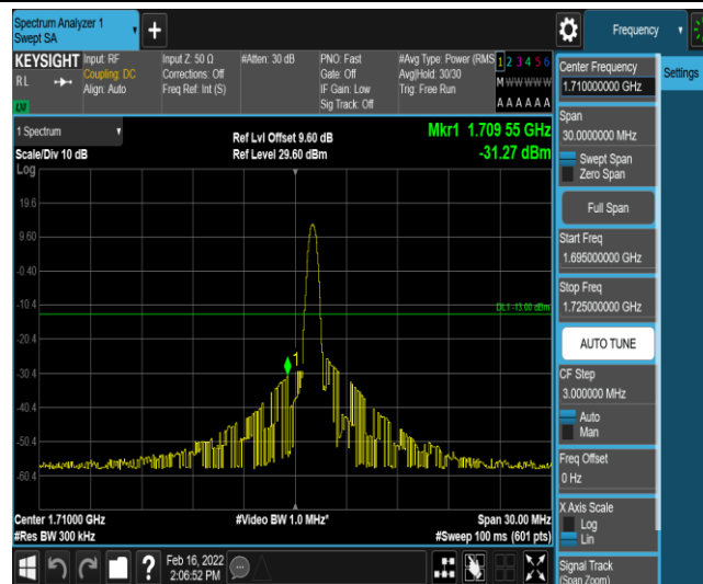
Band66-15MHz-QPSK-132047-1-0-Low--31.27-PASS
