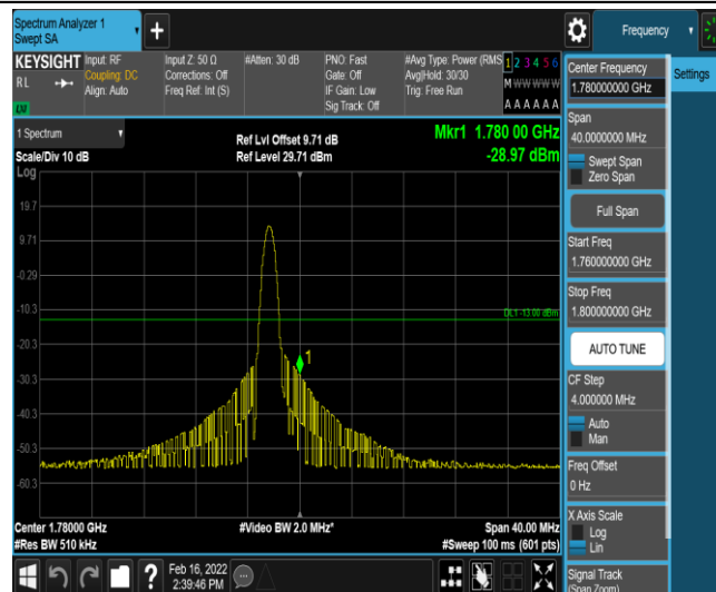
Band66-20MHz-QPSK-132572-1-0-High--28.97-PASS
