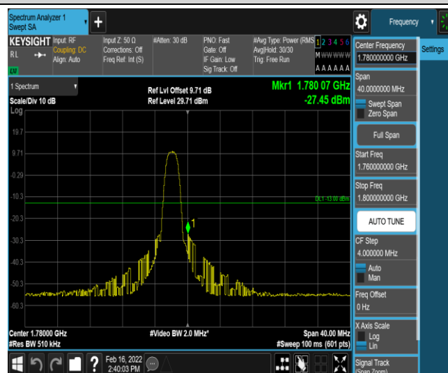
Band66-20MHz-QPSK-132572-6-0-High--27.45-PASS
