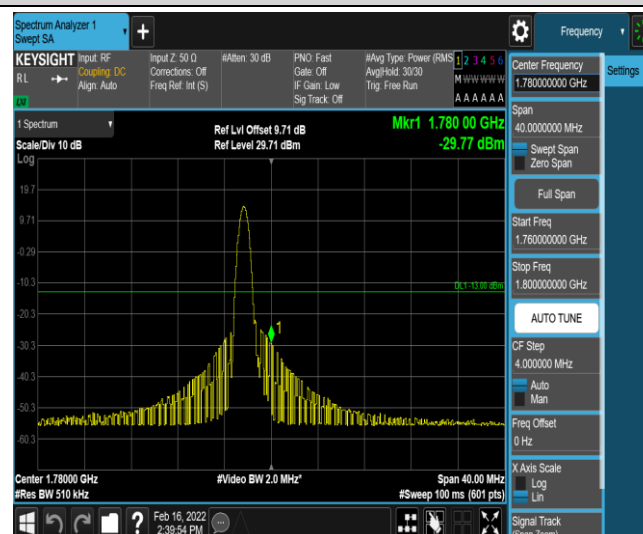
Band66-20MHz-16QAM-132572-1-0-High--29.77-PASS
