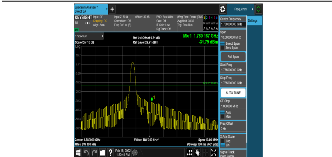
Band66-5MHz-16QAM-132647-1-0-High--31.79-PASS
