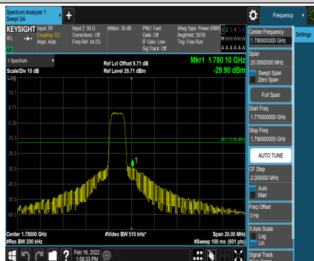
Band66-10MHz-16QAM-132622-6-0-High--29.90-PASS
