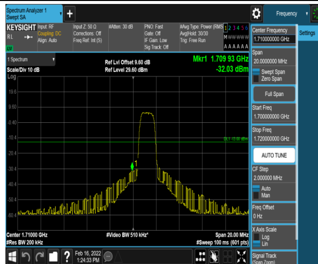
Band66-10MHz-16QAM-132022-6-0-Low--32.03-PASS
