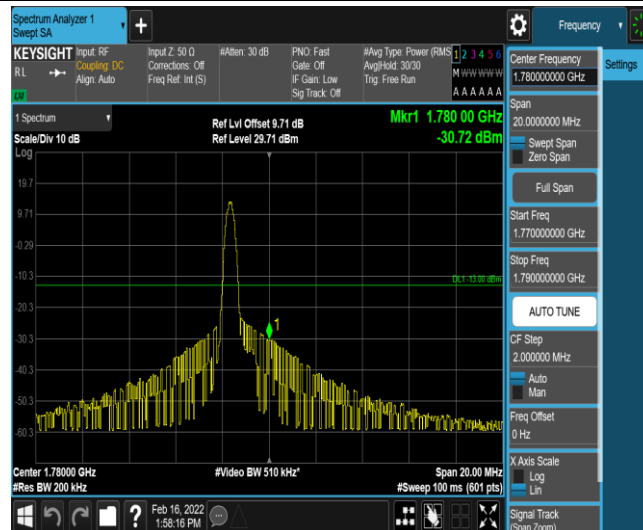
Band66-10MHz-16QAM-132622-1-0-High--30.72-PASS
