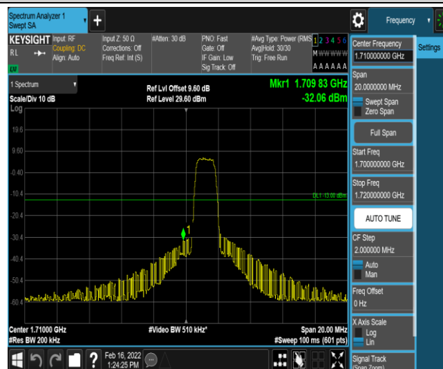
Band66-10MHz-QPSK-132022-6-0-Low--32.06-PASS
