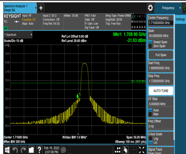
Band66-15MHz-QPSK-132047-6-0-Low--31.03-PASS
