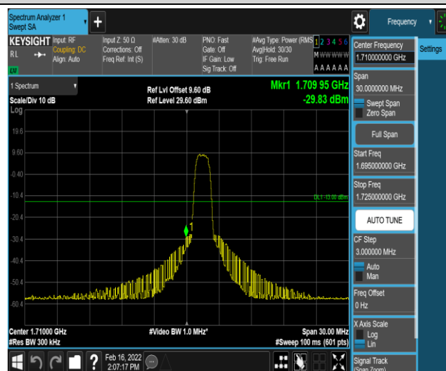
Band66-15MHz-16QAM-132047-6-0-Low--29.83-PASS
