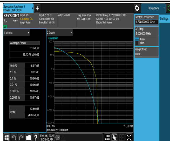
Band66-3MHz-QPSK-132657-1-0-High-10.80-=&lt;=13-PASS
