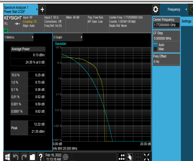
Band66-15MHz-16QAM-132597-1-0-High-9.36-<=13-PASS
