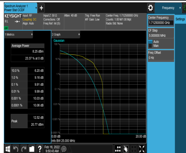
Band66-5MHz-16QAM-131997-1-0-Low-9.91-<=13-PASS
