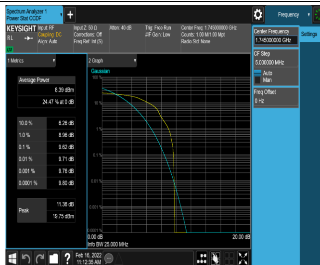
Band66-15MHz-16QAM-132322-1-0-Low-9.62-<=13-PASS
