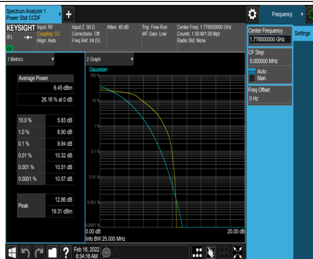
Band66-3MHz-QPSK-132657-6-0-High-9.94-&lt;=13-PASS
