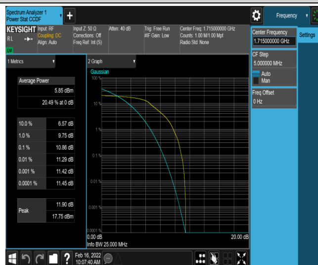
Band66-10MHz-QPSK-132022-6-0-Low-10.86-<=13-PASS
