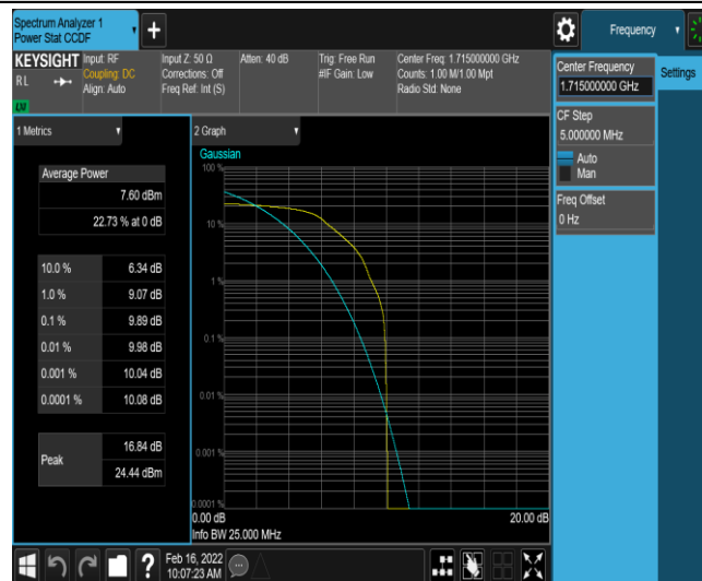
Band66-10MHz-QPSK-132022-1-0-Low-9.89-<=13-PASS
