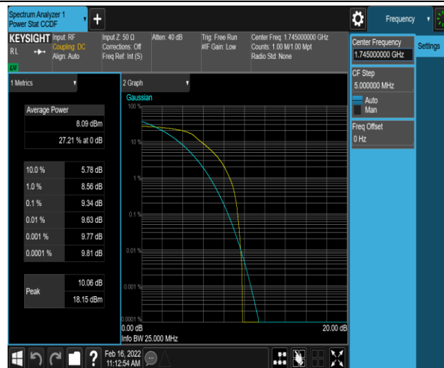
Band66-15MHz-16QAM-132322-6-0-Low-9.34-<=13-PASS
