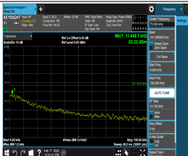
Band26-3MHz-QPSK-26805-1-0-Low-0.009-0.15--53.22-PASS
