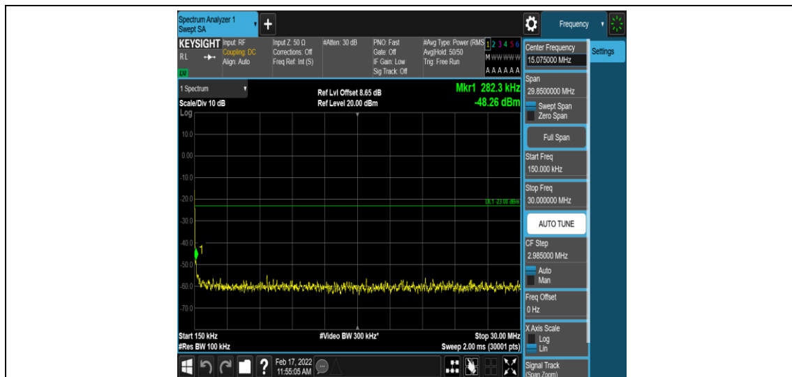
Band26-1.4MHz-16QAM-27033-1-0-High-0.15-30--48.26-PASS
