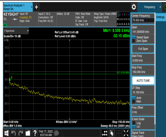
Band26-1.4MHz-16QAM-26783-1-0-High-0.009-0.15--53.15-PASS
