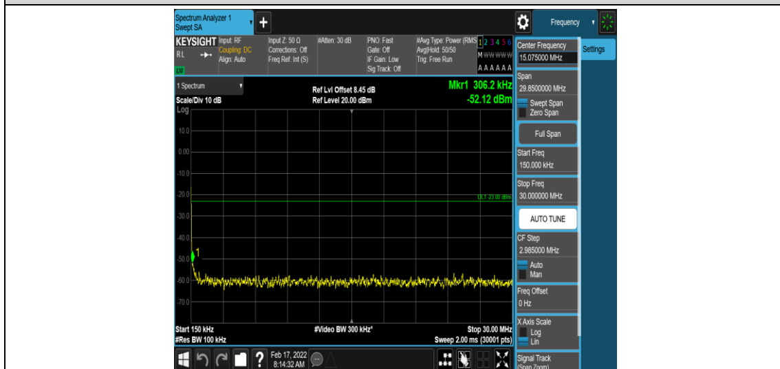
Band26-3MHz-QPSK-26740-1-0-Low-0.15-30--52.12-PASS
