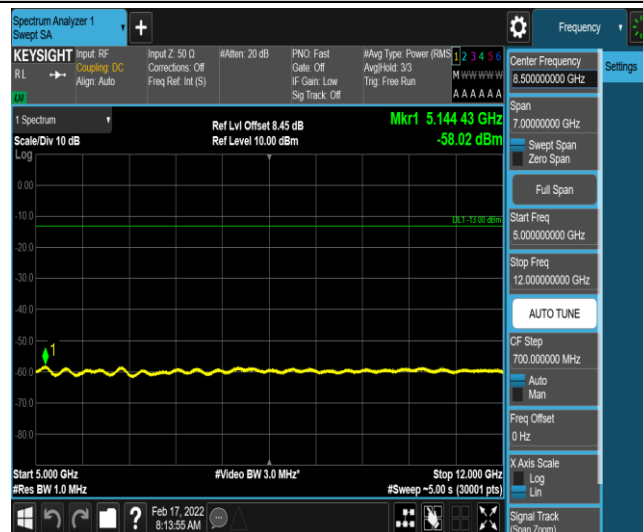
Band26-3MHz-16QAM-26705-1-0-Low-5000-12000--58.02-PASS
