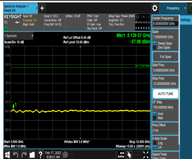
Band26-1.4MHz-16QAM-26783-1-0-High-5000-12000--57.98-PASS
