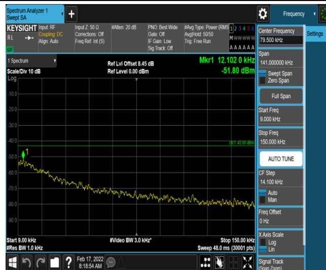
Band26-3MHz-16QAM-26775-1-0-High-0.009-0.15--51.8-PASS
