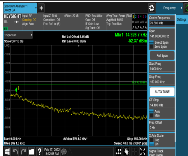
Band26-3MHz-16QAM-26705-1-0-Low-0.009-0.15--52.37-PASS
