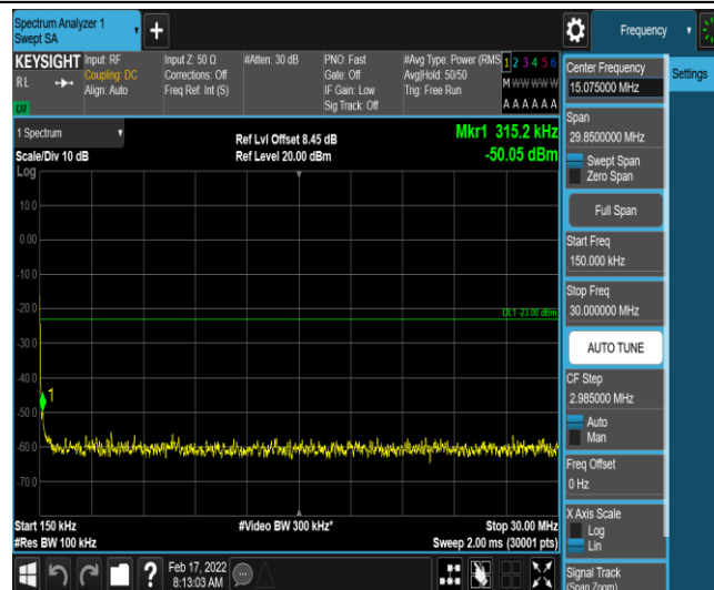
Band26-3MHz-16QAM-26705-1-0-Low-0.15-30--50.05-PASS
