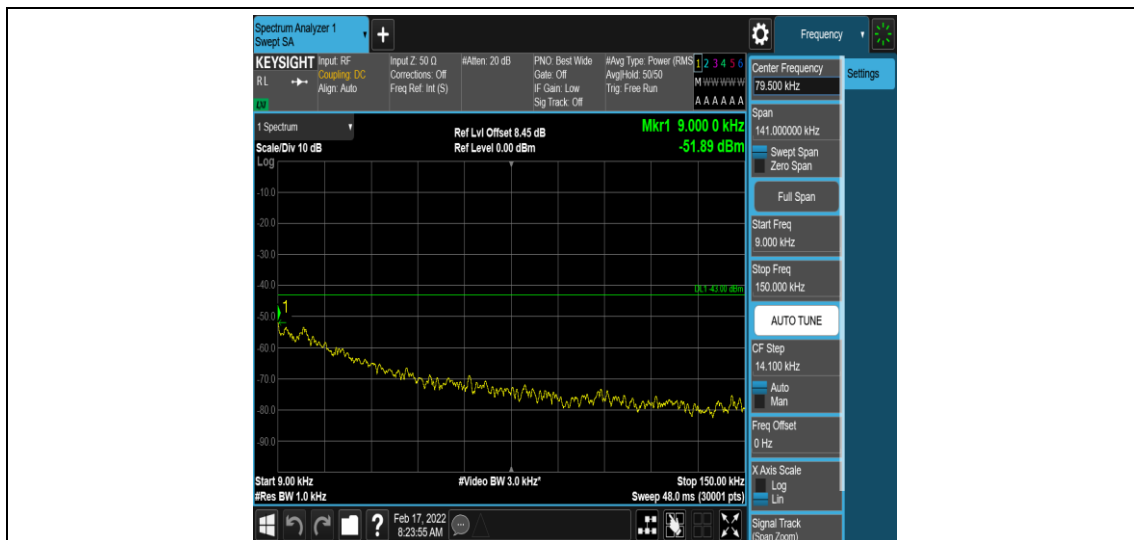
Band26-5MHz-QPSK-26715-1-0-Low-0.009-0.15--51.89-PASS
