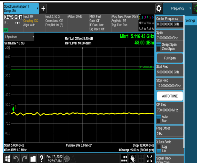
Band26-5MHz-QPSK-26740-1-0-Low-5000-12000--58-PASS
