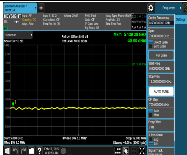
Band26-3MHz-16QAM-26775-1-0-High-5000-12000--58-PASS
