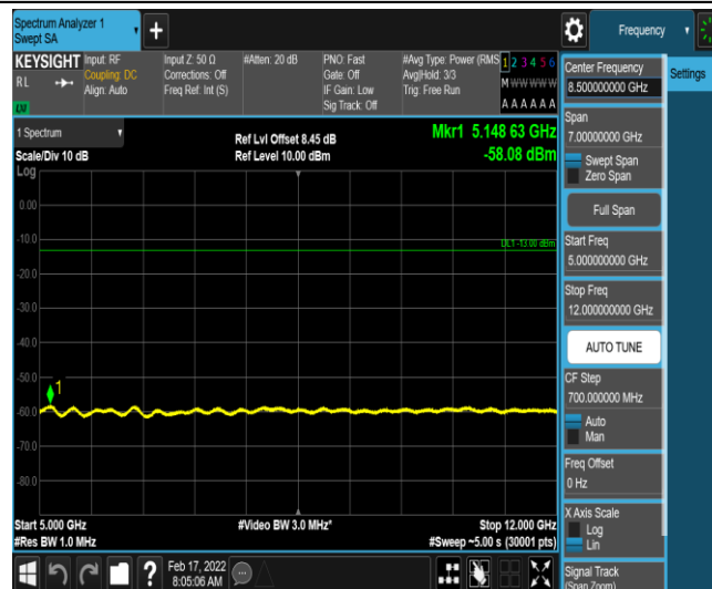
Band26-1.4MHz-16QAM-26740-1-0-Low-5000-12000--58.08-PASS
