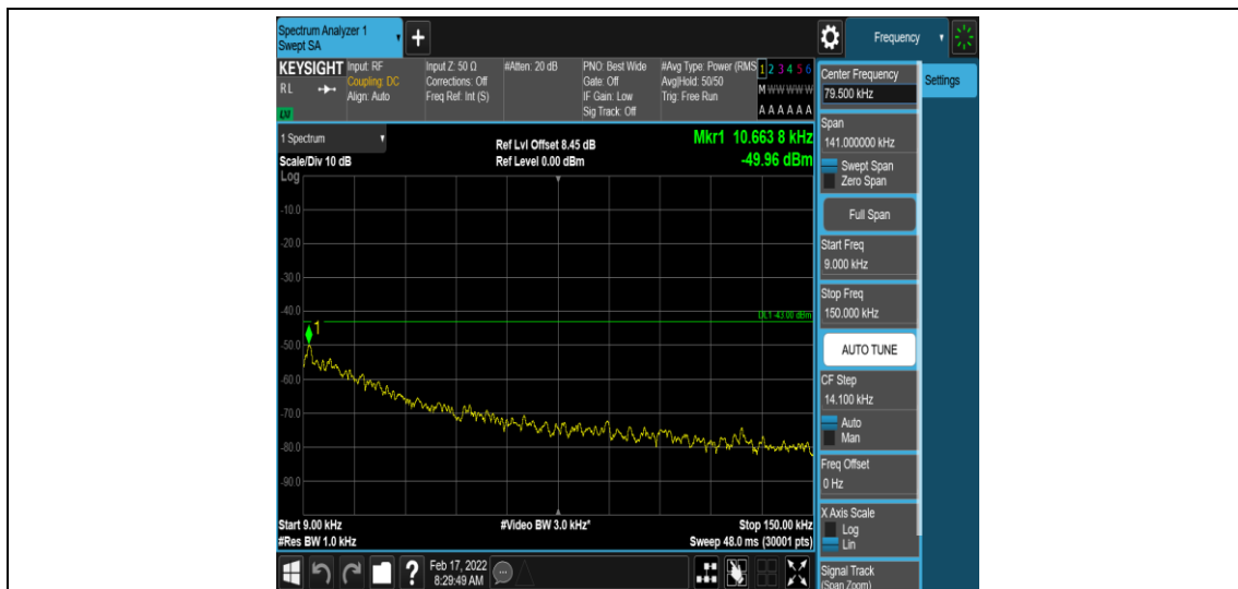
Band26-5MHz-QPSK-26765-1-0-High-0.009-0.15--49.96-PASS
