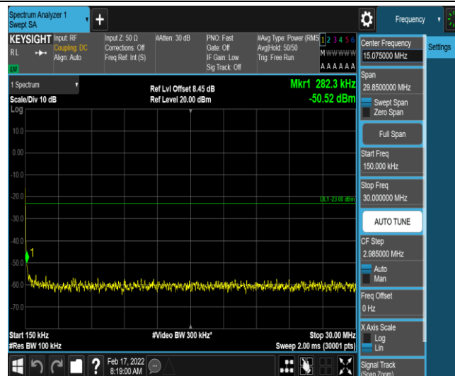
Band26-3MHz-16QAM-26775-1-0-High-0.15-30--50.52-PASS
