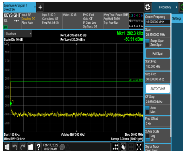
Band26-1.4MHz-16QAM-26783-1-0-High-0.15-30--50.91-PASS
