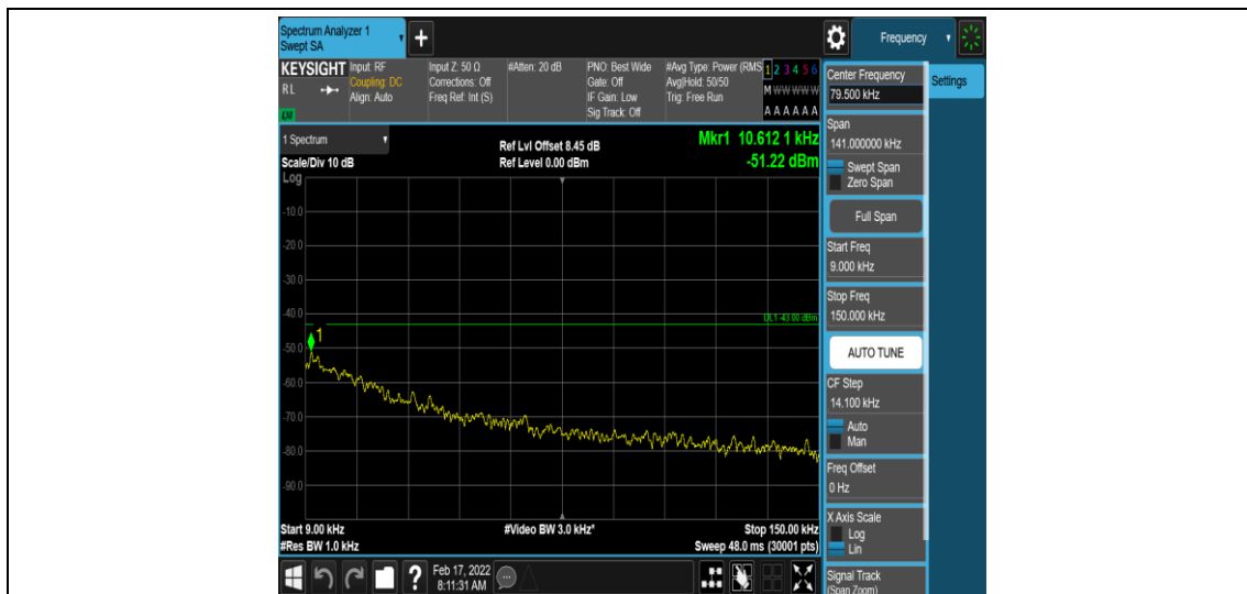
Band26-3MHz-QPSK-26705-1-0-Low-0.009-0.15--51.22-PASS
