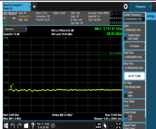
Band26-3MHz-QPSK-26775-1-0-High-5000-12000--58-PASS
