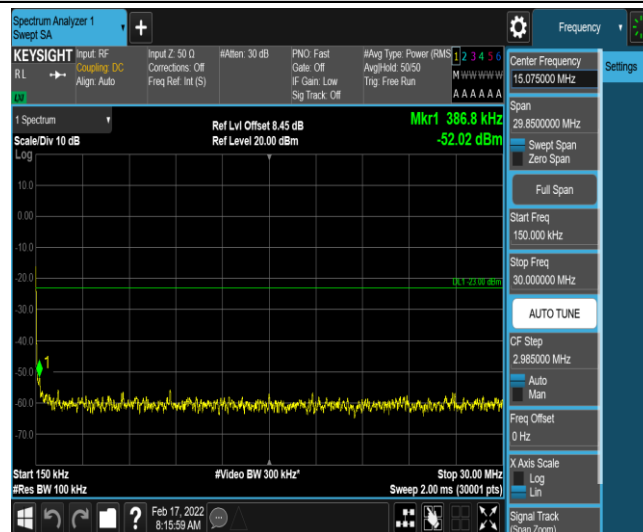
Band26-3MHz-16QAM-26740-1-0-Low-0.15-30--52.02-PASS
