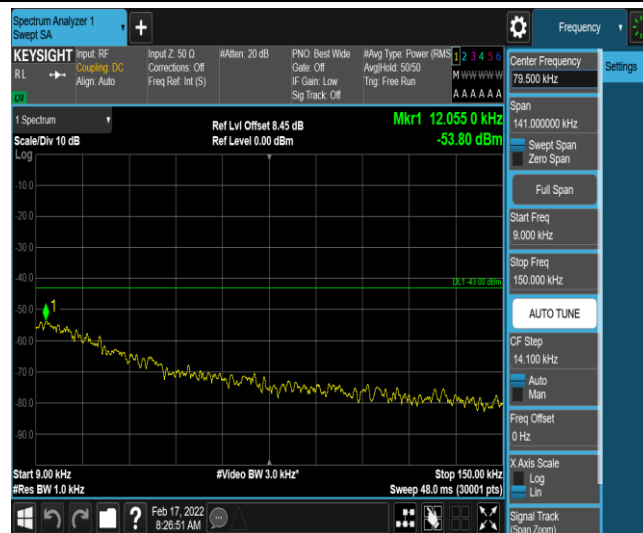
Band26-5MHz-QPSK-26740-1-0-Low-0.009-0.15--53.8-PASS
