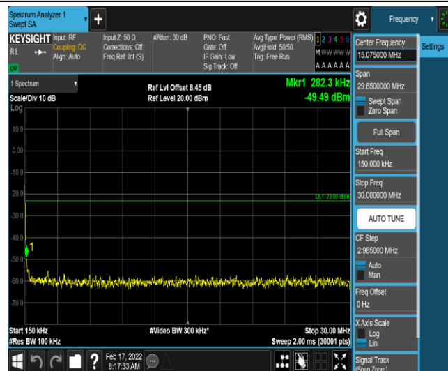
Band26-3MHz-QPSK-26775-1-0-High-0.15-30--49.49-PASS
