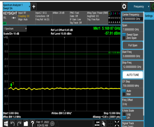
Band26-5MHz-QPSK-26715-1-0-Low-5000-12000--57.91-PASS
