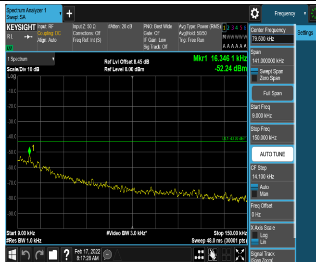
Band26-3MHz-QPSK-26775-1-0-High-0.009-0.15--52.24-PASS
