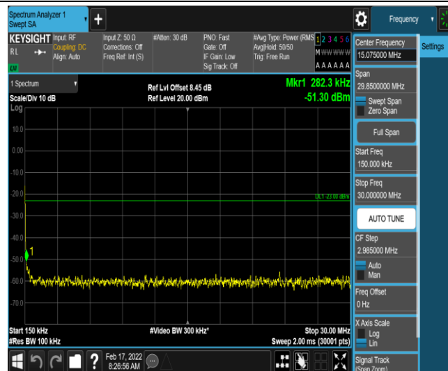
Band26-5MHz-QPSK-26740-1-0-Low-0.15-30--51.3-PASS
