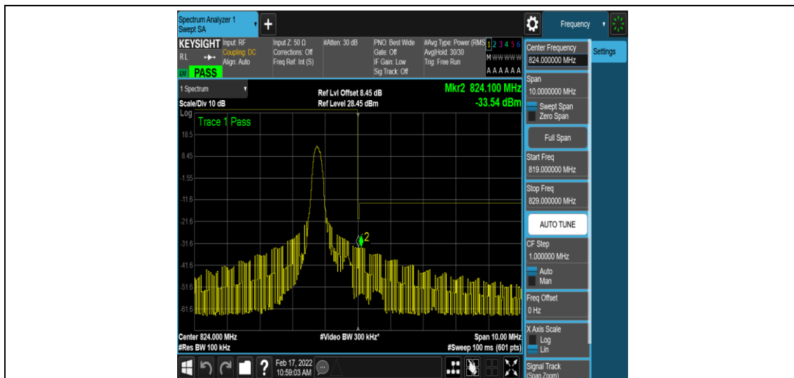
Band26-5MHz-QPSK-26765-1-0-High--33.74,-33.54-PASS
