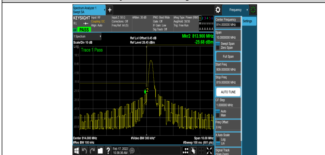
Band26-5MHz-16QAM-26715-1-0-Low--24.48,-25.68-PASS
