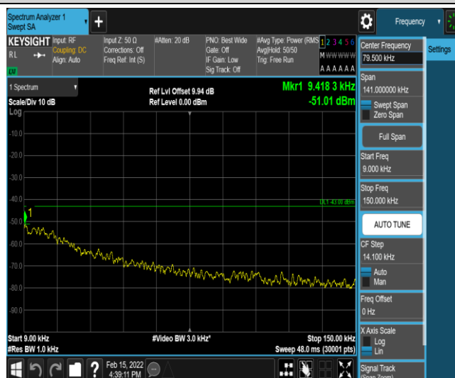
Band25-15MHz-16QAM-26615-1-0-High-0.009-0.15--51.01-PASS
