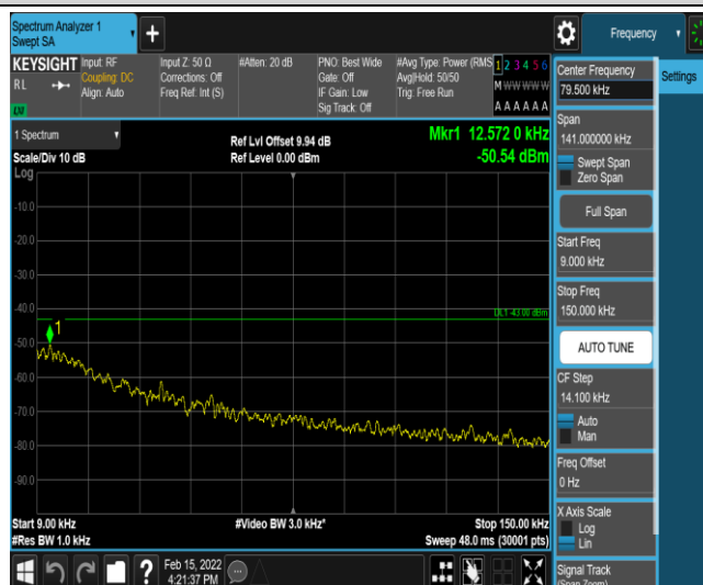
Band25-10MHz-16QAM-26640-1-0-High-0.009-0.15--50.54-PASS
