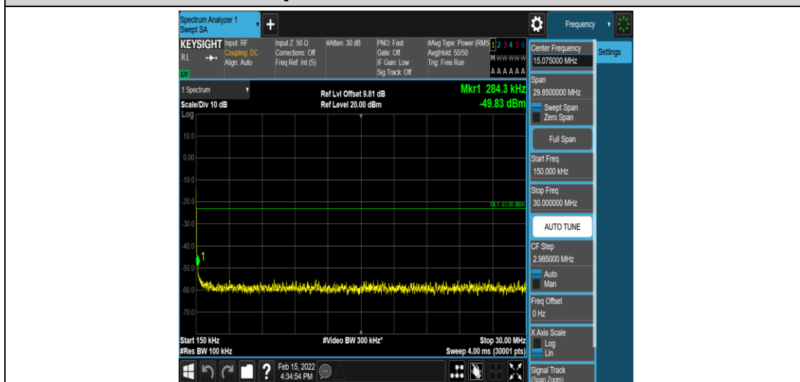
Band25-15MHz-QPSK-26365-1-0-Low-0.15-30--49.83-PASS
