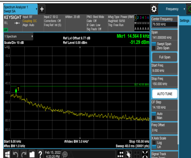
Band25-15MHz-16QAM-26115-1-0-Low-0.009-0.15--51.29-PASS
