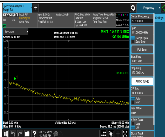
Band25-15MHz-QPSK-26615-1-0-High-0.009-0.15--51.04-PASS
