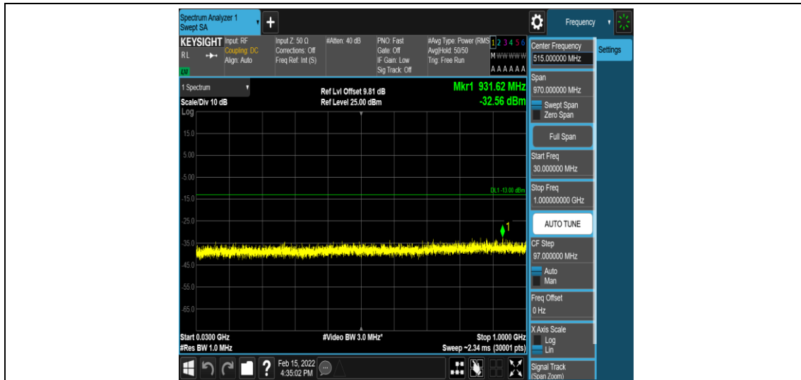
Band25-15MHz-QPSK-26365-1-0-Low-30-1000--32.56-PASS
