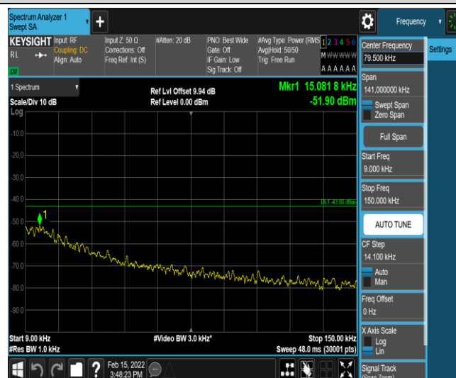
Band25-3MHz-16QAM-26675-1-0-High-0.009-0.15--51.9-PASS
