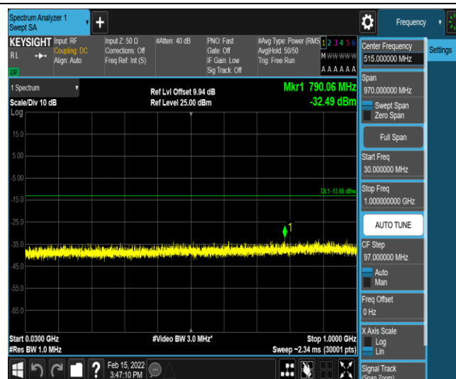
Band25-3MHz-QPSK-26675-1-0-High-30-1000--32.49-PASS
