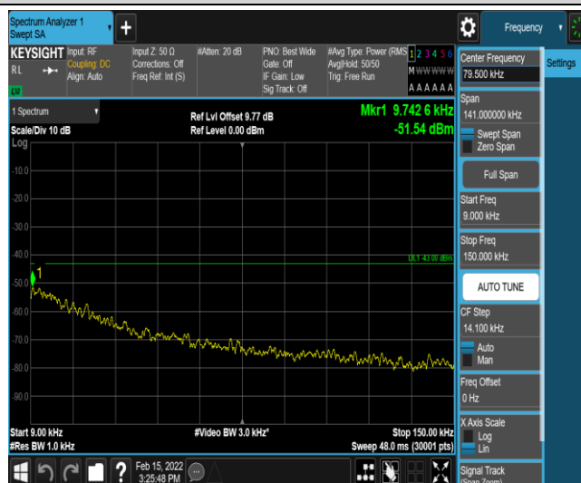
Band25-1.4MHz-16QAM-26047-1-0-Low-0.009-0.15--51.54-PASS
