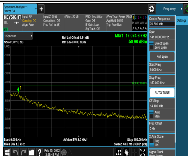
Band25-1.4MHz-16QAM-26365-1-0-Low-0.009-0.15--50.96-PASS
