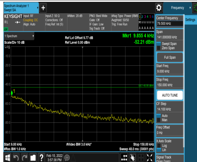
Band25-5MHz-QPSK-26065-1-0-Low-0.009-0.15--52.21-PASS
