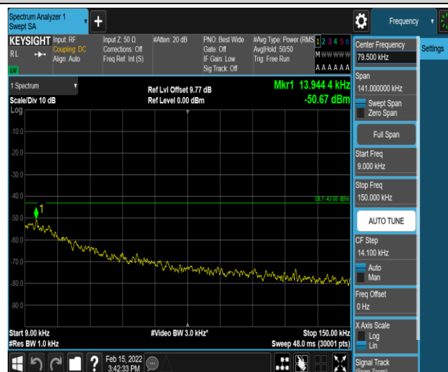
Band25-3MHz-16QAM-26055-1-0-Low-0.009-0.15--50.68-PASS
