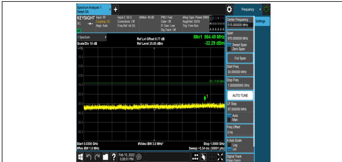
Band25-1.4MHz-16QAM-26047-1-0-Low-30-1000--32.29-PASS
