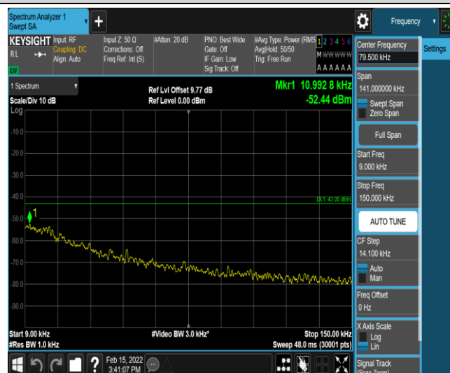
Band25-3MHz-QPSK-26055-1-0-Low-0.009-0.15--52.44-PASS
