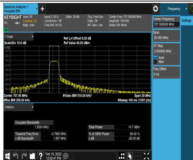
Band12-10MHz-16QAM-23095-6-0-Low-1.3024-1.567-PASS
