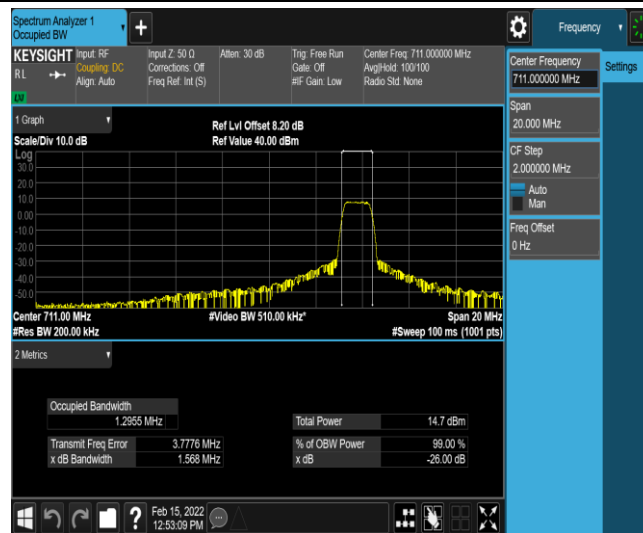
Band12-10MHz-QPSK-23130-6-0-High-1.2955-1.568-PASS
