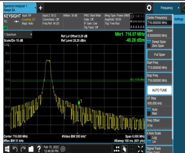
Band12-3MHz-QPSK-23165-1-0-High--40.28-PASS
