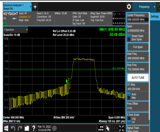
Band12-3MHz-QPSK-23025-6-0-Low--30.49-PASS
