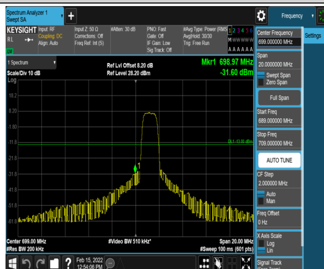
Band12-10MHz-16QAM-23060-6-0-Low--31.60-PASS
