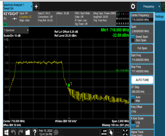
Band12-1.4MHz-16QAM-23173-6-0-High--32.69-PASS
