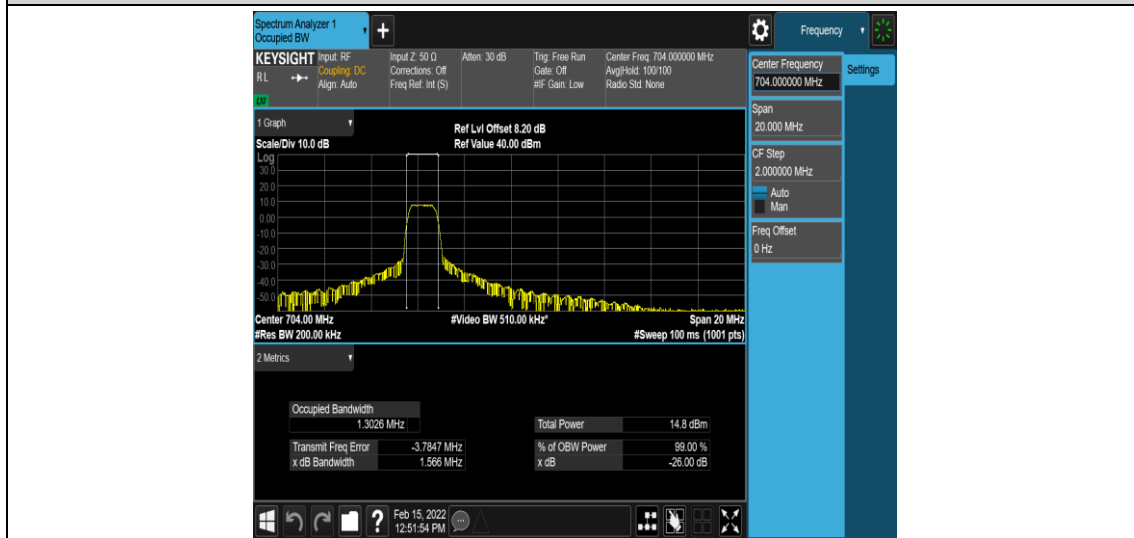
Band12-10MHz-QPSK-23060-6-0-Low-1.3026-1.566-PASS
