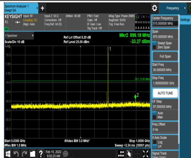
Band12-1.4MHz-QPSK-23095-1-0-Low-30-1000--33.27-PASS
