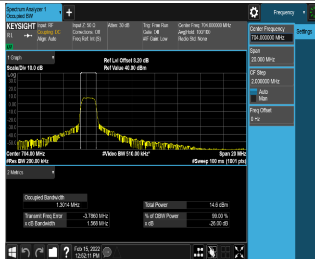
Band12-10MHz-16QAM-23060-6-0-Low-1.3014-1.568-PASS
