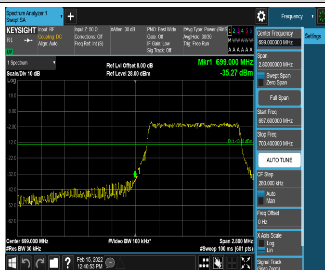
Band12-1.4MHz-16QAM-23017-6-0-Low--35.27-PASS
