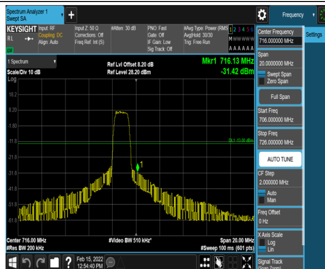
Band12-10MHz-QPSK-23130-6-0-High--31.42-PASS
