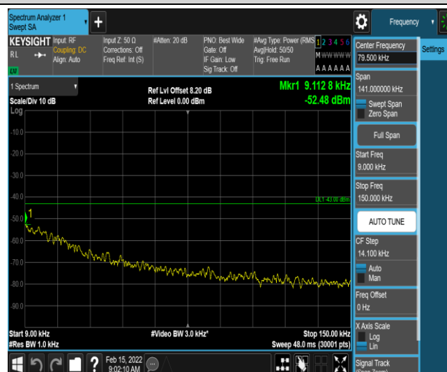
Band12-1.4MHz-QPSK-23095-1-0-Low-0.009-0.15--52.48-PASS
