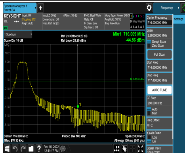
Band12-1.4MHz-16QAM-23173-1-0-High--44.56-PASS
