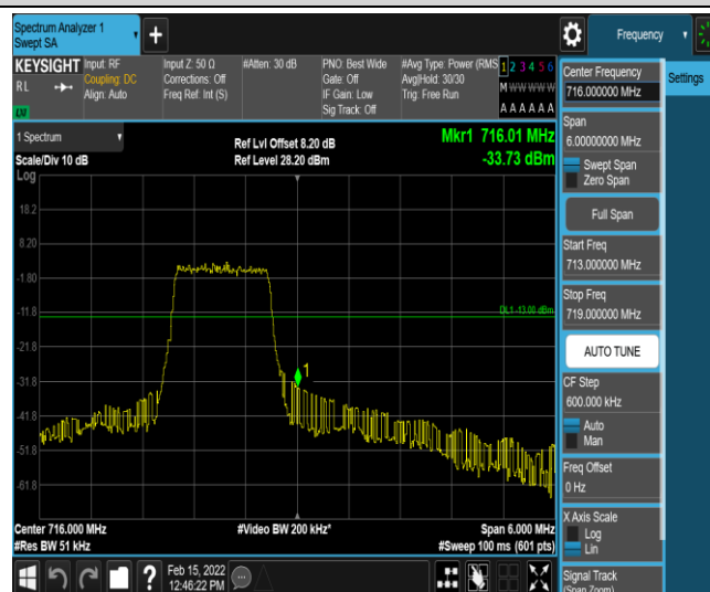
Band12-3MHz-QPSK-23165-6-0-High--33.73-PASS
