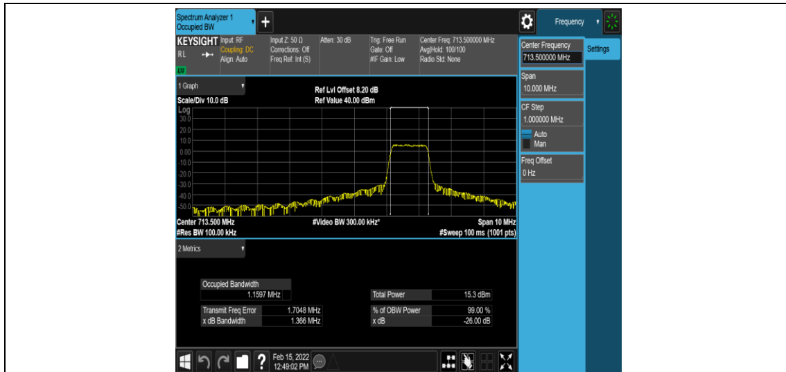
Band12-5MHz-16QAM-23155-6-0-High-1.1597-1.366-PASS
