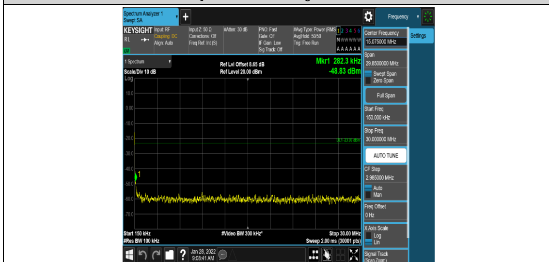
Band4-20MHz-16QAM-20300-1-0-High-0.15-30--48.83-PASS
