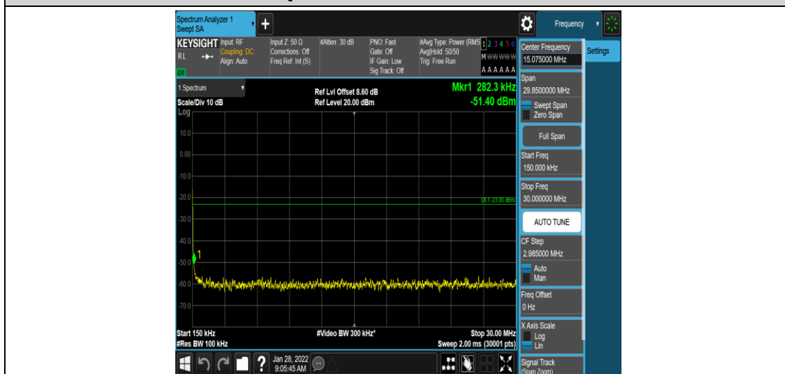
Band4-20MHz-16QAM-20175-1-0-Low-0.15-30--51.4-PASS
