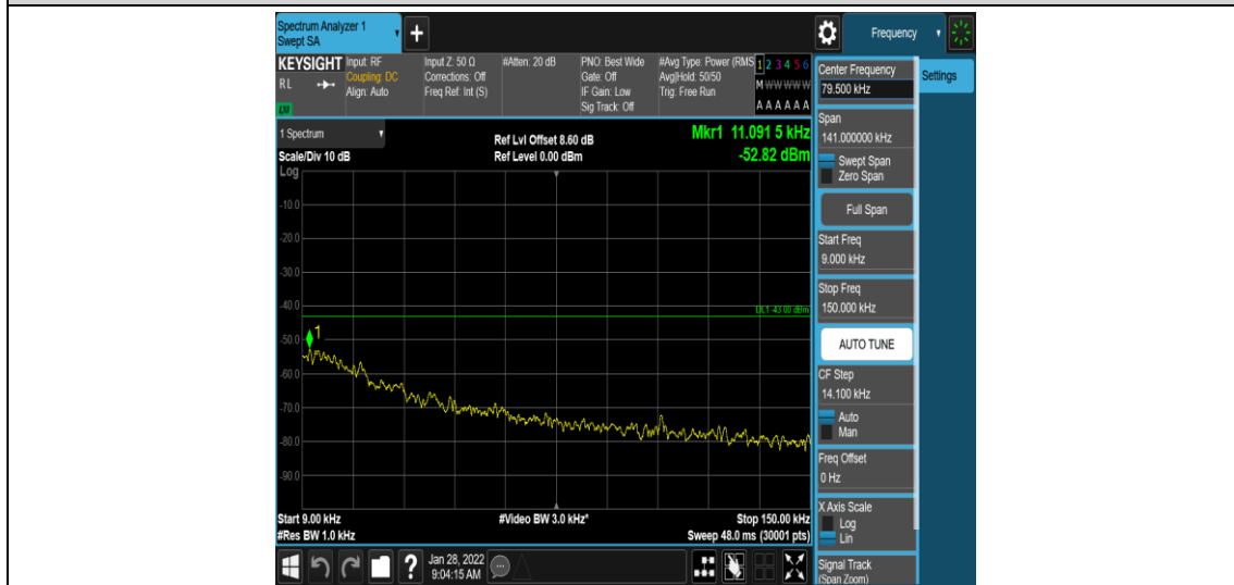
Band4-20MHz-QPSK-20175-1-0-Low-0.009-0.15--52.82-PASS
