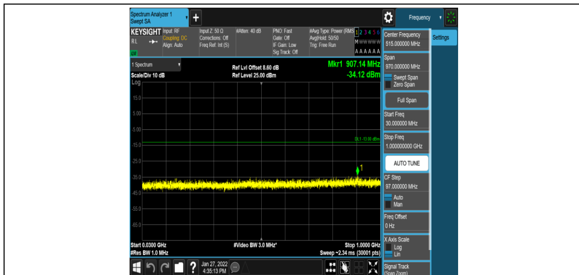
Band4-15MHz-QPSK-20025-1-0-Low-30-1000--34.12-PASS
