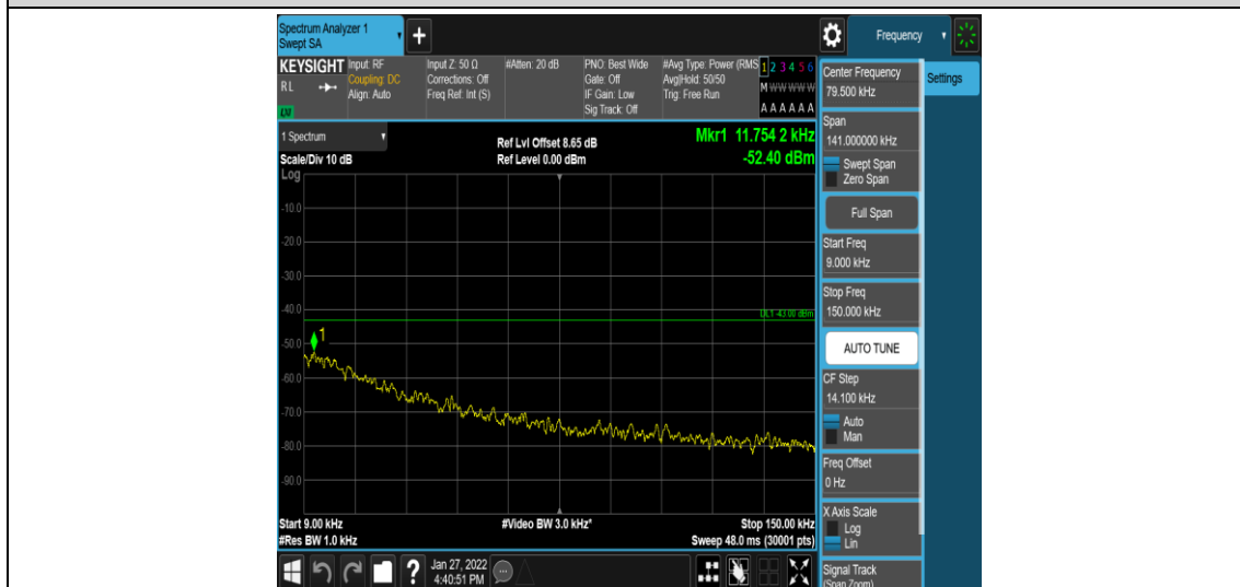
Band4-15MHz-QPSK-20325-1-0-High-0.009-0.15--52.4-PASS
