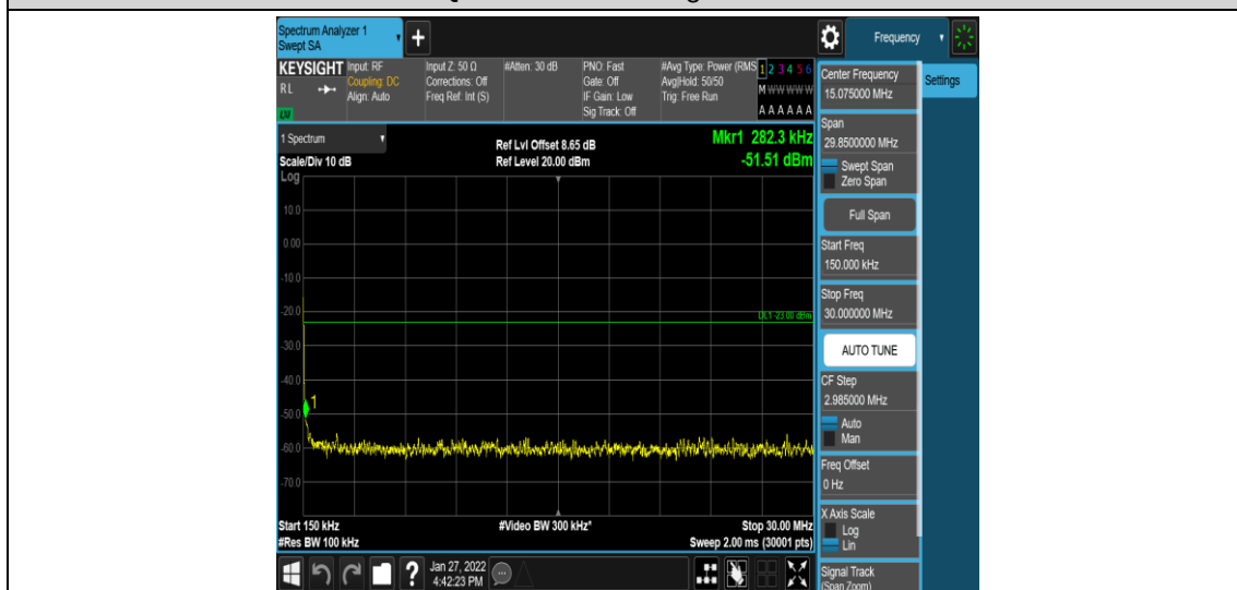
Band4-15MHz-16QAM-20325-1-0-High-0.15-30--51.51-PASS
