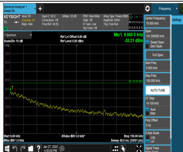
Band4-15MHz-QPSK-20025-1-0-Low-0.15--53.21-PASS
