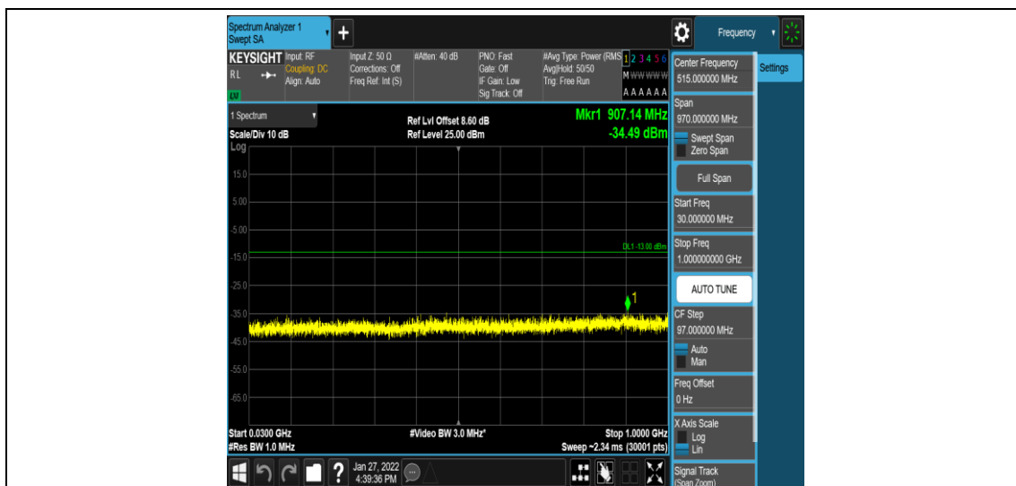
Band4-15MHz-16QAM-20175-1-0-Low-30-1000--34.49-PASS
