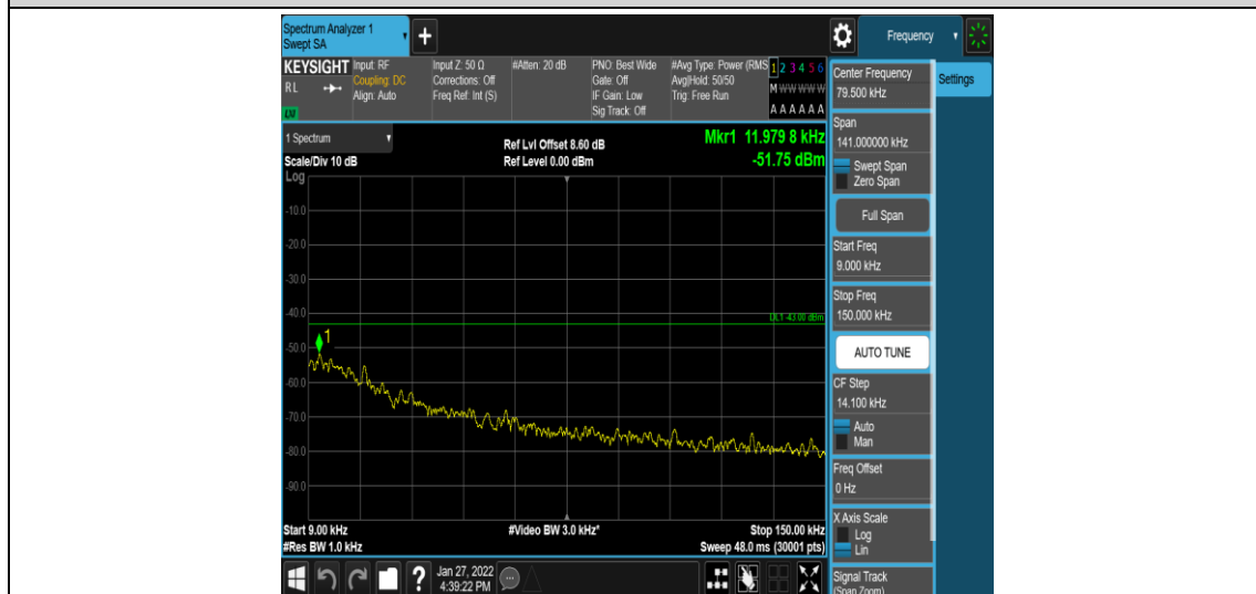
Band4-15MHz-16QAM-20175-1-0-Low-0.009-0.15--51.75-PASS
