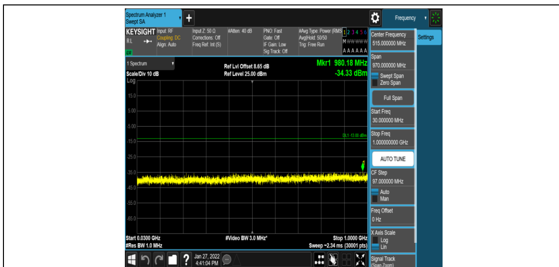
Band4-15MHz-QPSK-20325-1-0-High-30-1000--34.33-PASS
