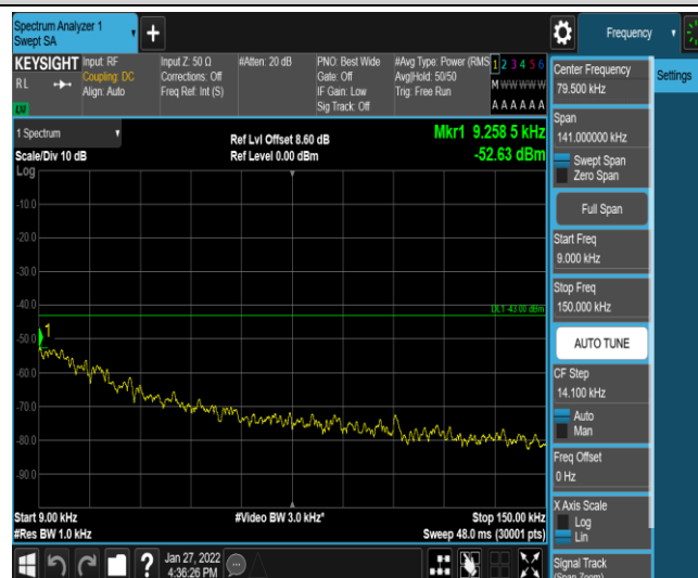
Band4-15MHz-16QAM-20025-1-0-Low-0.009-0.15--52.63-PASS
