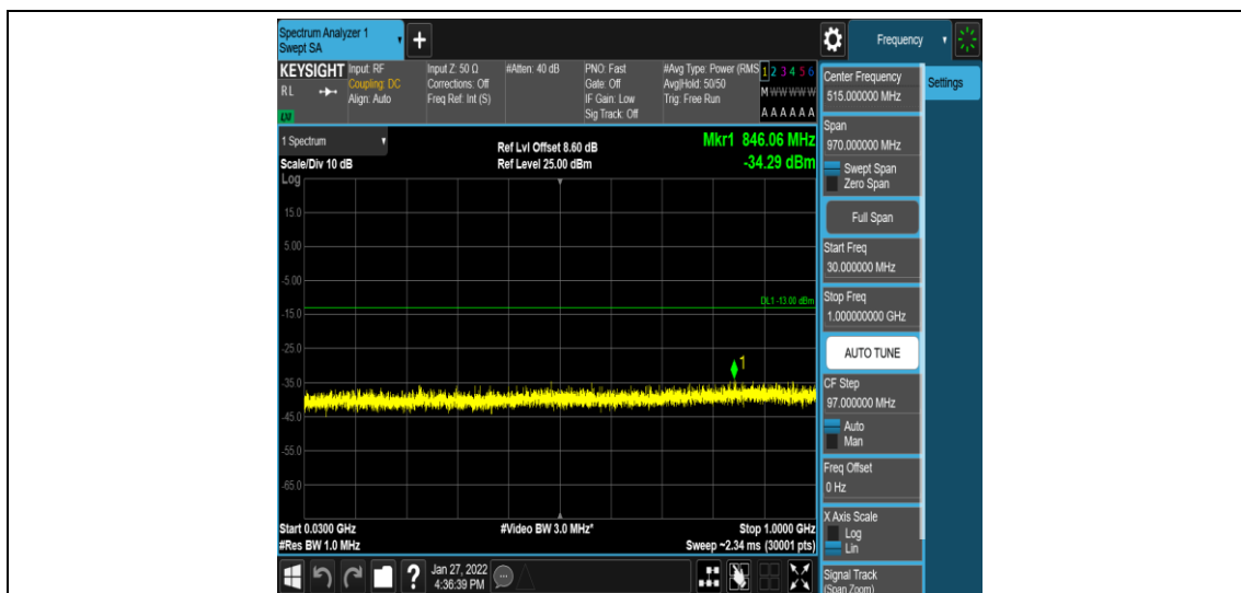
Band4-15MHz-16QAM-20025-1-0-Low-30-1000--34.29-PASS
