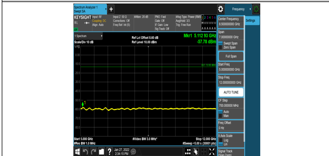
Band4-5MHz-16QAM-20175-1-0-Low-5000-12000--57.78-PASS
