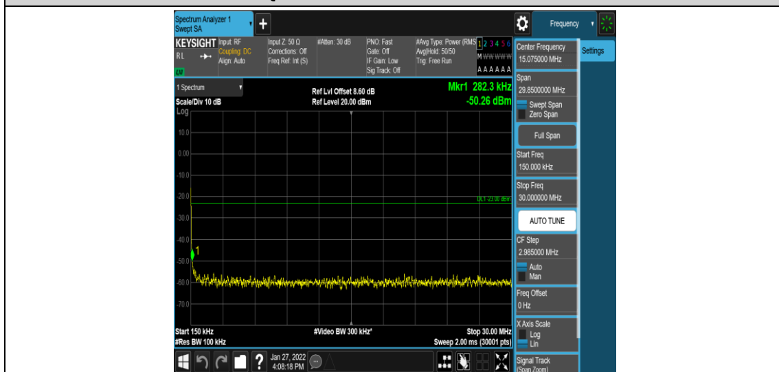
Band4-10MHz-QPSK-20000-1-0-Low-0.15-30--50.26-PASS
