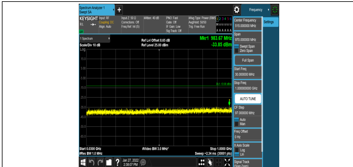
Band4-5MHz-16QAM-20375-1-0-High-30-1000--33.85-PASS
