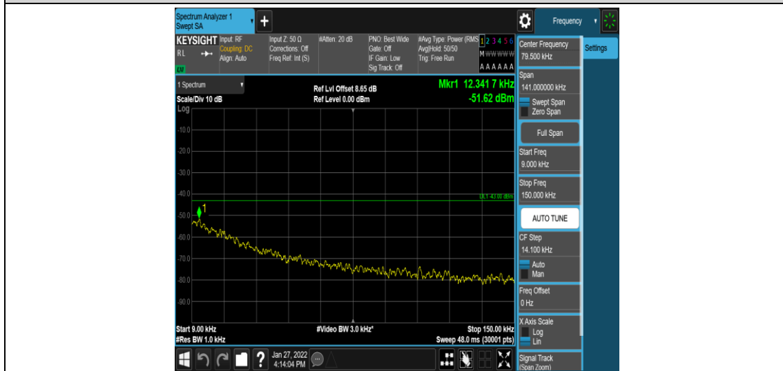
Band4-10MHz-QPSK-20350-1-0-High-0.009-0.15--51.62-PASS
