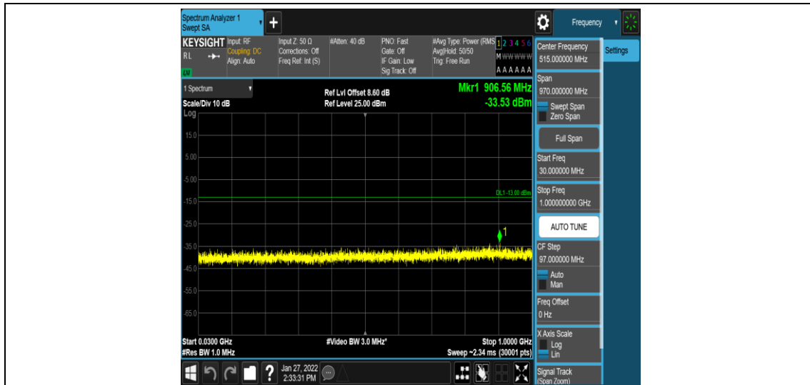
Band4-5MHz-16QAM-20175-1-0-Low-30-1000--33.53-PASS
