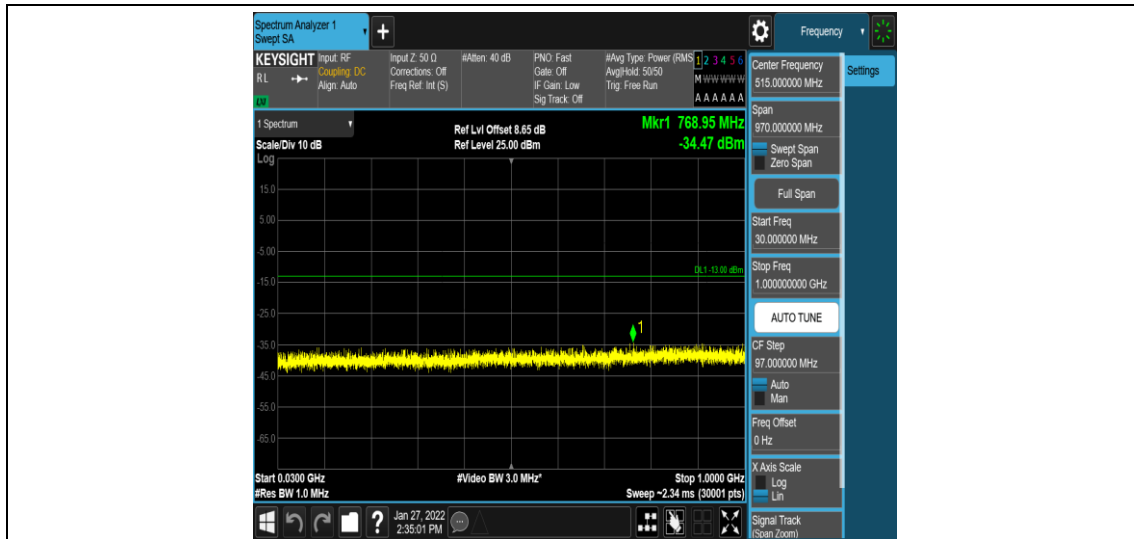
Band4-5MHz-QPSK-20375-1-0-High-30-1000--34.47-PASS
