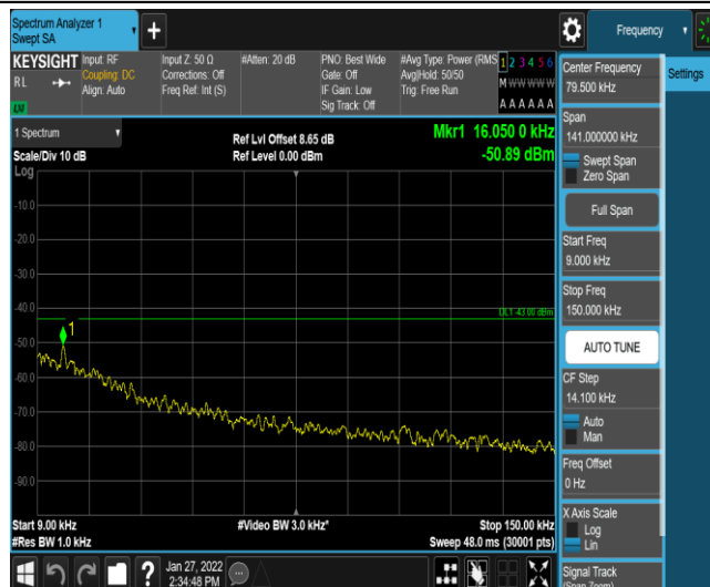
Band4-5MHz-QPSK-20375-1-0-High-0.009-0.15--50.9-PASS
