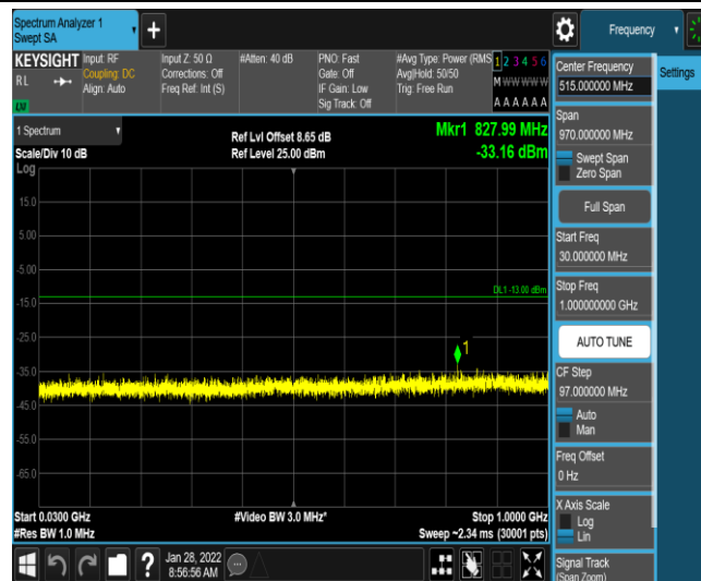
Band4-3MHz-16QAM-20385-1-0-High-30-1000--33.16-PASS
