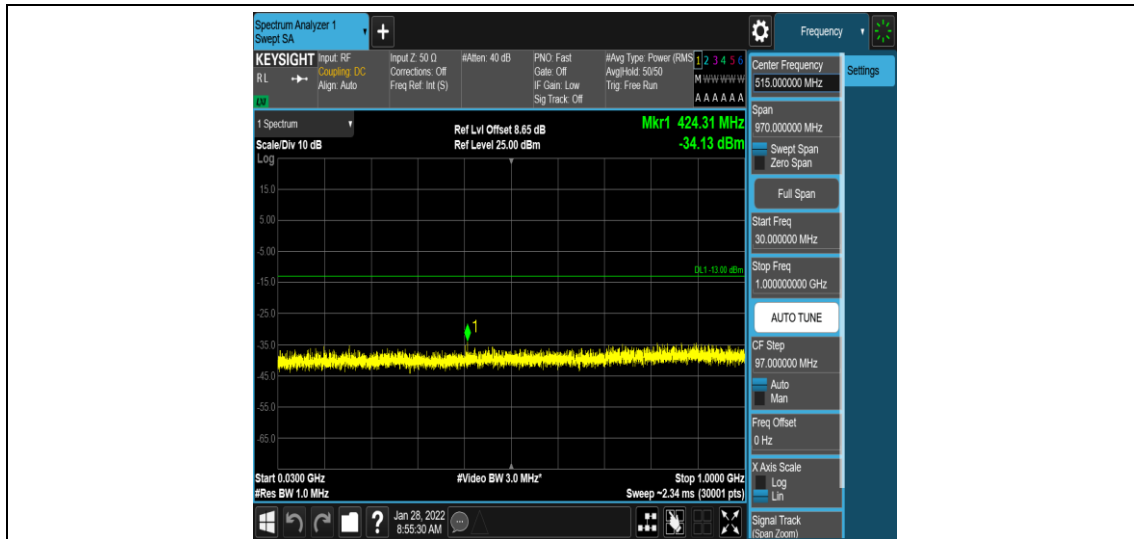
Band4-3MHz-QPSK-20385-1-0-High-30-1000--34.13-PASS
