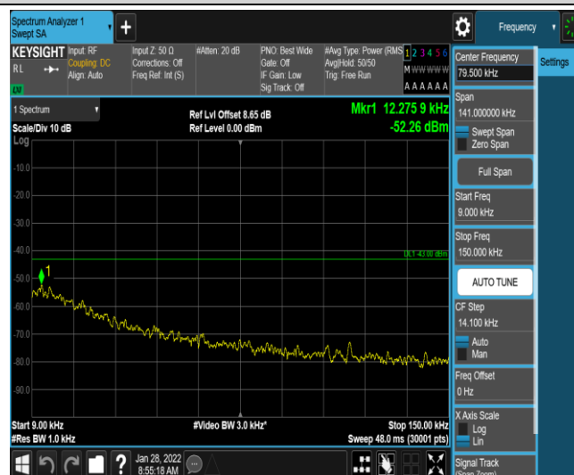
Band4-3MHz-QPSK-20385-1-0-High-0.009-0.15--52.26-PASS
