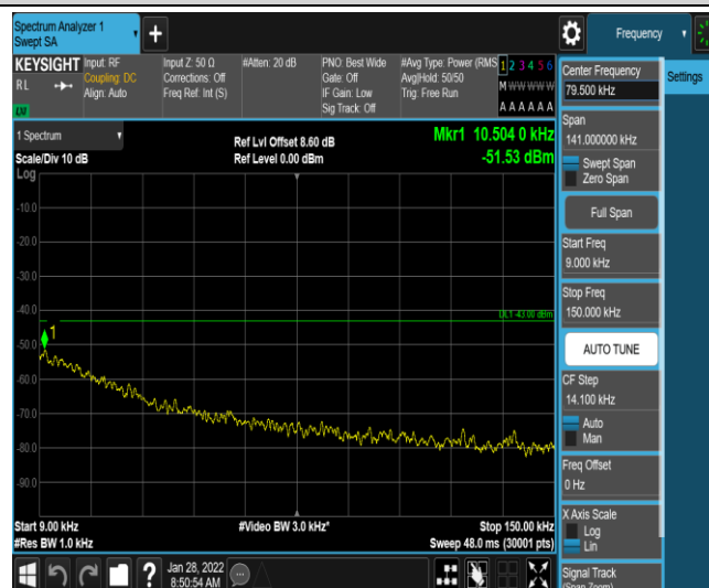
Band4-3MHz-16QAM-19965-1-0-Low-0.009-0.15--51.53-PASS
