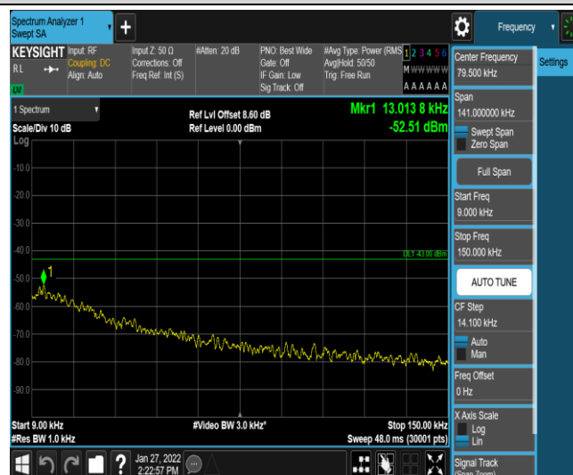
Band4-5MHz-QPSK-19975-1-0-Low-0.009-0.15--52.51-PASS
