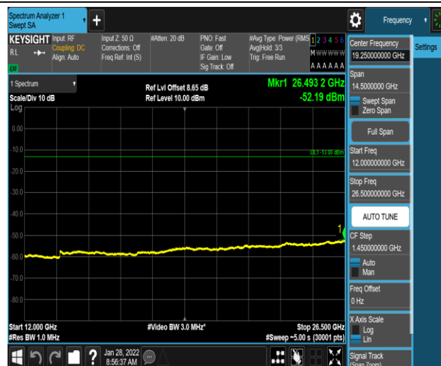
Band4-3MHz-QPSK-20385-1-0-High-12000-26500--52.19-PASS
