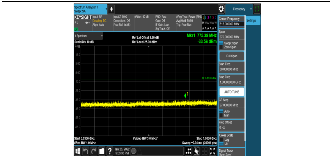
Band4-1.4MHz-16QAM-20175-1-0-Low-30-1000--33.56-PASS
