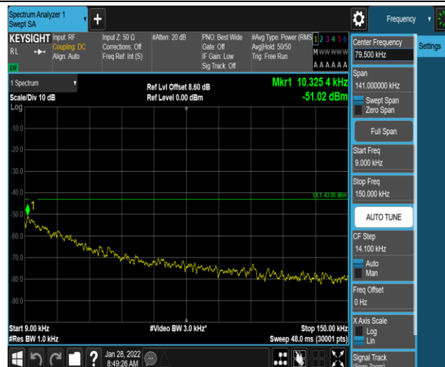
Band4-3MHz-QPSK-19965-1-0-Low-0.009-0.15--51.02-PASS
