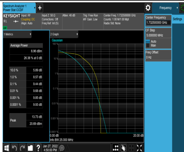
Band4-20MHz-16OAM-20175-6-0-Low-9.44-<=13-PASS
