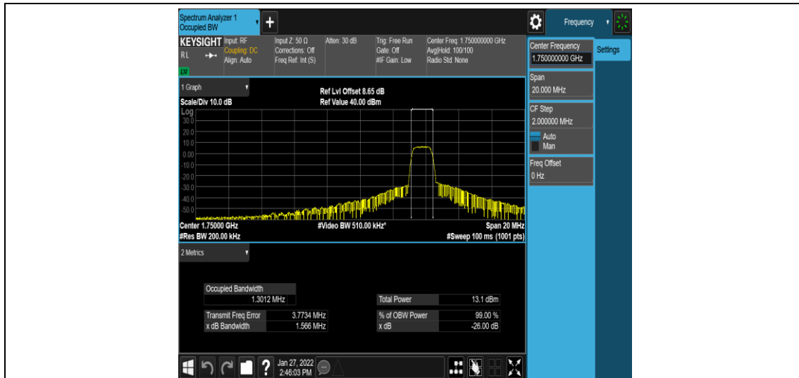
Band4-10MHz-QPSK-20350-6-0-High-1.3012-1.566-PASS
