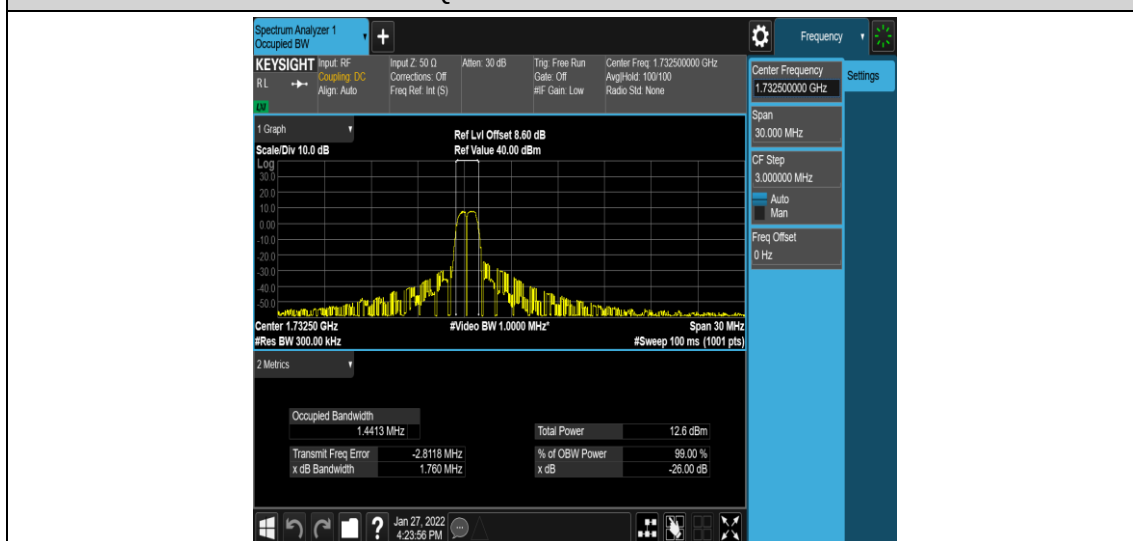
Band4-15MHz-16QAM-20175-6-0-Low-1.4413-1.760-PASS
