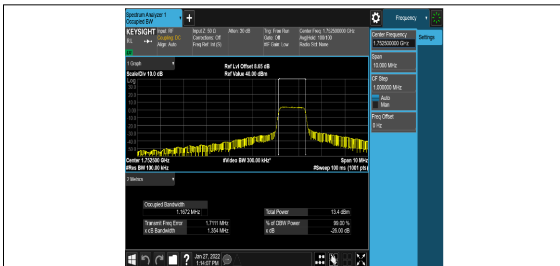
Band4-5MHz-16QAM-20375-6-0-High-1.1672-1.354-PASS
