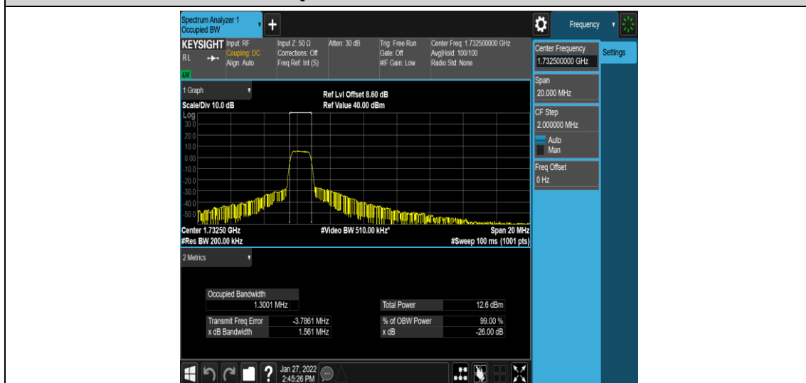
Band4-10MHz-QPSK-20175-6-0-Low-1.3001-1.561-PASS
