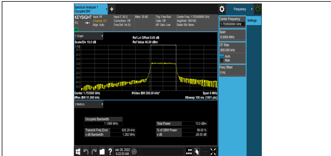
Band4-3MHz-QPSK-20385-6-0-High-1.1088-1.282-PASS
