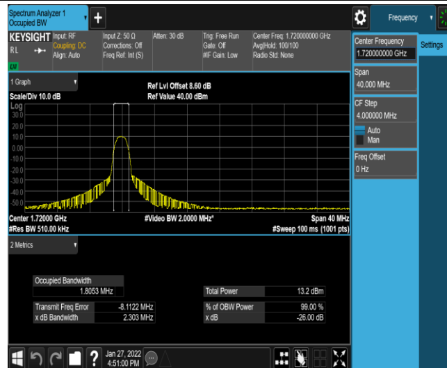
Band4-20MHz-QPSK-20050-6-0-Low-1.8053-2.303-PASS
