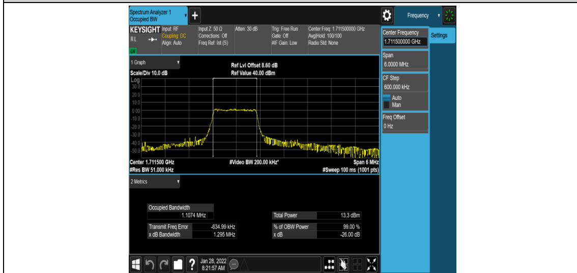
Band4-3MHz-16QAM-19965-6-0-Low-1.1074-1.295-PASS
