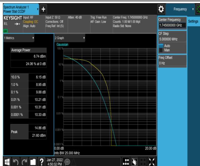
Band4-20MHz-QPSK-20300-6-0-High-9.88-&lt;=13-PASS
