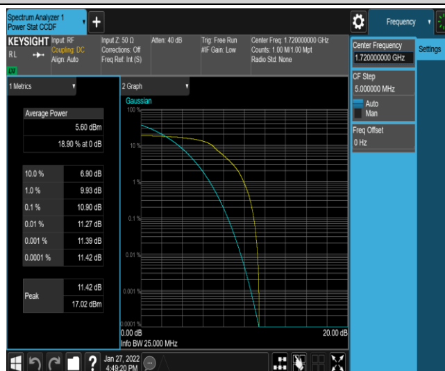
Band4-20MHz-16QAM-20050-6-0-Low-10.90-&lt;=13-PASS
