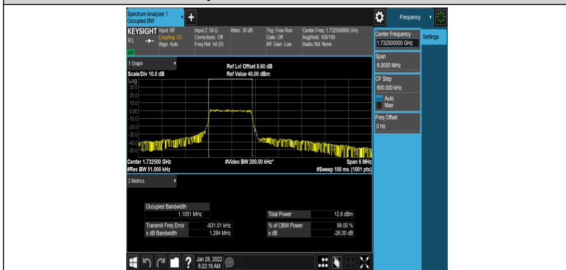
Band4-3MHz-QPSK-20175-6-0-Low-1.1051-1.284-PASS
