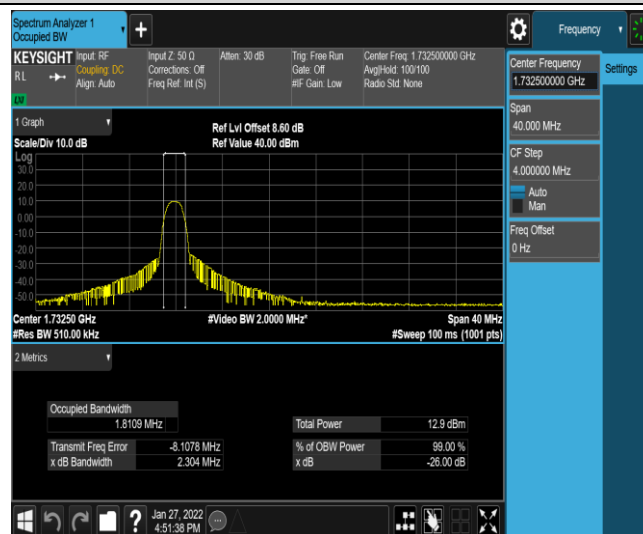
Band4-20MHz-QPSK-20175-6-0-Low-1.8109-2.304-PASS
