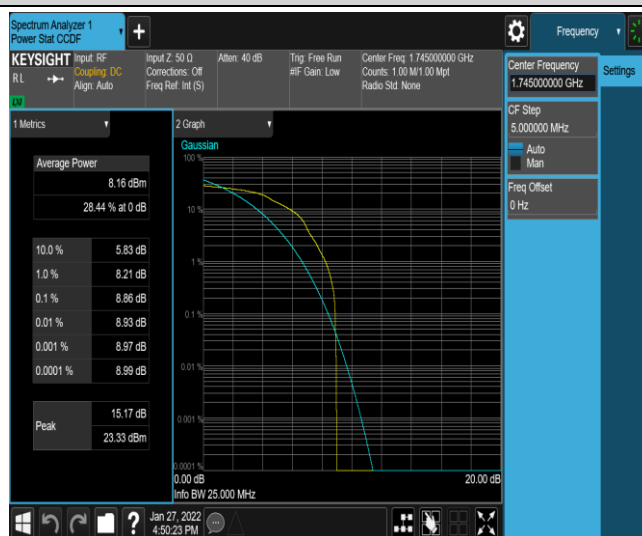
Band4-20MHz-16QAM-20300-1-0-High-8.86-<=13-PASS
