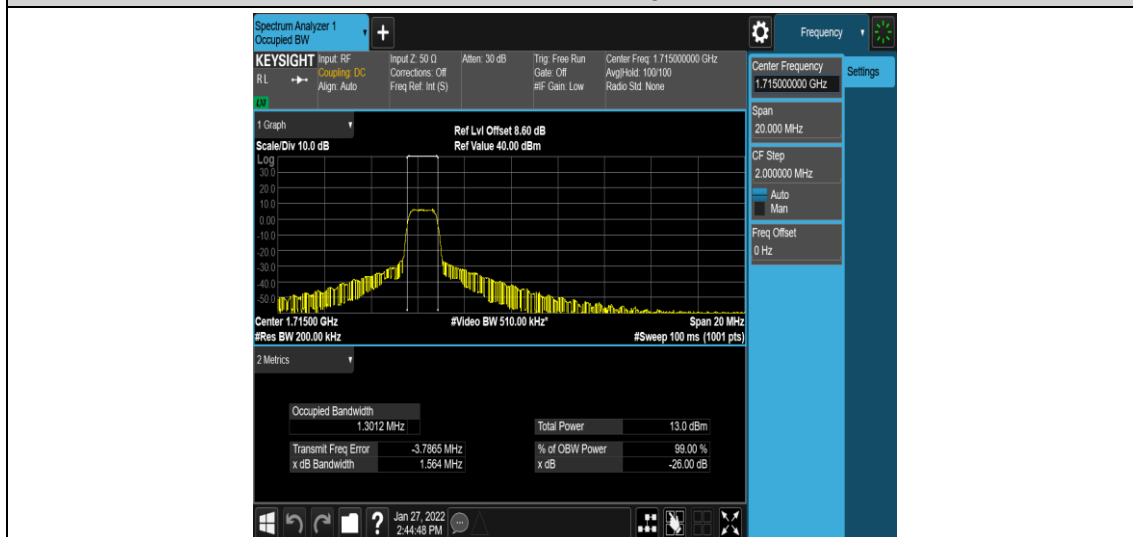
Band4-10MHz-QPSK-20000-6-0-Low-1.3012-1.564-PASS
