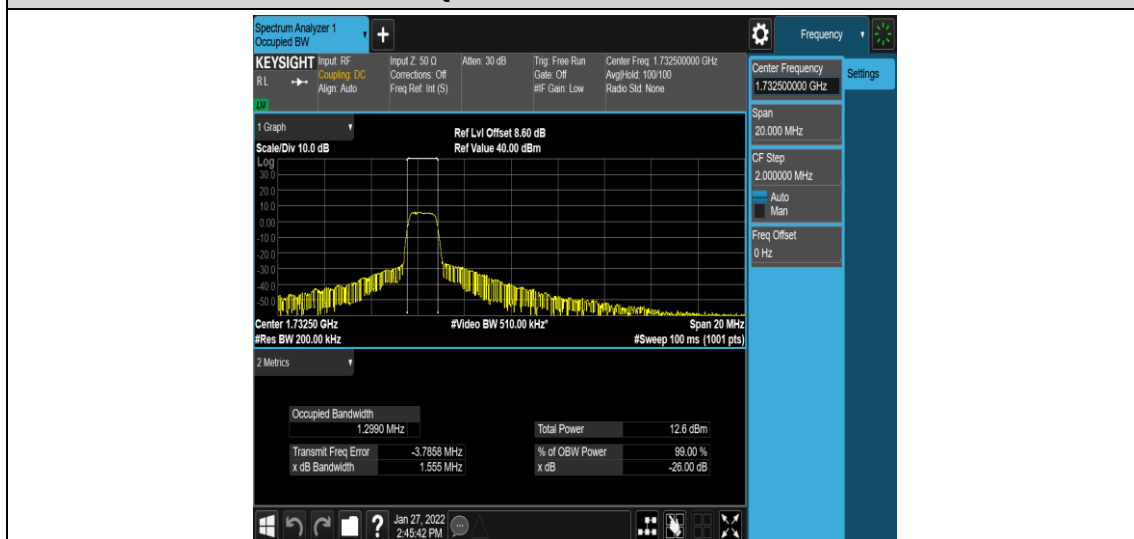
Band4-10MHz-16QAM-20175-6-0-Low-1.2990-1.555-PASS
