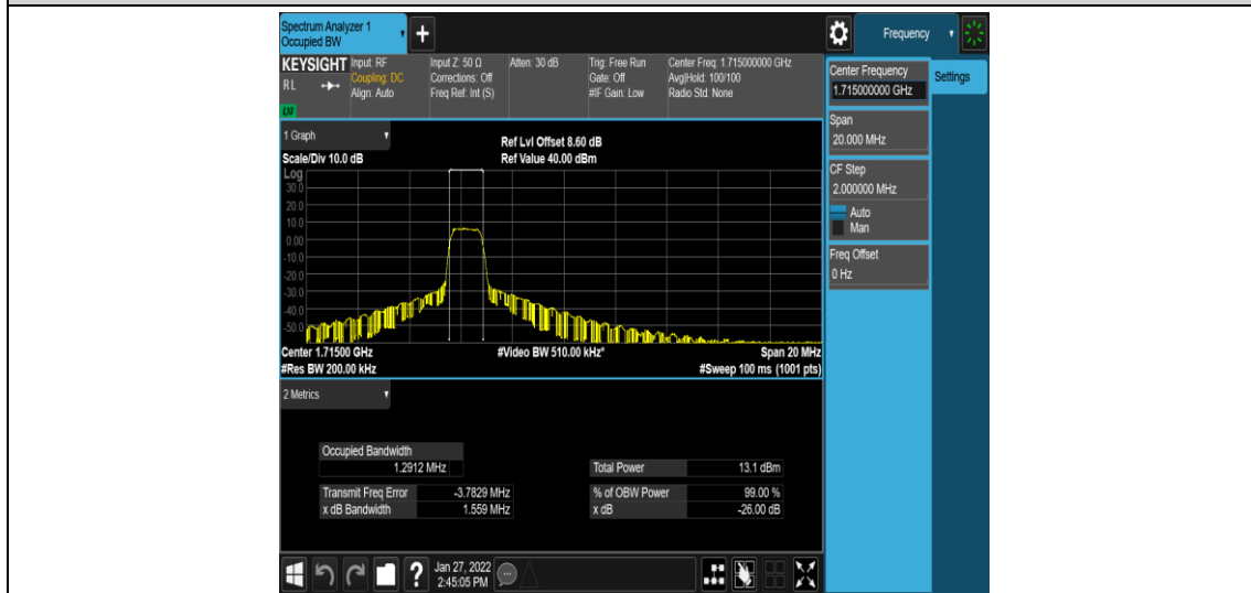
Band4-10MHz-16QAM-20000-6-0-Low-1.2912-1.559-PASS
