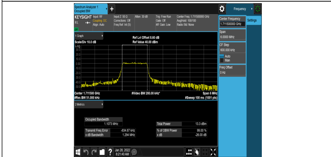
Band4-3MHz-QPSK-19965-6-0-Low-1.1073-1.294-PASS
