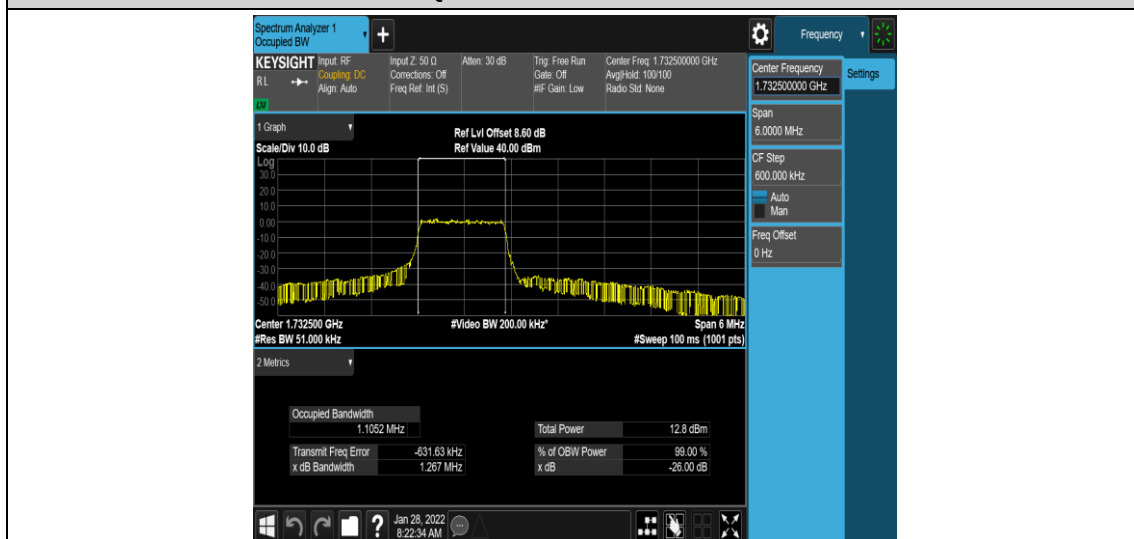
Band4-3MHz-16QAM-20175-6-0-Low-1.1052-1.267-PASS
