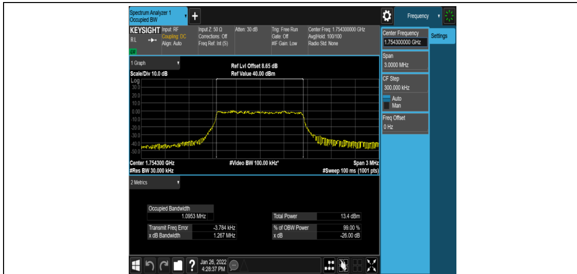
Band4-1.4MHz-16QAM-20393-6-0-High-1.0953-1.267-PASS
