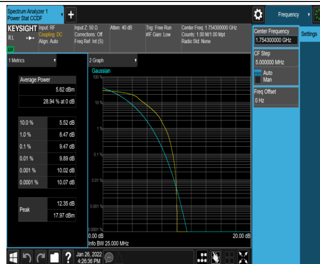
Band4-1.4MHz-16QAM-20393-6-0-High-9.47-&lt;=13-PASS
