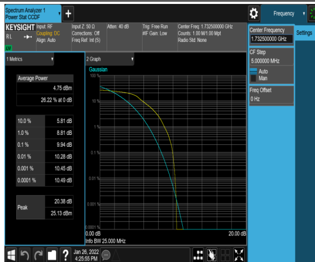
Band4-1.4MHz-16QAM-20175-6-0-Low-9.94-&lt;=13-PASS
