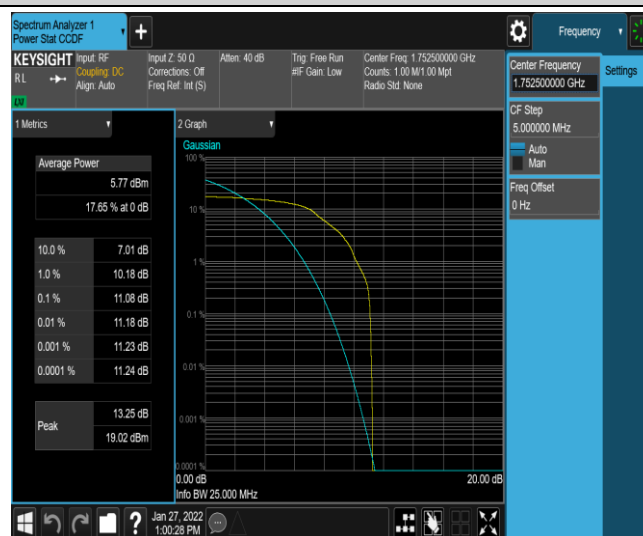
Band4-5MHz-QPSK-20375-1-0-High-11.08-&lt;=13-PASS
