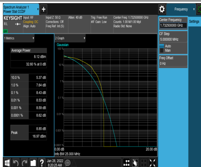
Band4-3MHz-16QAM-20175-1-0-Low-8.43-&lt;=13-PASS
