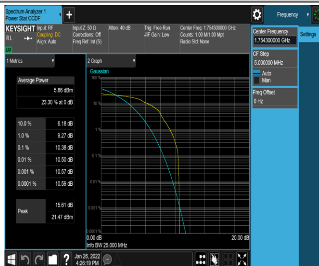
Band4-1.4MHz-16QAM-20393-1-0-High-10.38-&lt;=13-PASS
