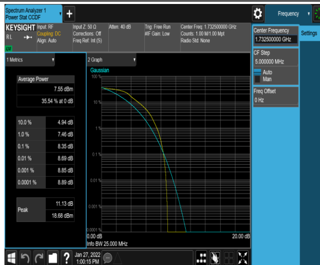
Band4-5MHz-16QAM-20175-6-0-Low-8.35-&lt;=13-PASS
