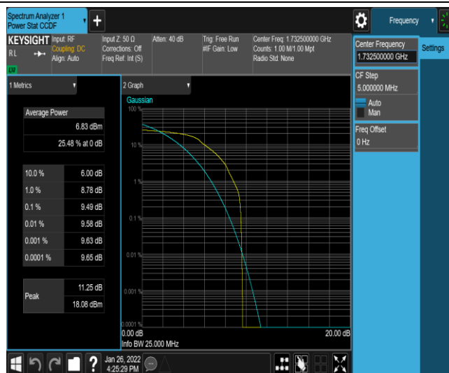
Band4-1.4MHz-QPSK-20175-1-0-Low-9.49-<=13-PASS
