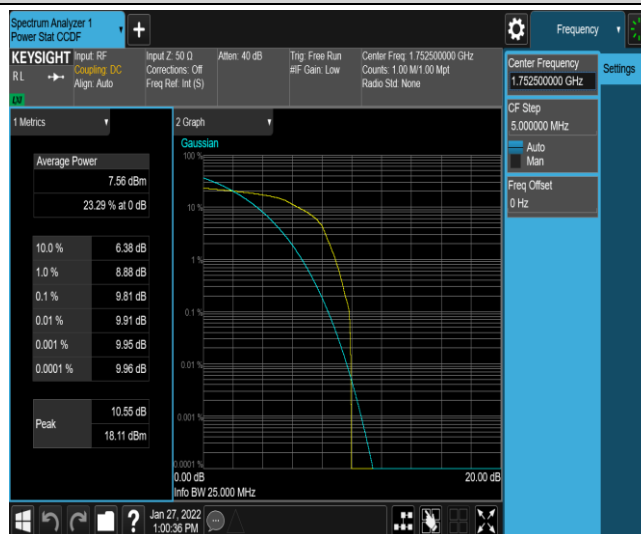
Band4-5MHz-16QAM-20375-1-0-High-9.81-&lt;=13-PASS
