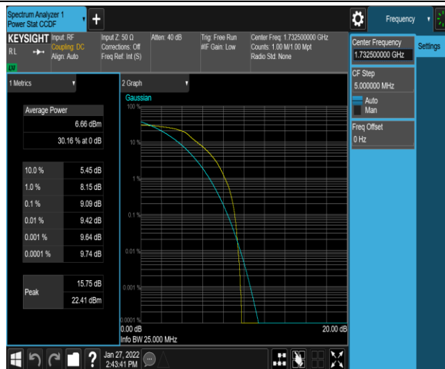
Band4-10MHz-OPSK-20175-6-0-Low-9.09-<=13-PASS
