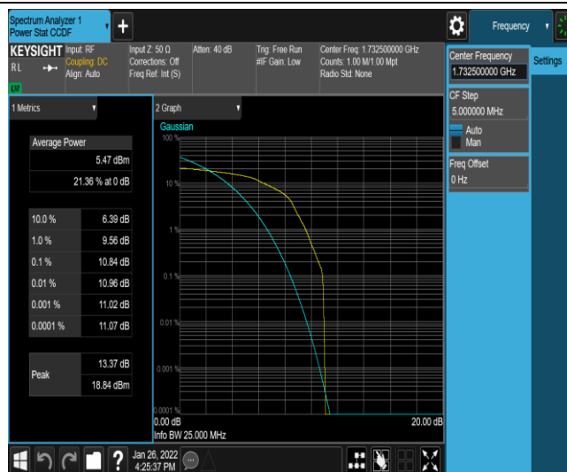
Band4-1.4MHz-16QAM-20175-1-0-Low-10.84-&lt;=13-PASS
