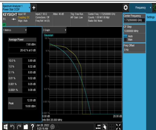
Band4-3MHz-QPSK-20175-1-0-Low-8.93-&lt;=13-PASS
