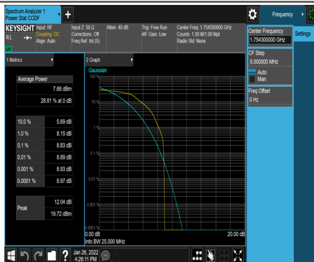
Band4-1.4MHz-QPSK-20393-1-0-High-8.83-<=13-PASS
