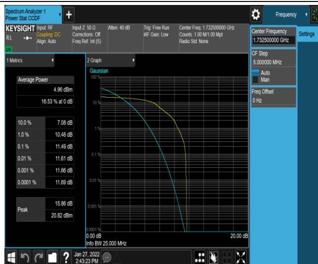
Band4-10MHz-QPSK-20175-1-0-Low-11.49-<=13-PASS
