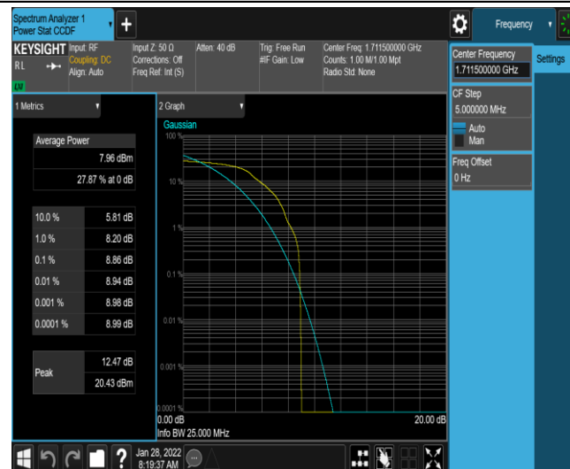
Band4-3MHz-QPSK-19965-1-0-Low-8.86-&lt;=13-PASS
