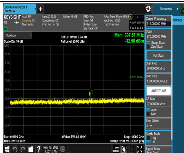
Band2-10MHz-QPSK-19150-1-0-High-30-1000--32.58-PASS
