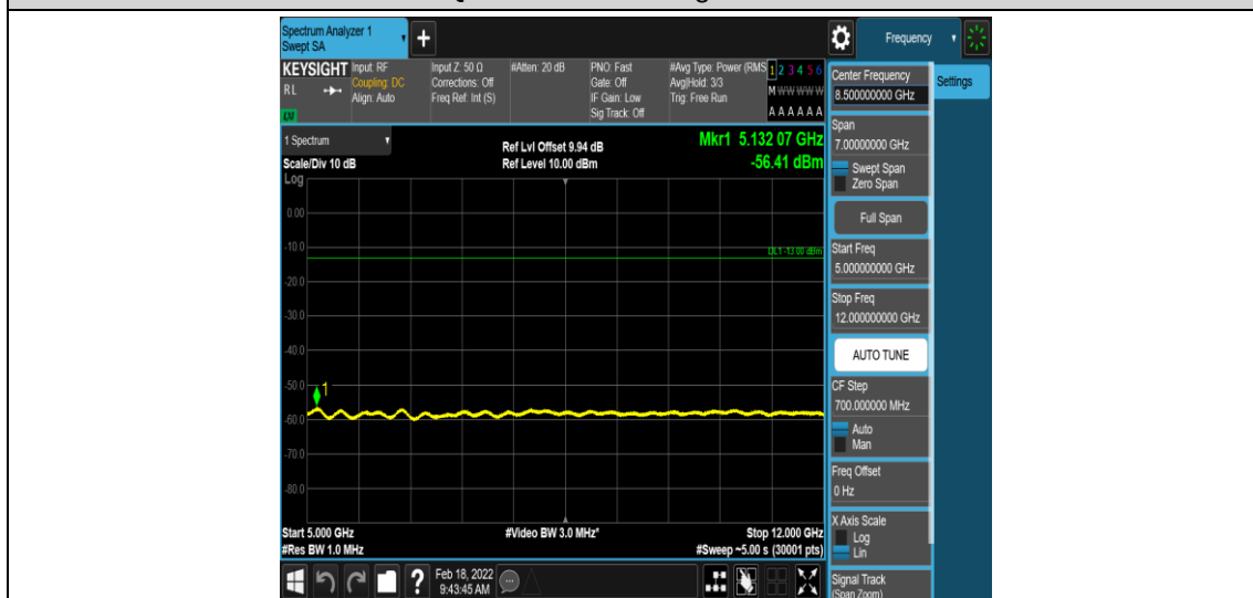
Band2-15MHz-16QAM-19125-1-0-High-5000-12000--56.41-PASS
