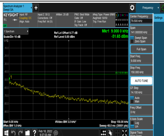
Band2-15MHz-16QAM-18675-1-0-Low-0.009-0.15--51.65-PASS
