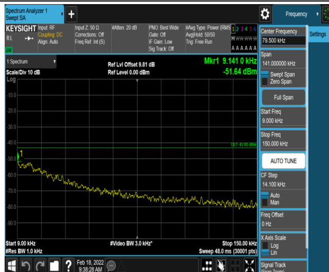
Band2-15MHz-QPSK-18900-1-0-Low-0.009-0.15--51.64-PASS
