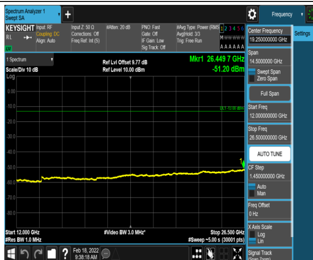
Band2-15MHz-16QAM-18675-1-0-Low-12000-26500--51.2-PASS
