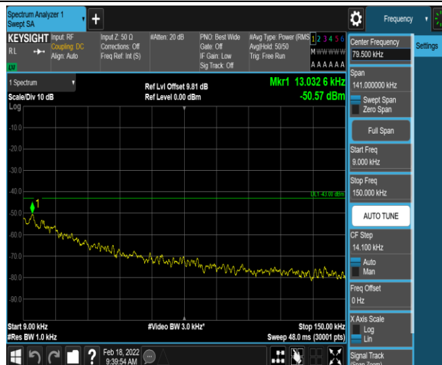
Band2-15MHz-16QAM-18900-1-0-Low-0.009-0.15--50.57-PASS
