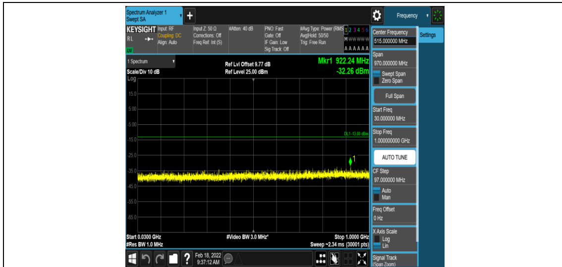
Band2-15MHz-16QAM-18675-1-0-Low-30-1000--32.26-PASS
