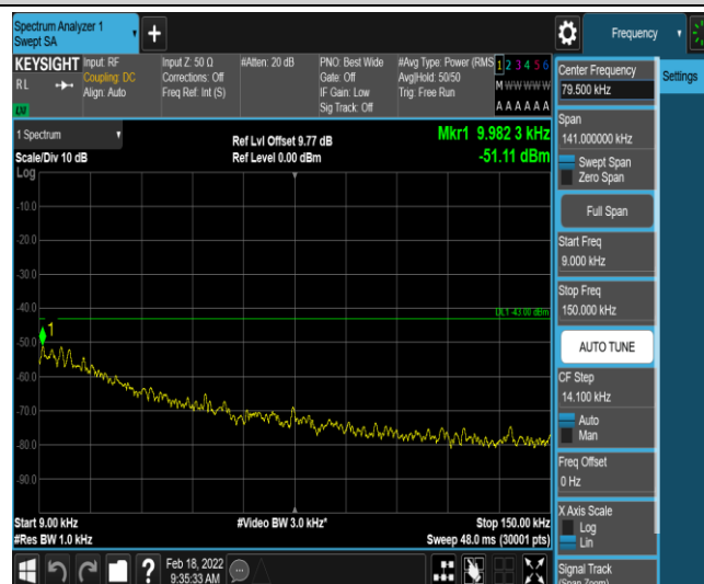
Band2-15MHz-QPSK-18675-1-0-Low-0.009-0.15--51.11-PASS
