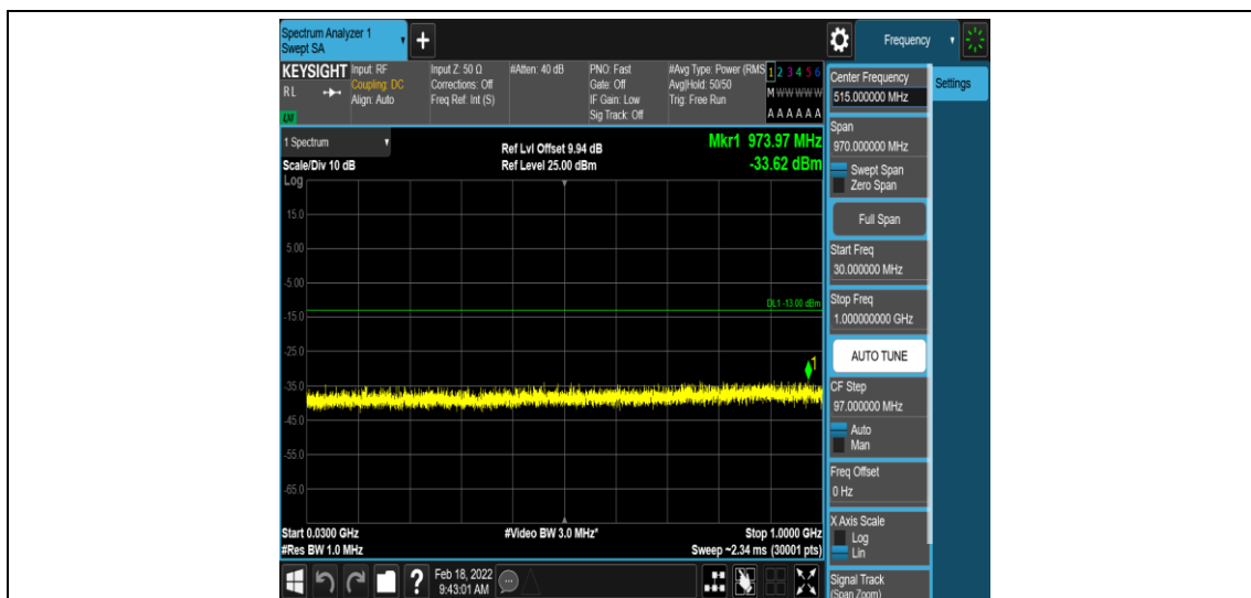
Band2-15MHz-16QAM-19125-1-0-High-30-1000--33.62-PASS
