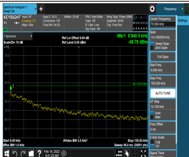
Band2-15MHz-QPSK-19125-1-0-High-0.009-0.15--48.79-PASS
