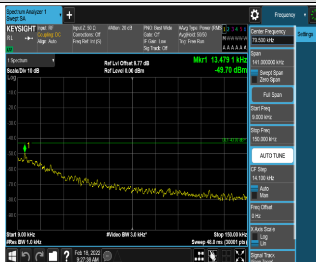
Band2-10MHz-16QAM-18650-1-0-Low-0.009-0.15--49.7-PASS
