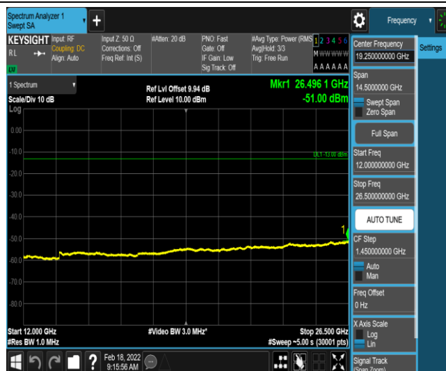
Band2-3MHz-16QAM-19185-1-0-High-12000-26500--51-PASS
