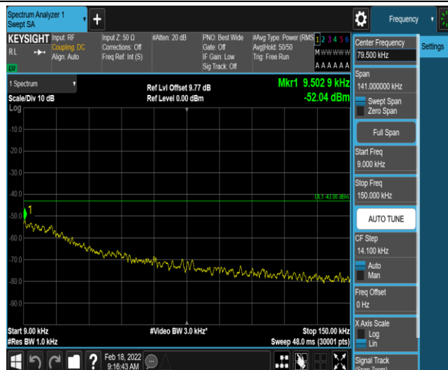
Band2-5MHz-QPSK-18625-1-0-Low-0.009-0.15--52.04-PASS
