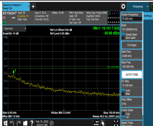
Band2-5MHz-QPSK-19175-1-0-High-0.009-0.15--50.88-PASS
