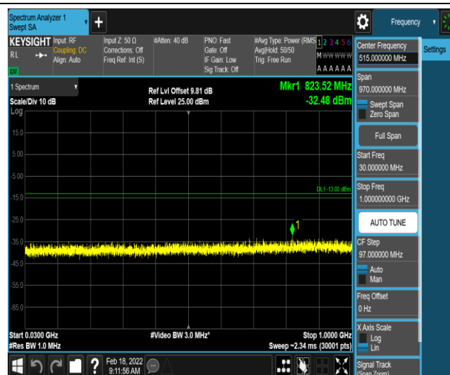
Band2-3MHz-16QAM-18900-1-0-Low-30-1000--32.48-PASS
