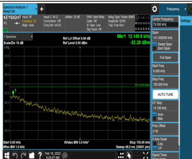
Band2-5MHz-16QAM-19175-1-0-High-0.009-0.15--52.28-PASS
