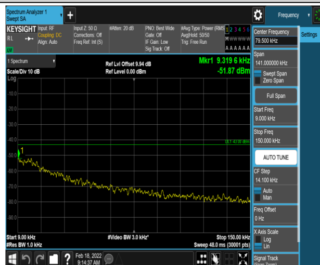
Band2-3MHz-16QAM-19185-1-0-High-0.009-0.15--51.87-PASS
