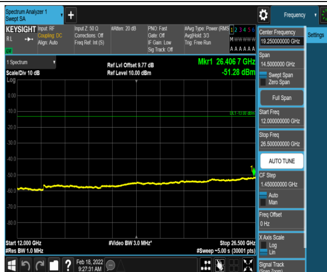
Band2-10MHz-QPSK-18650-1-0-Low-12000-26500--51.28-PASS
