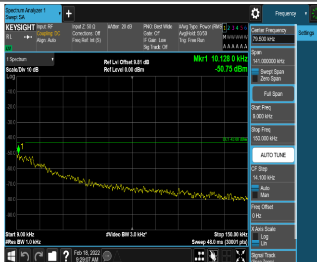
Band2-10MHz-QPSK-18900-1-0-Low-0.009-0.15--50.75-PASS
