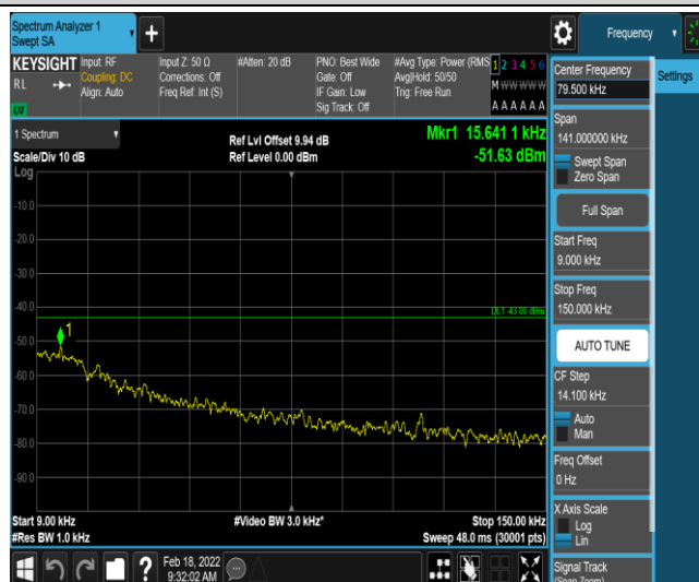
Band2-10MHz-QPSK-19150-1-0-High-0.009-0.15--51.63-PASS
