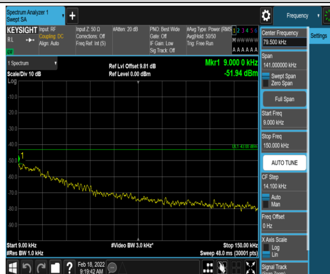
Band2-5MHz-QPSK-18900-1-0-Low-0.009-0.15--51.94-PASS
