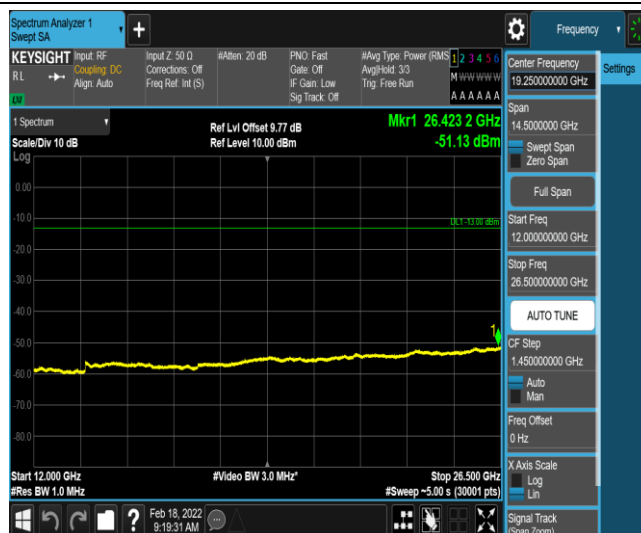
Band2-5MHz-16QAM-18625-1-0-Low-12000-26500--51.13-PASS
