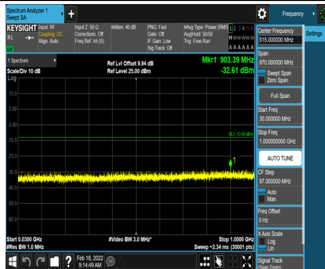
Band2-3MHz-16QAM-19185-1-0-High-30-1000--32.61-PASS
