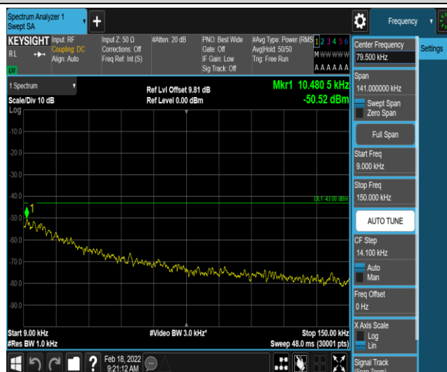
Band2-5MHz-16QAM-18900-1-0-Low-0.009-0.15--50.52-PASS
