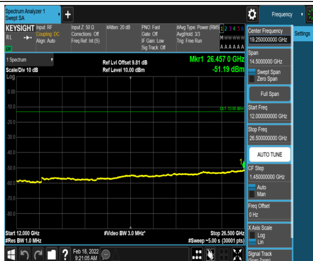
Band2-5MHz-QPSK-18900-1-0-Low-12000-26500--51.19-PASS
