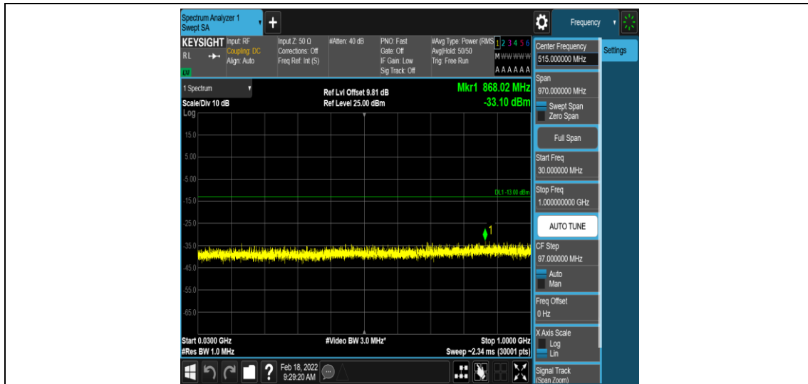
Band2-10MHz-QPSK-18900-1-0-Low-30-1000--33.1-PASS
