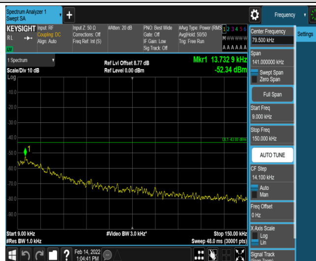
Band2-1.4MHz-16QAM-18607-1-0-Low-0.009-0.15--52.34-PASS
