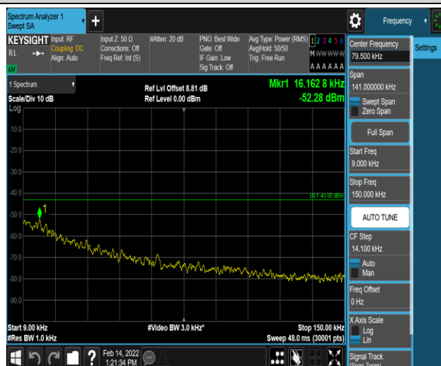
Band2-1.4MHz-QPSK-18900-1-0-Low-0.009-0.15--52.28-PASS
