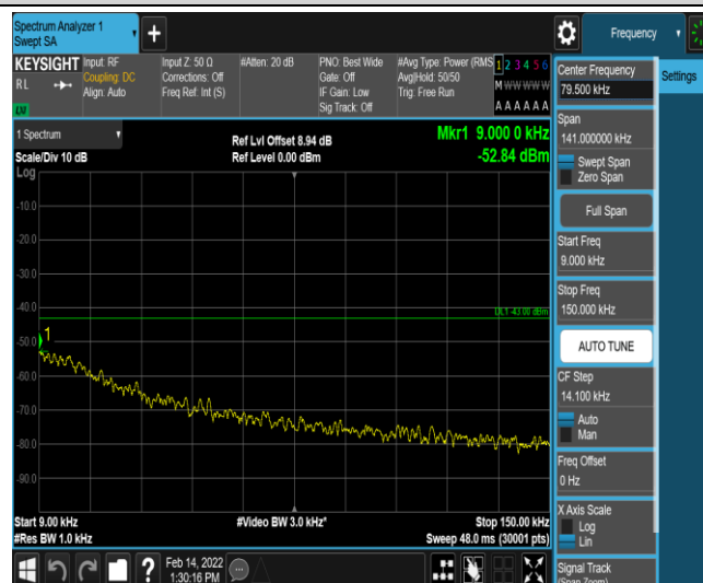
Band2-1.4MHz-QPSK-19193-6-0-Low-0.009-0.15--52.84-PASS
