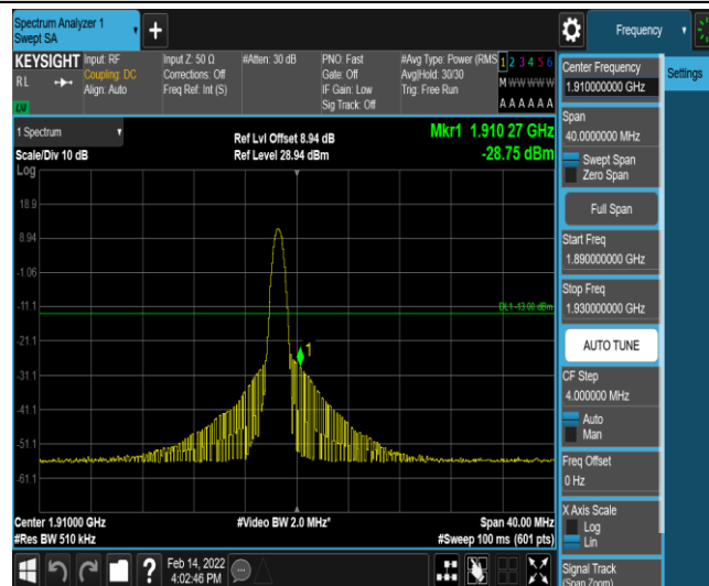
Band2-20MHz-QPSK-19100-1-5-High--28.75-PASS
