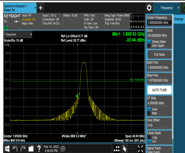
Band2-20MHz-QPSK-18700-6-0-Low--32.44-PASS
