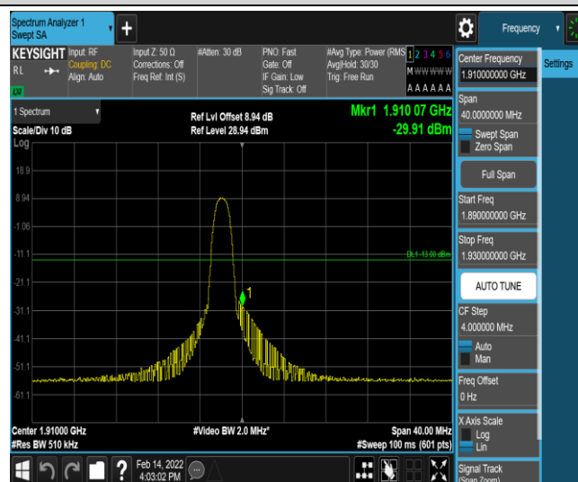
Band2-20MHz-QPSK-19100-6-0-High--29.91-PASS
