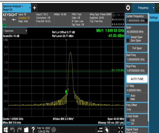
Band2-20MHz-16QAM-18700-1-0-Low--41.93-PASS
