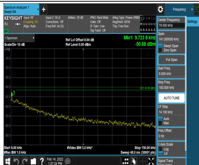
Band2-1.4MHz-QPSK-19193-1-5-Low-0.009-0.15--50.68-PASS
