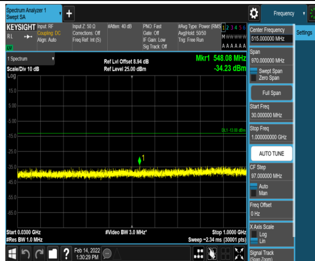
Band2-1.4MHz-QPSK-19193-6-0-Low-30-1000--34.23-PASS
