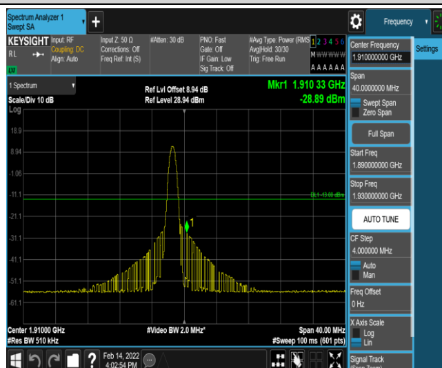
Band2-20MHz-16QAM-19100-1-5-High--28.89-PASS
