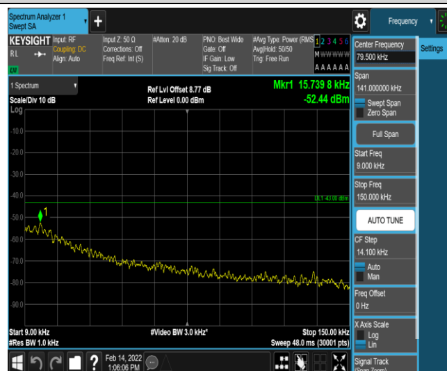
Band2-1.4MHz-QPSK-18607-6-0-Low-0.009-0.15--52.44-PASS
