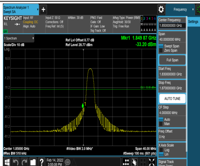
Band2-20MHz-16QAM-18700-6-0-Low--33.20-PASS
