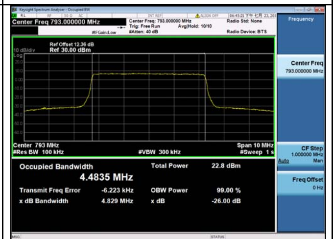
LTE band 14 - Middle CH 16QAM-5
