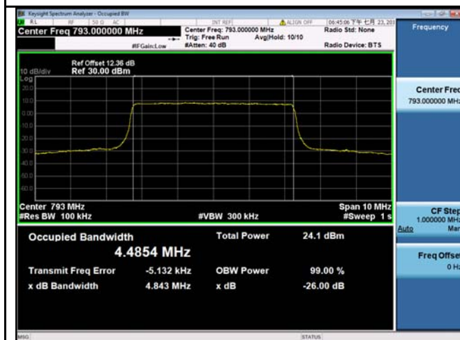
LTE band 14 - Middle CH QPSK-5
