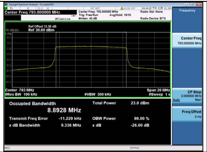
LTE band 14 - Middle CH 16QAM-10
