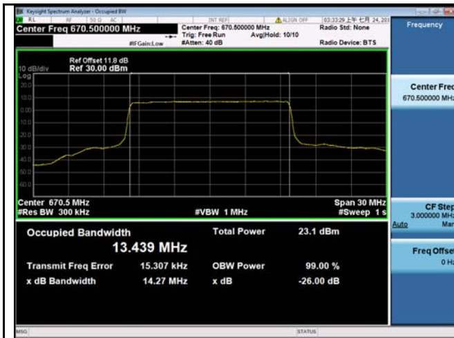
LTE band 71 - Low CH QPSK-15
