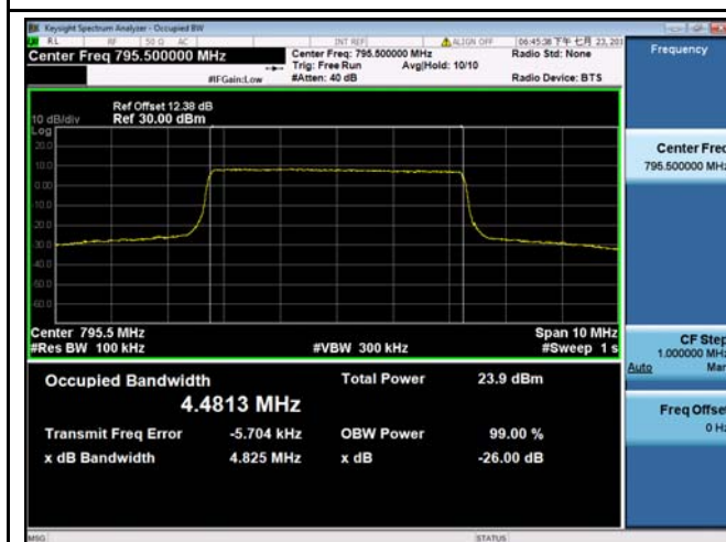
LTE band 14 - Middle CH QPSK-5
