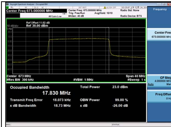
LTE band 71 - Low CH QPSK-20
