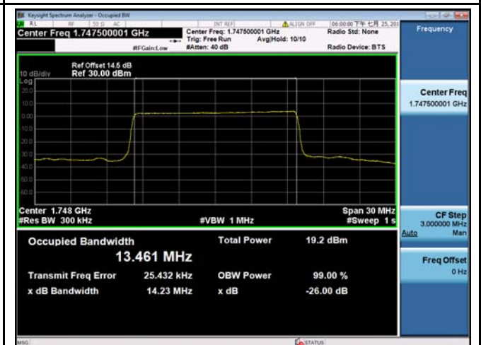
LTE band 4 - High CH 16QAM-15
